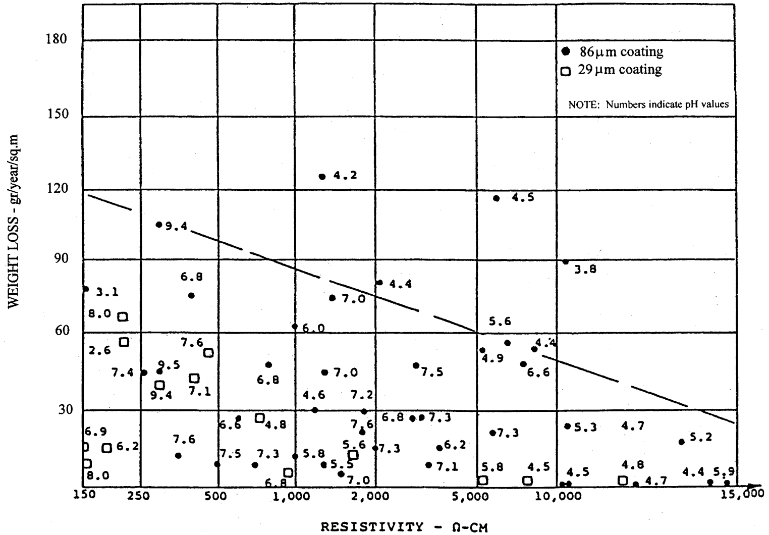
Figure 1. Metal loss as a function of resistivity (galvanized steel).
