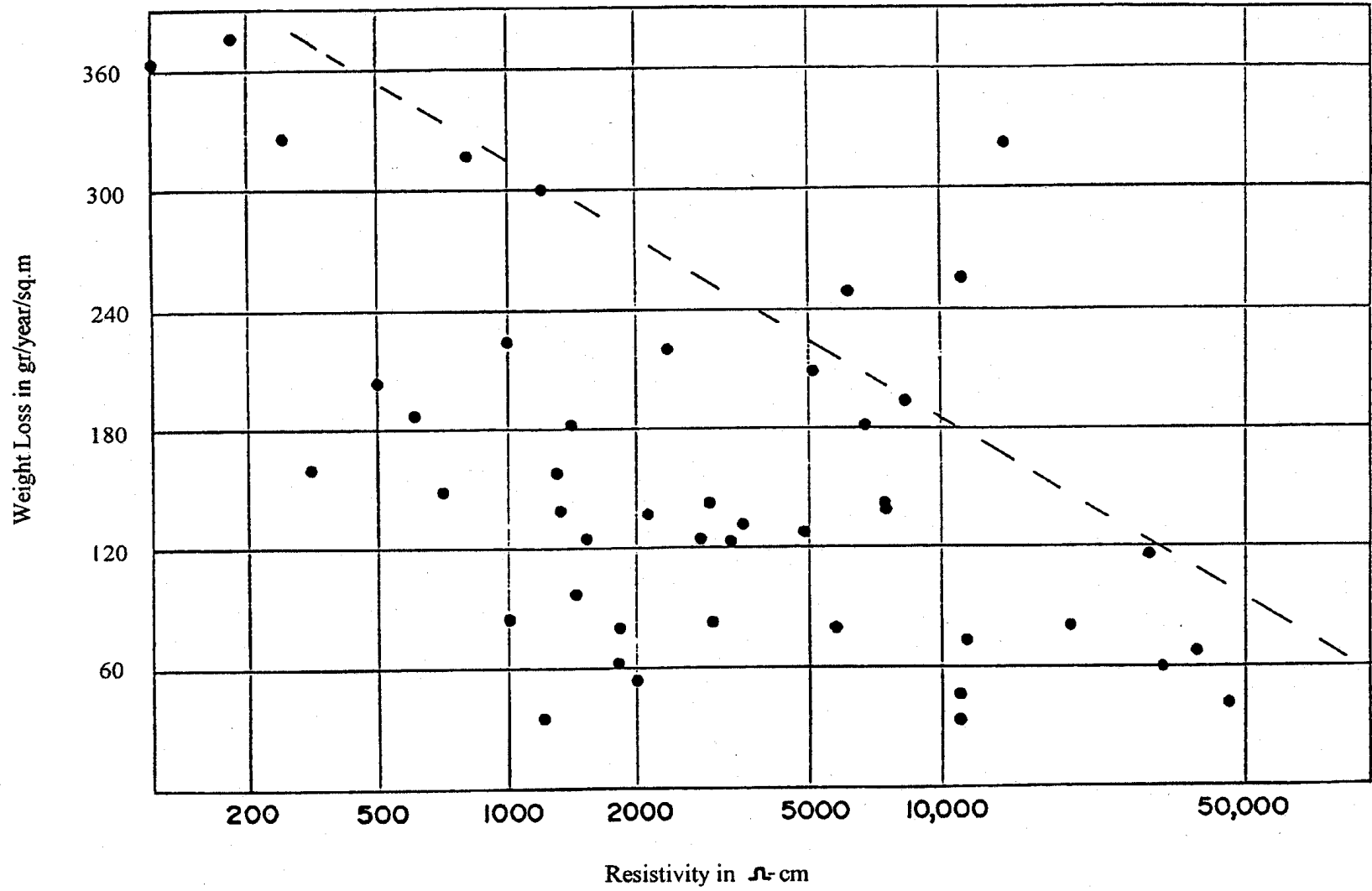
Figure 2. Metal loss as a function of resistivity (carbon steel).
