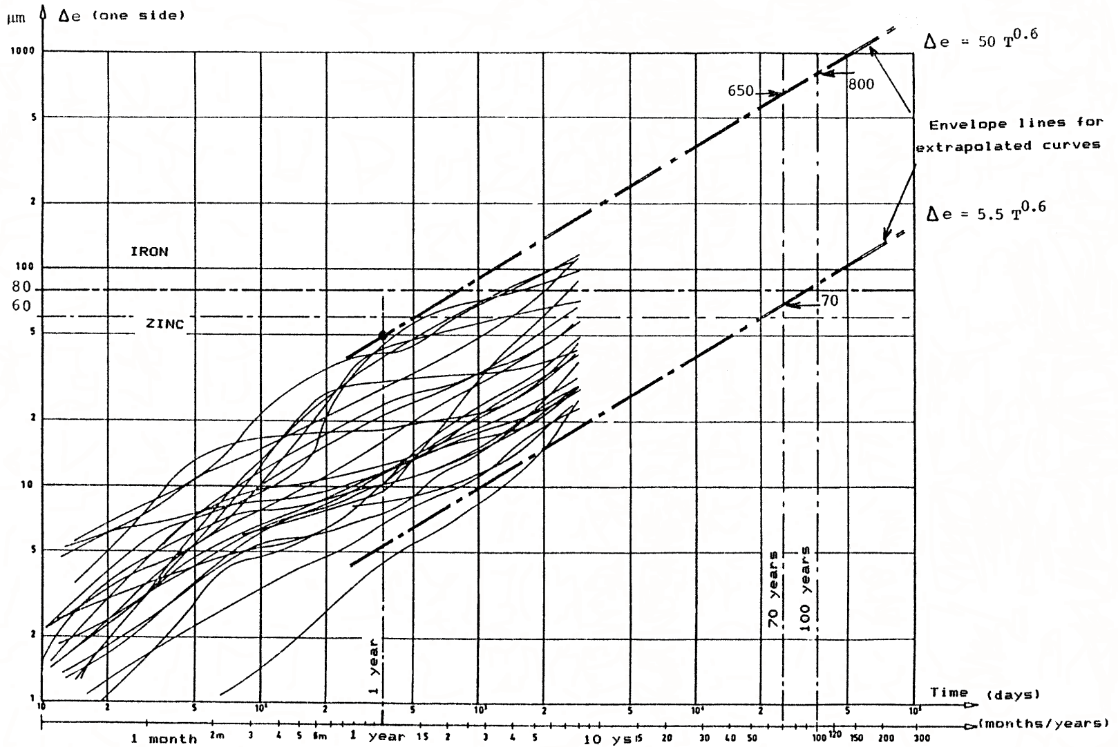
Figure 5. Summary of electrochemical cell test data at 50% and 100% saturation.
