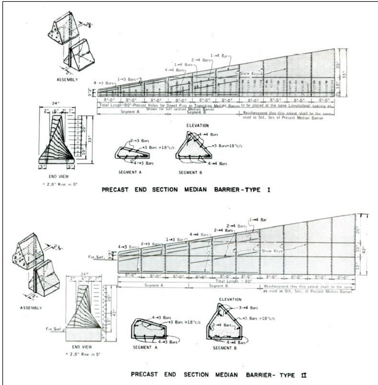
Figure 14. Oklahoma Sloped End Treatment Drawing [5]
