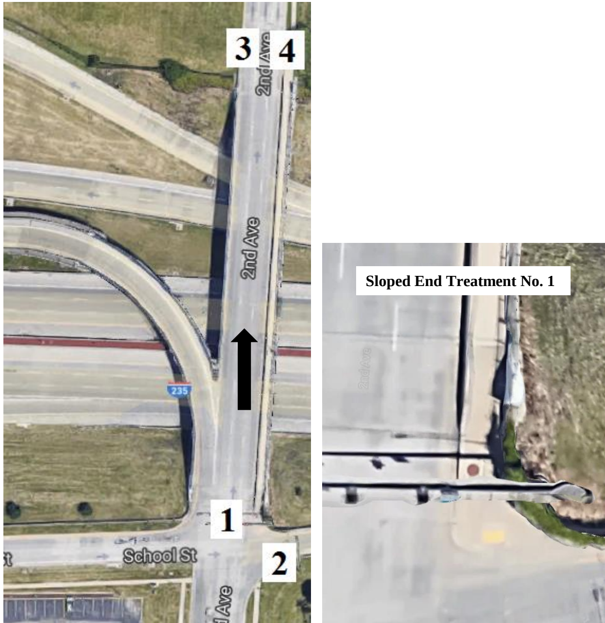
Figure 151. Bridge No. 7708.3O235 with Sloped End Treatments Labeled [1]
