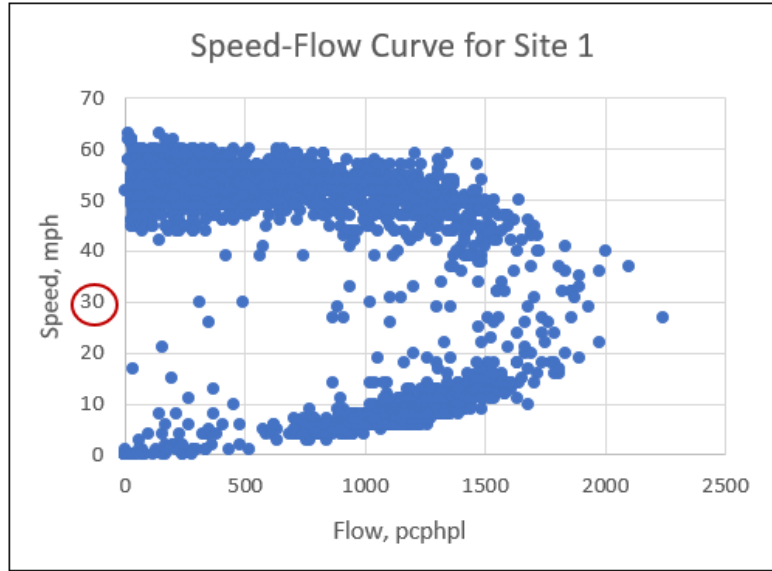
Figure 13. Speed curve for site 1
