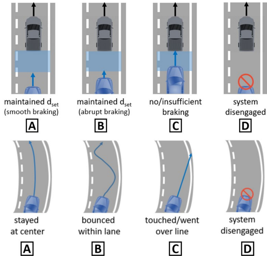
Figure 2. Example codes for the automated longitudinal control features' responses to a slow lead (top) and the lateral control features' responses on curves (bottom) used for classifying participants' qualitative comments.
