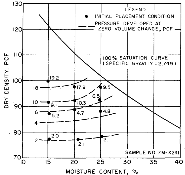
Figure 15. Total uplift pressure caused by wetting for various placement conditions (from Reference 95)
