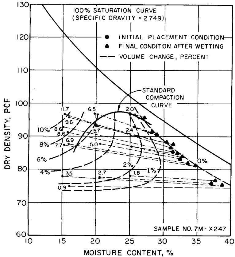
Figure 14. Percentage of expansion for various placement conditions under a 1 psi surcharge (from Reference 95)
