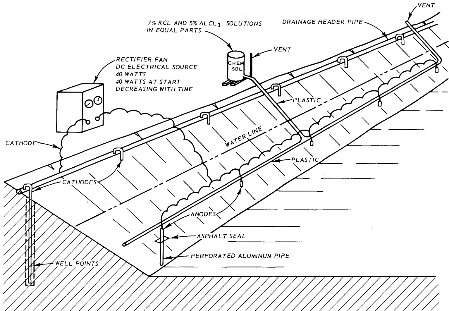
Figure 17. Electro-chemical stabilization experiment, Friant-Kern Canal, California (from Reference 28)
