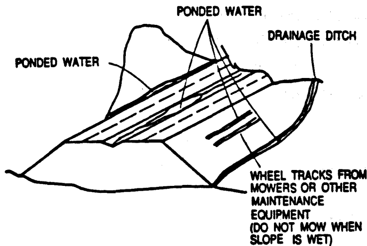
Areas of the slope where water may pond
