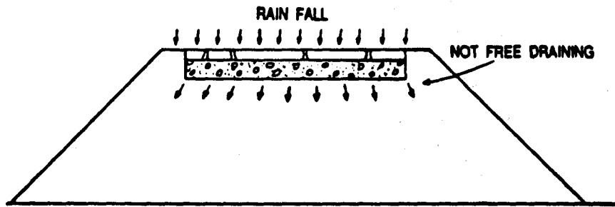
Bathtub drainage condition caused by poor drainage material
