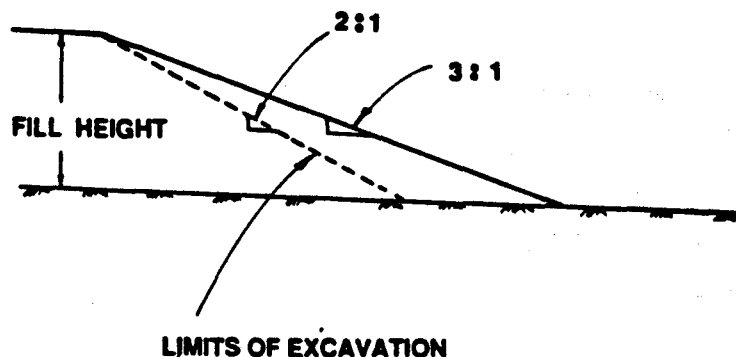
Suggested limits of excavation for various slopes
