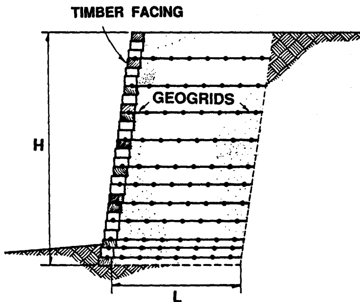
Use of timber facing to protect geotextile material
