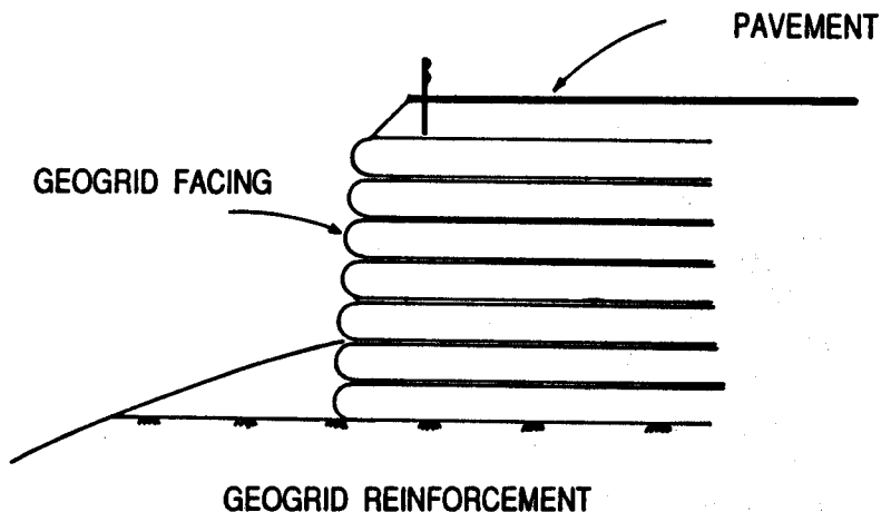
Reinforced retaining wall
