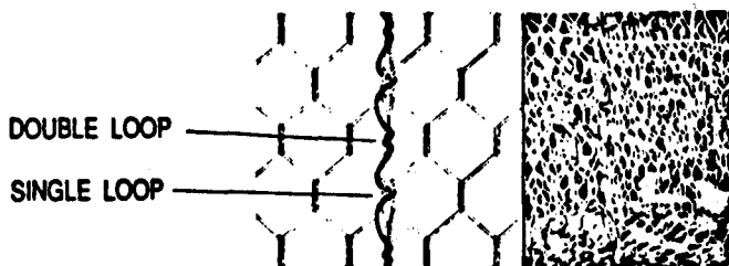
Method of looping lacing wire
