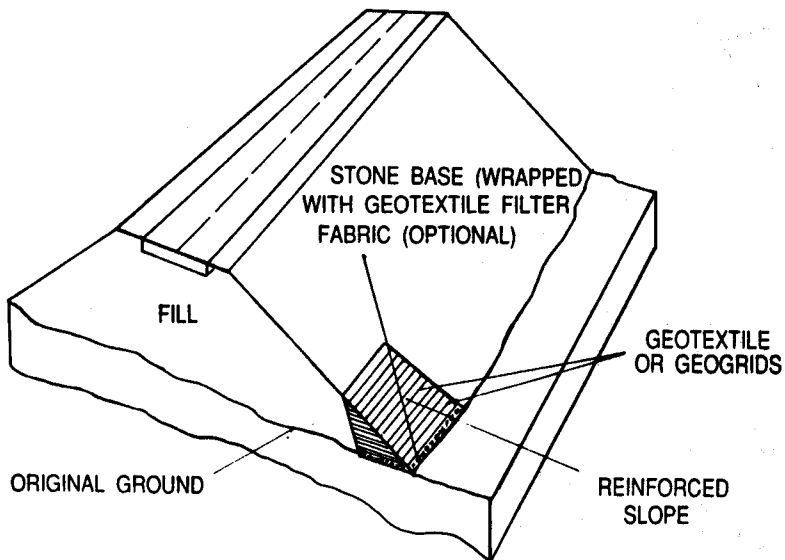
Repair of a toe slump using a reinforced slope
