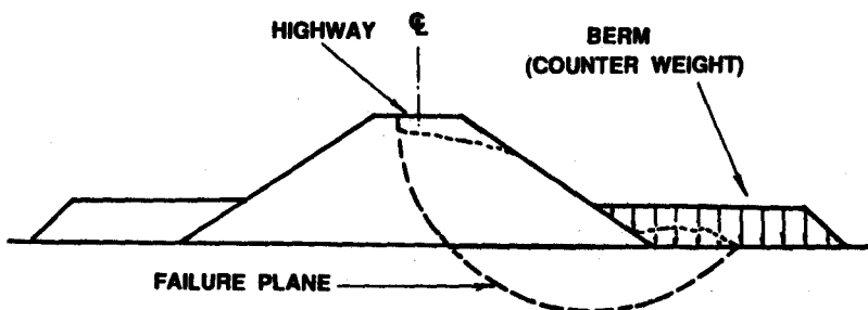
Use of earth and rock berms as a counterweight in the toe area of a failed slope
