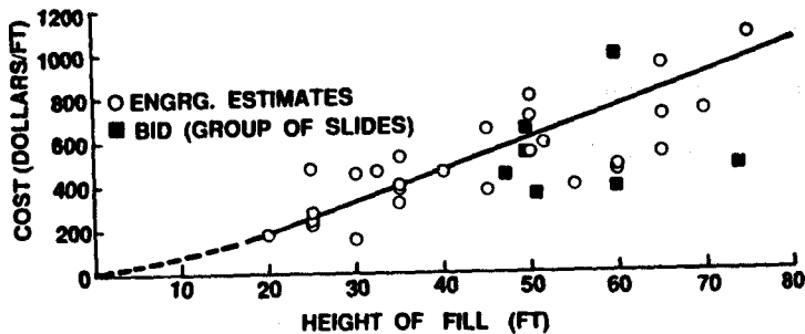
Repair cost of berm and / or flattened slope per linear foot of slope failure and height of fill ( or height of slope failure )
