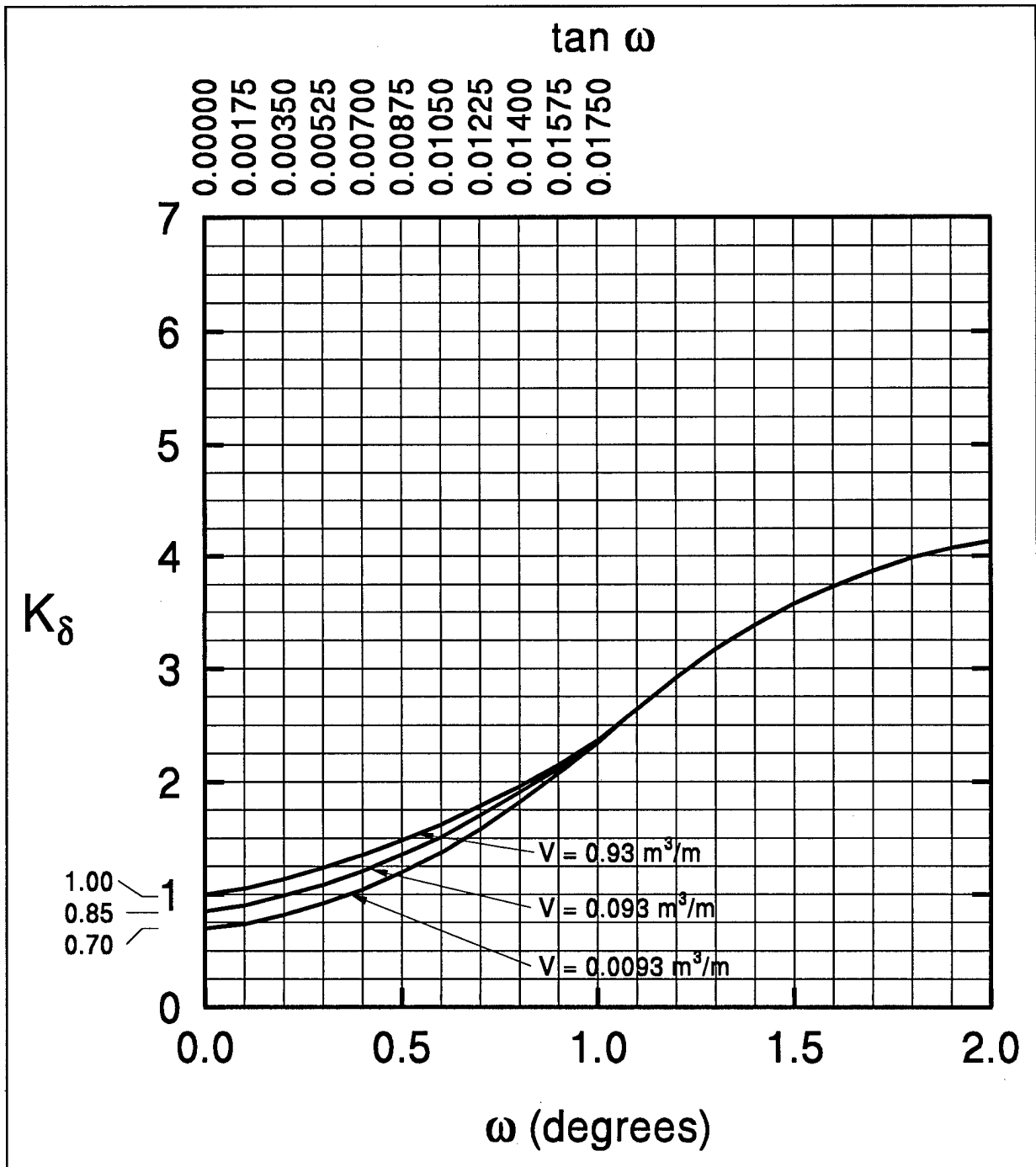
Figure 7-5. Design curves for evaluating K_\delta for piles when \phi = 25^\circ (after Norlund 1979).
