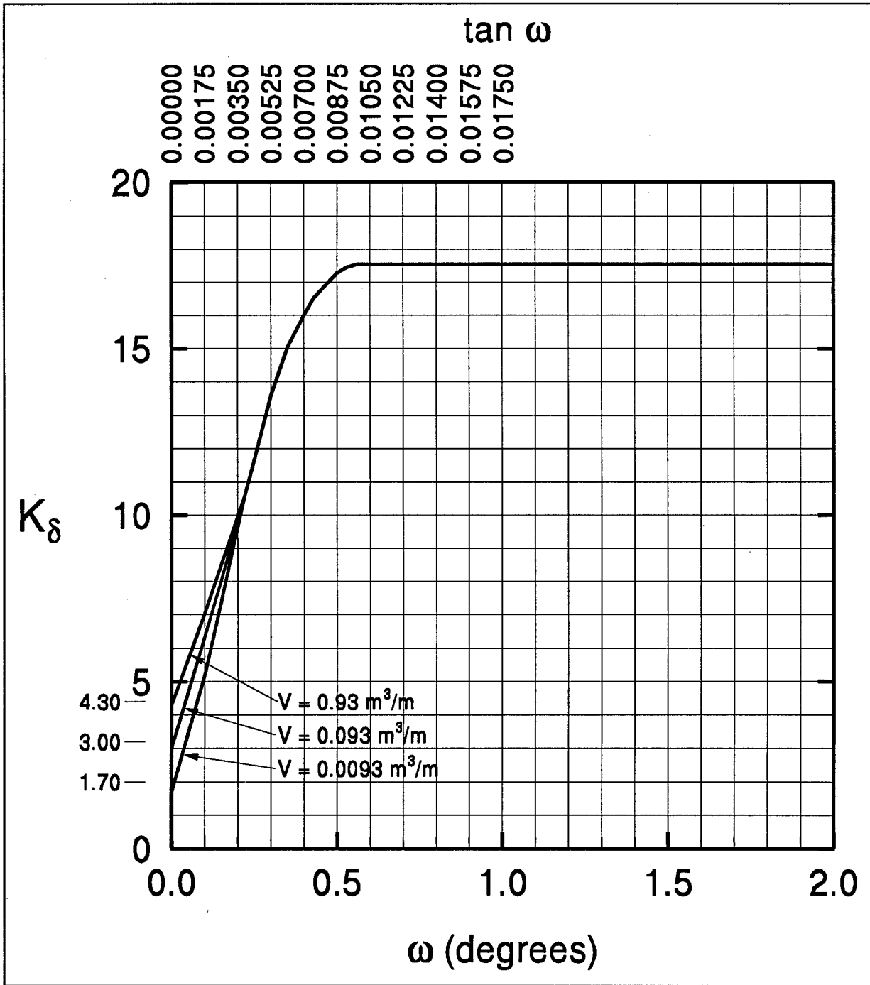
Figure 7-8. Design curves for evaluating K_\delta for piles when \phi = 40^\circ (after Norlund 1979).
