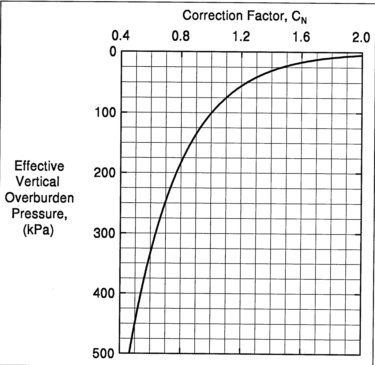
Figure 7-11. Chart for correction of N-values in sand for influence of effective overburden pressure (after Peck et. al. 1974).
