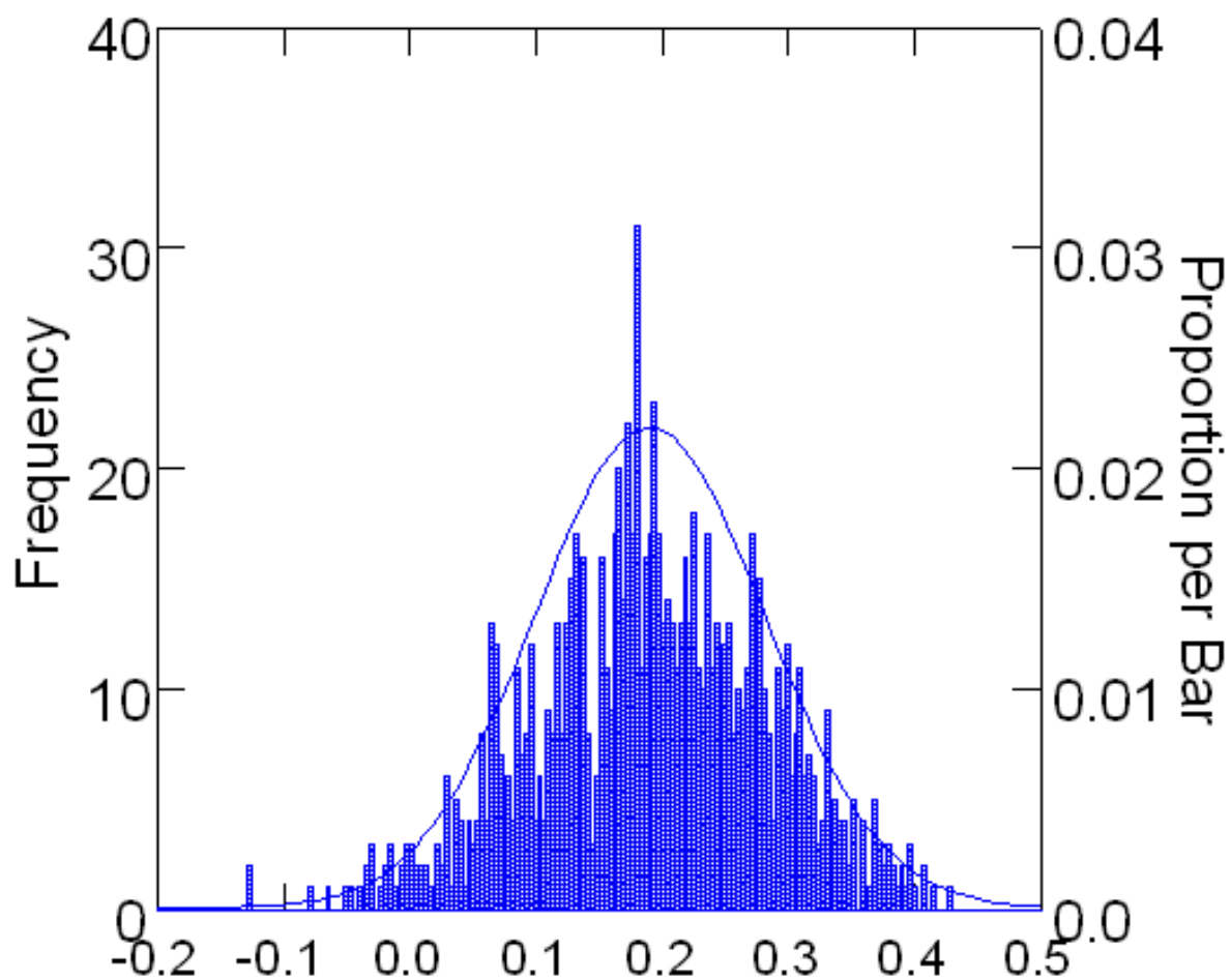
Graph A-6: Distribution of TMC-NLCOMP correlations uncorrected for range restriction for B = 1,000 bootstrap samples of n = 150
