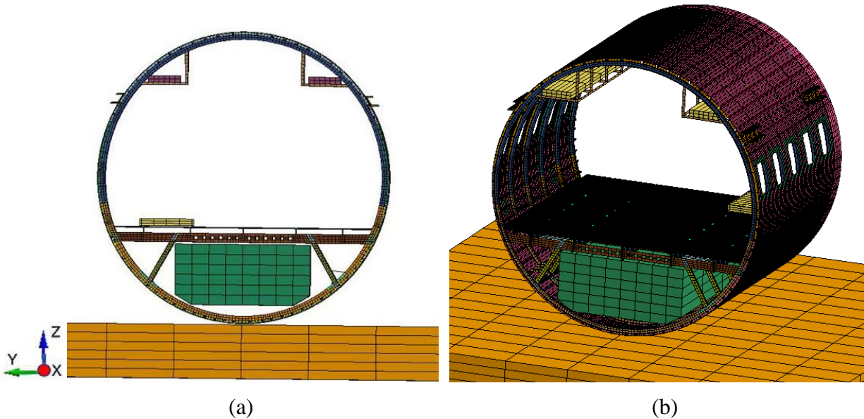
Figure 14. Views of the FEM of the F-28 fuselage section: (a) rear view of model and (b) three-quarter front view of model
