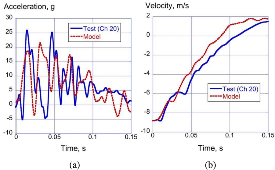
Figure 34. Vertical acceleration and velocity comparisons at the starboard window at FS 6805: (a) acceleration responses and (b) velocity responses
