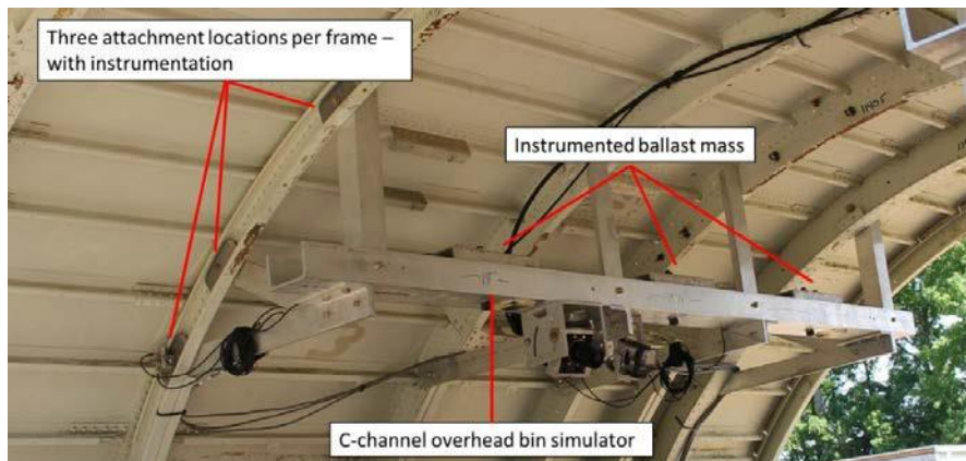
Figure 7. Hat rack simulators with ballast
