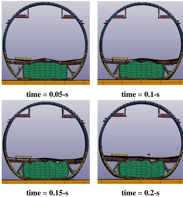
Figure 38. Model deformation sequence
