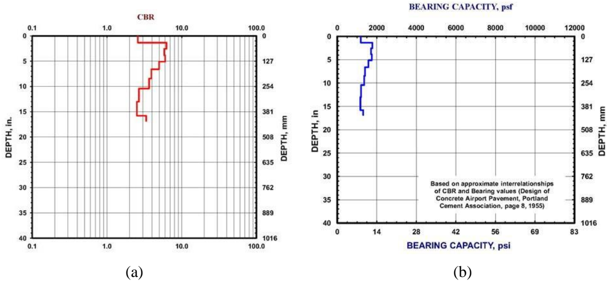
Figure 12. CBR and bearing capacity data recorded following the F-28 forward section drop test: (a) CBR plot and (b) bearing capacity plot
