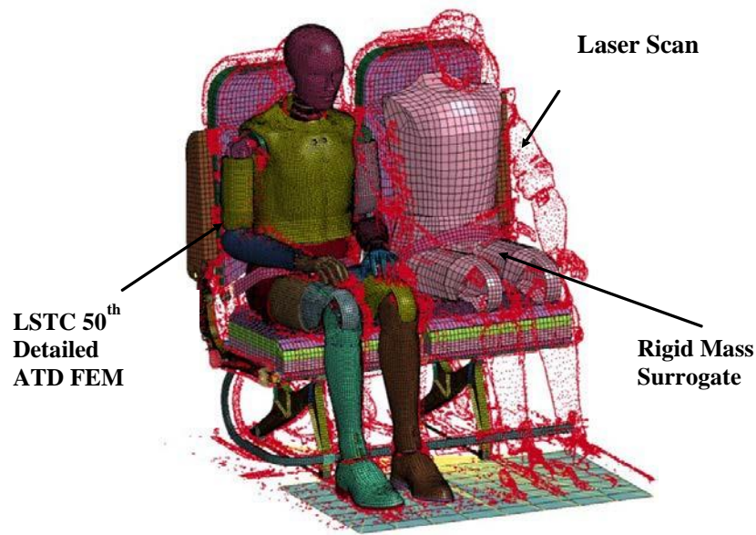
Figure 25. Combined LSTC-detailed FEM, rigid torso model, and double-seat model with laser-scan overlay
