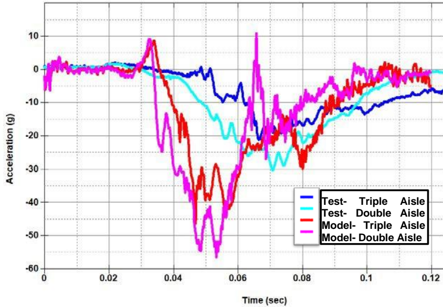
Figure 42. Pelvic z-acceleration – F-28 forward section model with seat and occupant models
