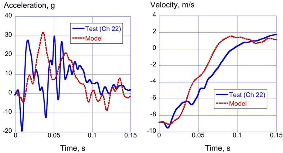
Figure 33. Vertical acceleration and velocity comparisons at the starboard aisle at FS 6805: (a) acceleration responses and (b) velocity responses
