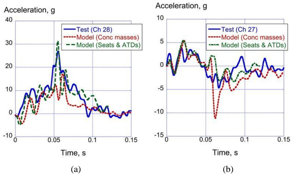
Figure 63. Plots of vertical and forward acceleration for the starboard aisle location at FS 10305: (a) vertical acceleration and (b) forward acceleration
