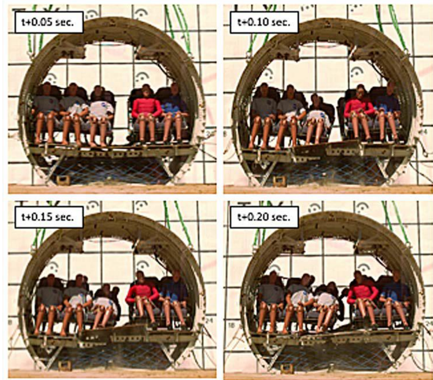
Figure 37. Impact sequence of the test
