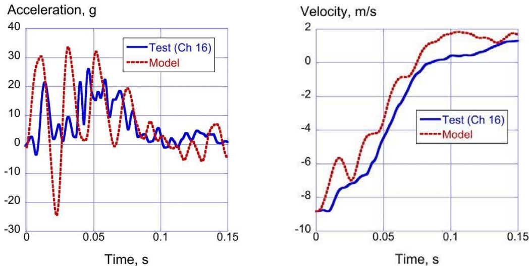
Figure 31. Vertical acceleration and velocity comparisons at the port window at FS 6805: (a) acceleration responses and (b) velocity responses
