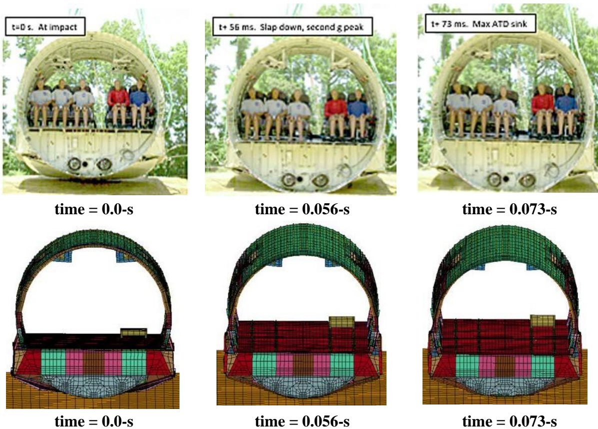
Figure 54. Test-analysis impact sequence (front view)
