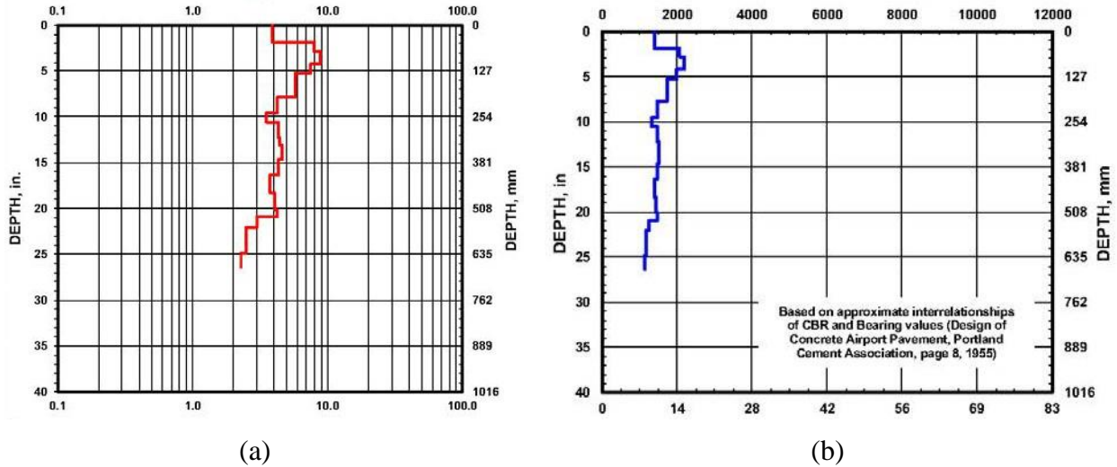
Figure 13. CBR and bearing capacity data recorded following the F-28 wing-box drop test: (a) CBR plot and (b) bearing capacity plot
