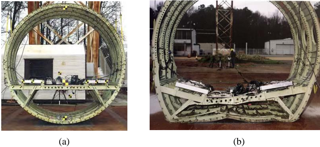
Figure 2. Pre- and post-test photographs of the 2001 vertical drop test of an F-28 fuselage section: (a) pre-test photograph and (b) post-test photograph
