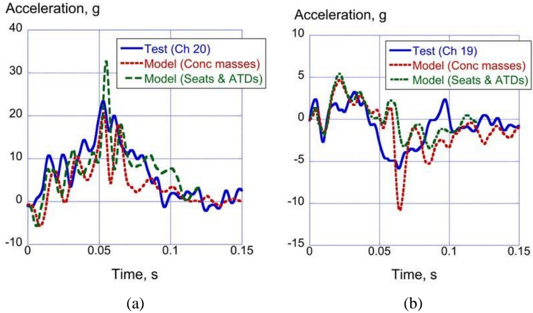
Figure 62. Plots of vertical and forward acceleration for the port aisle location at FS 10305: (a) vertical acceleration and (b) forward acceleration
