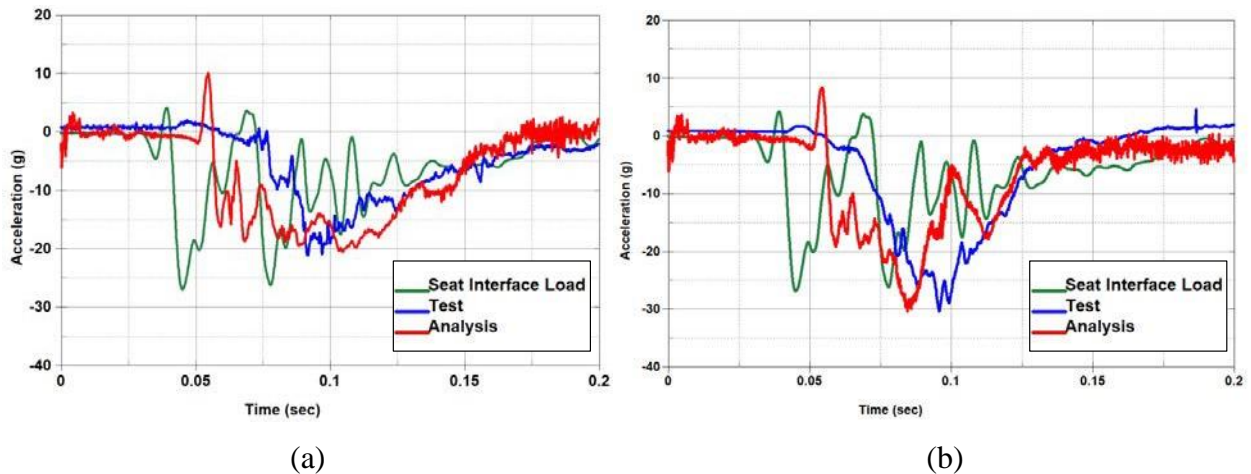
Figure 27. Pelvic z-acceleration response – LSTC-detailed FEM model of the ATD and seat: (a) Pelvic z-accel. of the triple seat ATD and (b) Pelvic z-accel. for the double seat ATD
