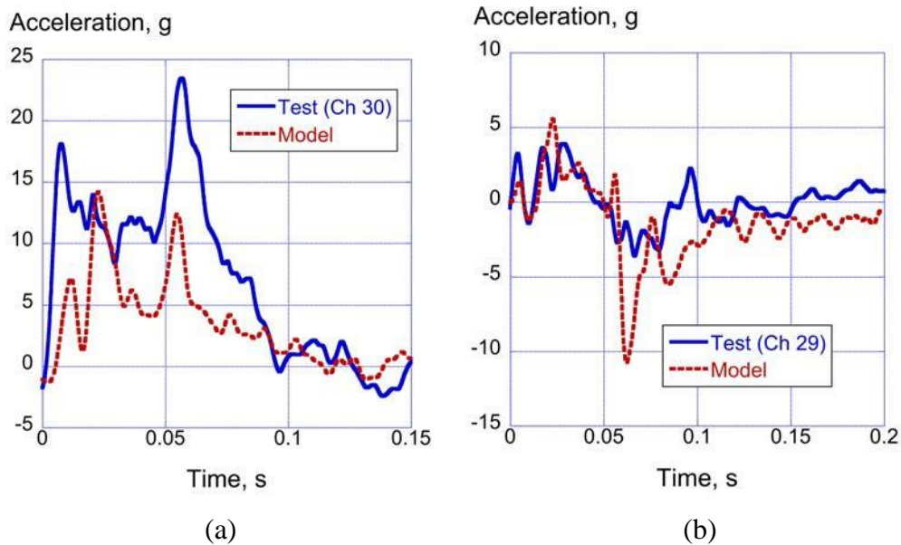
Figure 50. Vertical acceleration and velocity comparisons at the starboard window at FS 10790: (a) vertical acceleration responses and (b) forward acceleration responses
