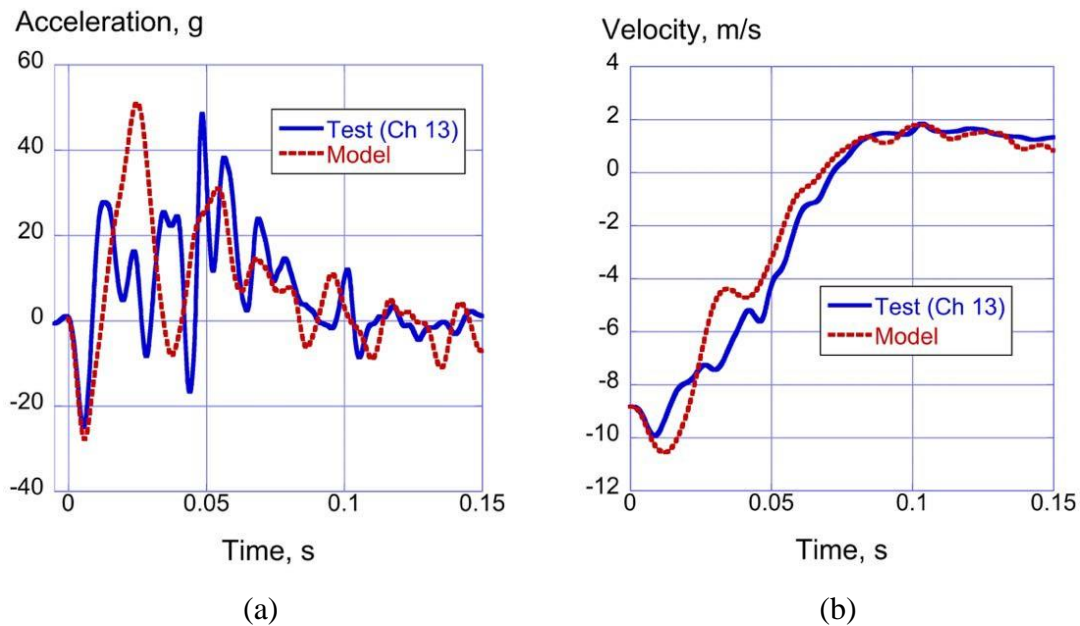
Figure 29. Vertical acceleration and velocity comparisons at the port aisle at FS 5805: (a) acceleration responses and (b) velocity responses
