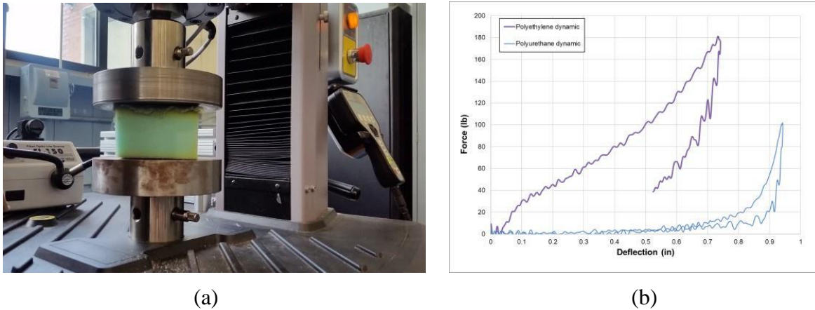
Figure 23. Foam-dynamic compression tests (a) polyurethane-foam compression test and (b) force/deflection response
