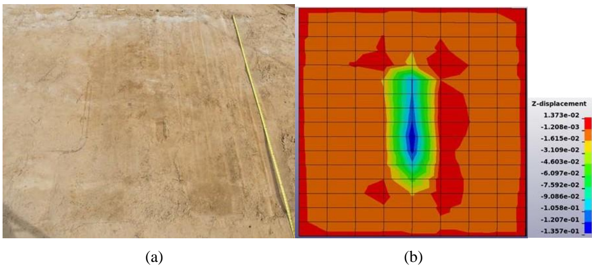
Figure 39. Crater in soil created by the F-28 forward section drop test and model deformation: (a) photograph of crater and (b) fringe plot of z-displacement of soil
