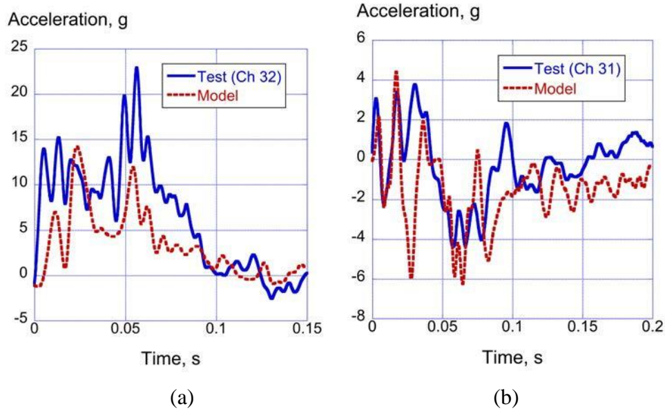
Figure 49. Vertical and forward acceleration comparisons at the starboard aisle at FS 10790: (a) vertical acceleration responses and (b) forward acceleration responses
