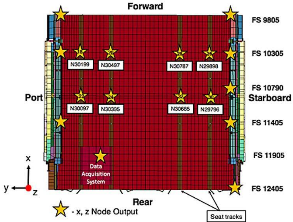
Figure 17. Depiction of the model floor layout showing test channels and nodal output locations
