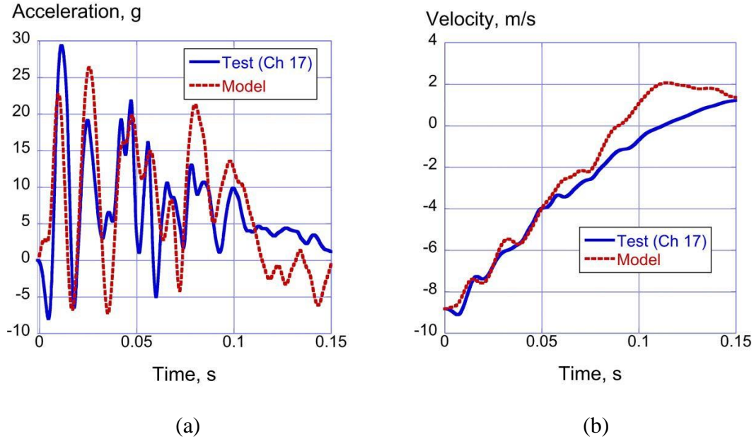
Figure 30. Vertical acceleration and velocity comparisons at the starboard window at FS 5805: (a) acceleration responses and (b) velocity responses
