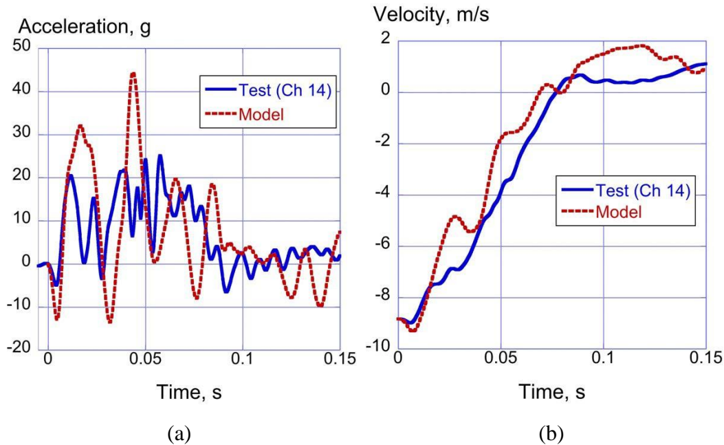
Figure 28. Vertical acceleration and velocity comparisons at the port window at FS 5805: (a) acceleration responses and (b) velocity responses
