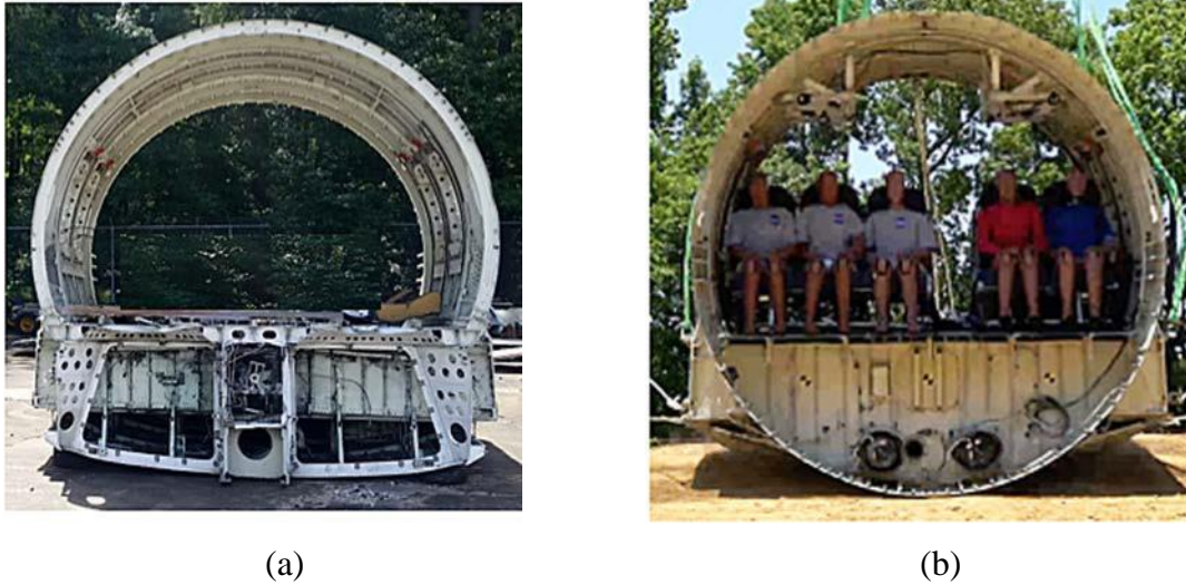
Figure 6. F-28 wing-box section photographs: (a) unloaded F-28 fuselage section and (b) fully loaded F-28 wing-box section
