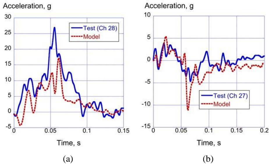
Figure 45. Vertical and forward acceleration comparisons at the starboard aisle at FS 10305: (a) vertical acceleration responses and (b) forward acceleration responses
