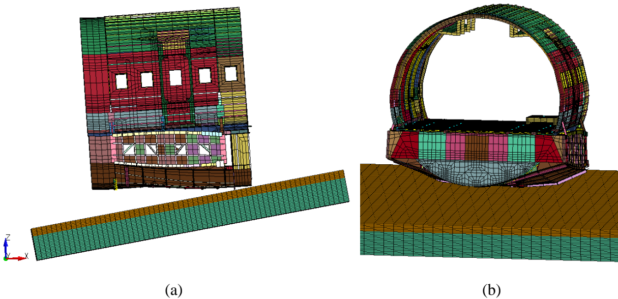
Figure 16. Two views of the FEM of the F-28 wing-box section: (a) side view and (b) three-quarter view
