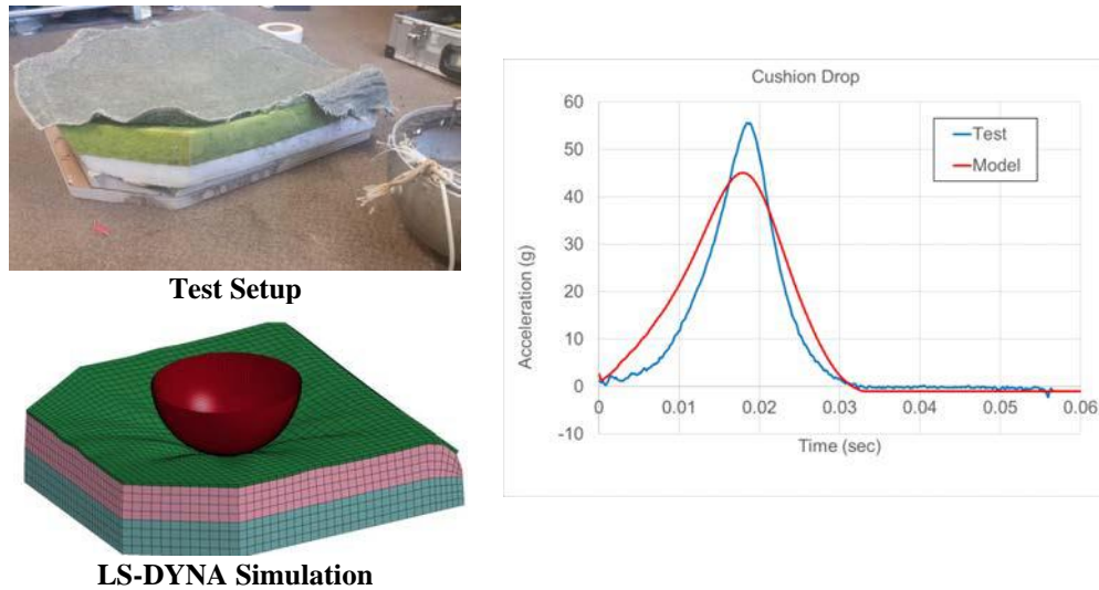
Figure 24. Seat cushion drop test and model calibration
