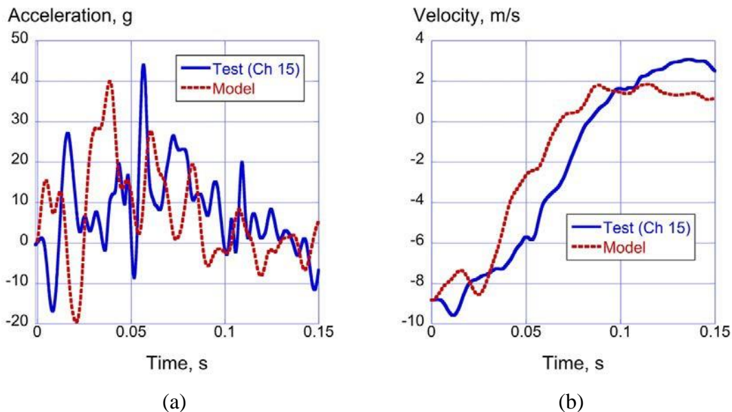
Figure 32. Vertical acceleration and velocity comparisons at the port aisle at FS 6805: (a) acceleration responses and (b) velocity responses
