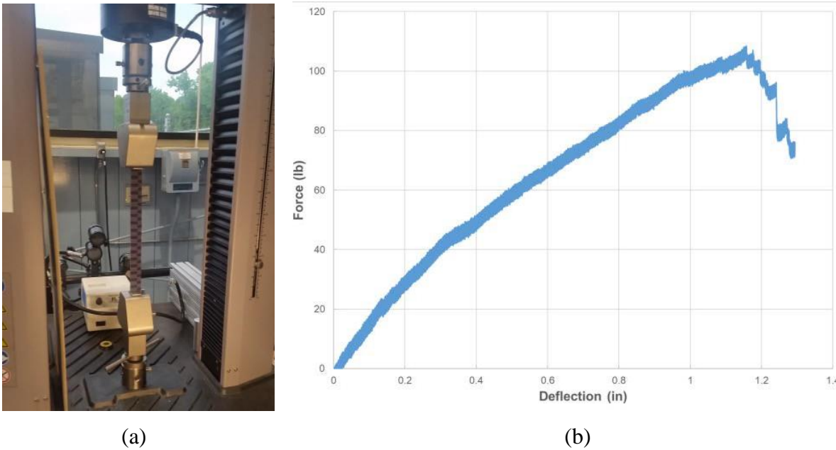
Figure 22. Fabric tensile tests: (a) tensile test of a seat cushion cover and (b) tensile test data of the seat pan fabric
