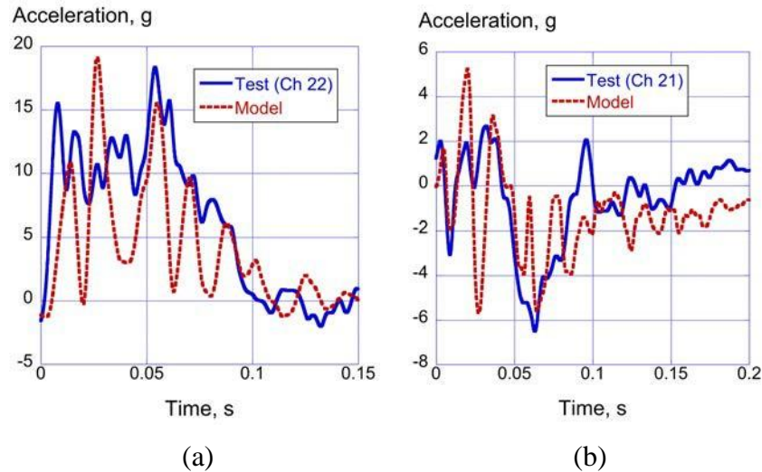
Figure 47. Vertical and forward acceleration comparisons at the port window at FS 10790: (a) vertical acceleration responses and (b) forward acceleration responses
