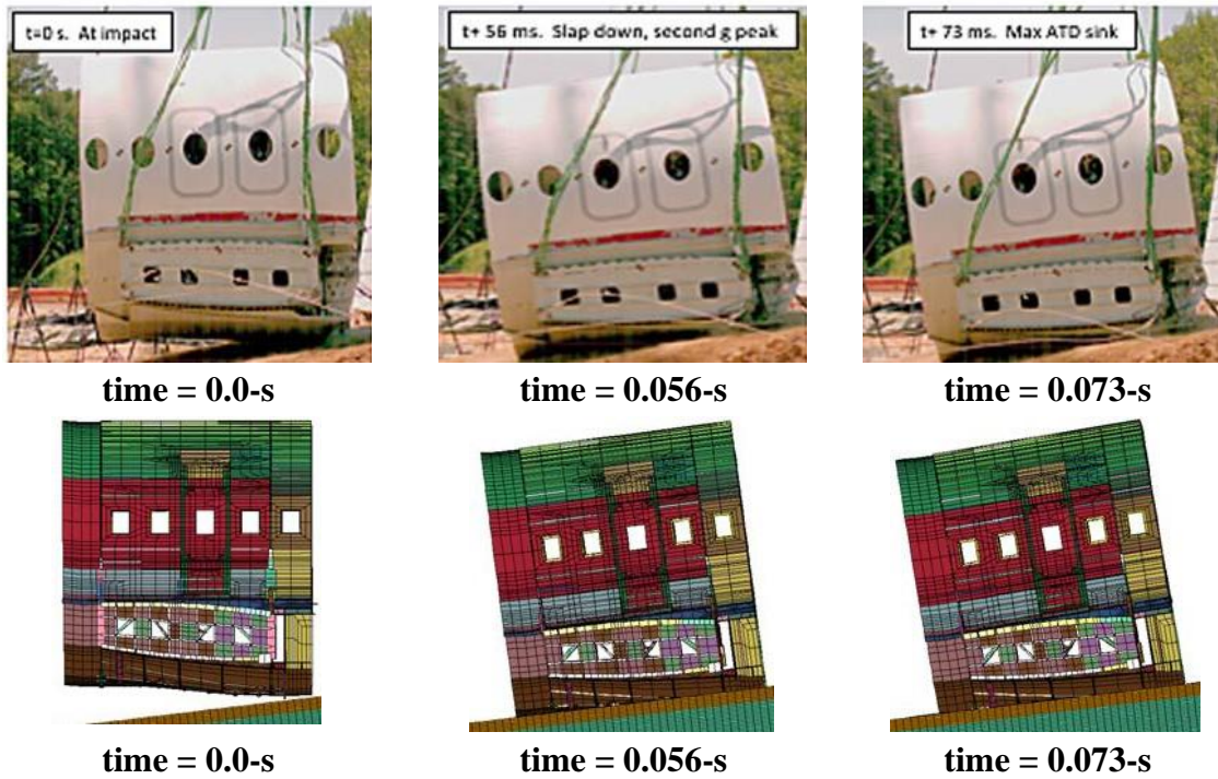
Figure 55. Test-analysis impact sequence (side view)
