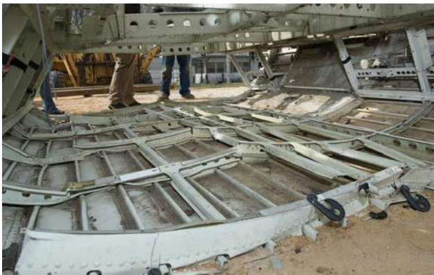
Figure 36. Post-test photographs: (a) bottom centerline failures and (b) floor failures
