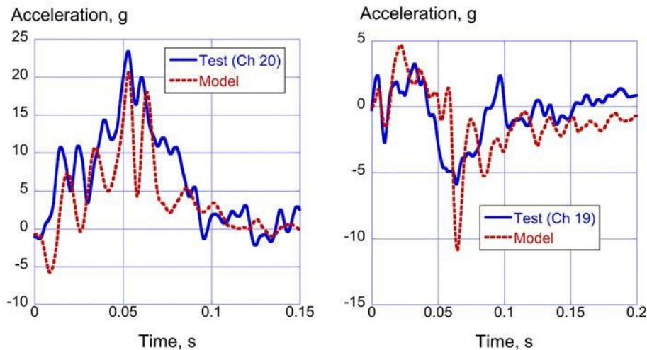
Figure 44. Vertical and forward acceleration comparisons at the port aisle at FS 10305: (a) vertical acceleration responses and (b) forward acceleration responses
