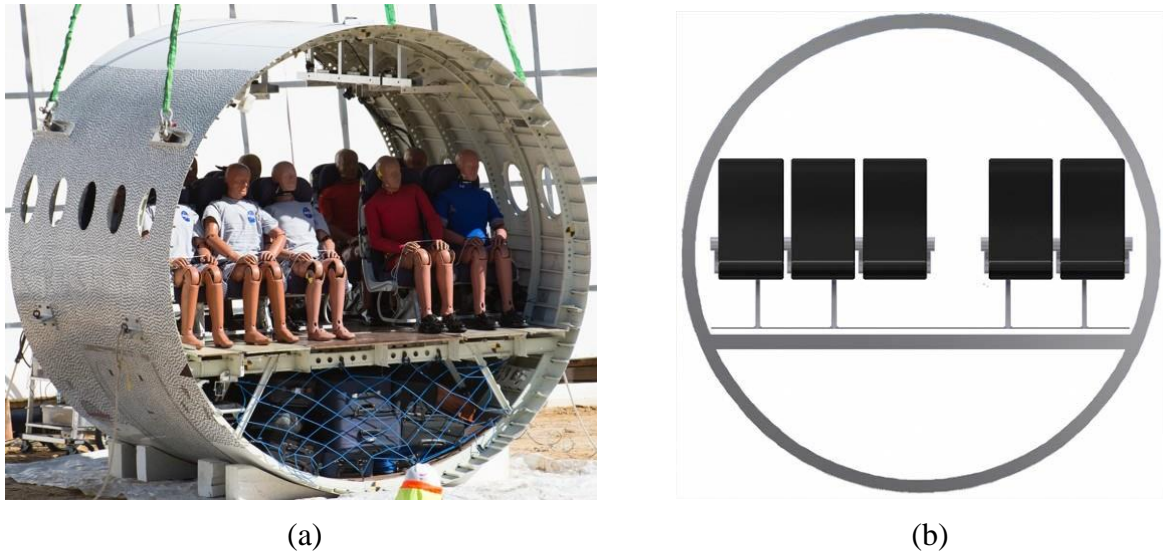
Figure 4. Photograph of the F-28 section and schematic of the 3+2 seat configuration: (a) pre-test photo of the test article and (b) 3+2 seat arrangement
