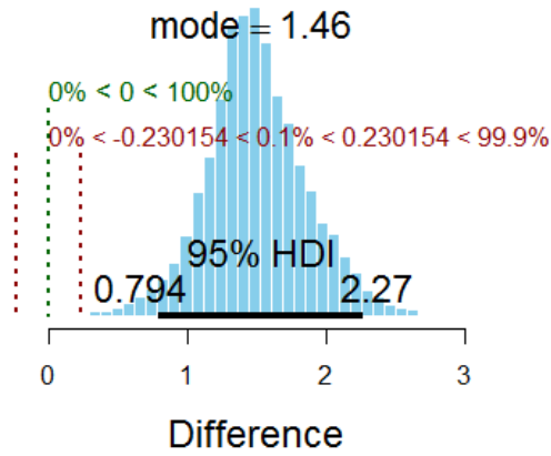
Figure 67. Posterior distribution displaying a 95% HDI, comparison to zero, and ROPE for the CP Location analysis of ratings of overall CP use.
