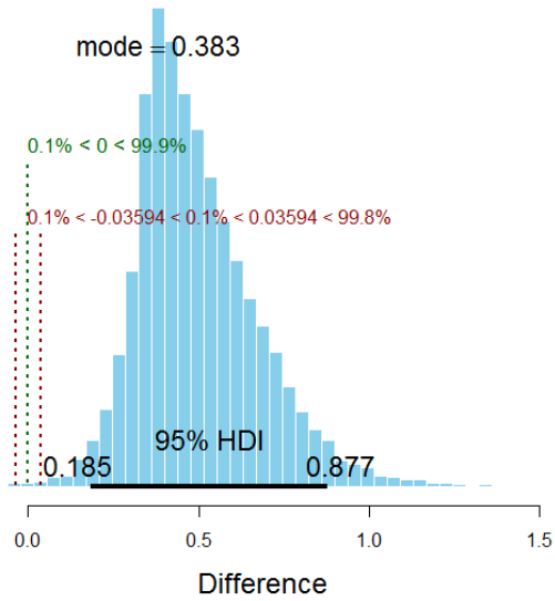
Figure 15. Posterior distribution displaying a 95% HDI, comparison to zero, and ROPE for CP Algorithm analysis of nuisance alerts.
