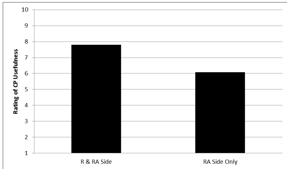
Figure 38. Graph of the mean estimates from the CP Location analysis of controller confidence in CP accuracy.
