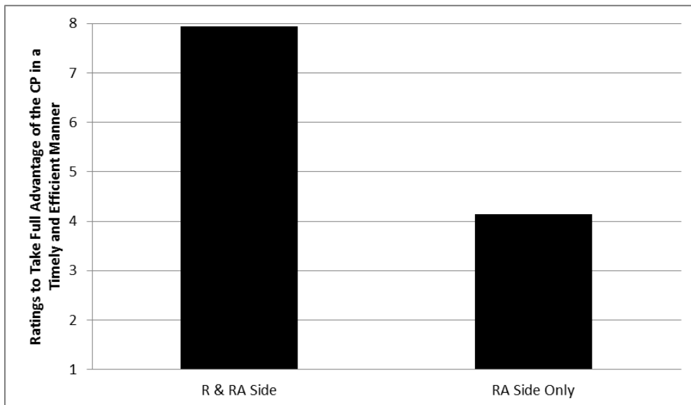
Figure 66. Graph of the mean estimates from the CP Location analysis of the ratings of taking full advantage of the CP in a timely and efficient manner.
