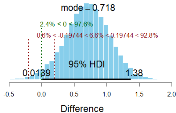
Figure 20. Posterior distribution displaying a 95% HDI, comparison to zero, and ROPE for CP Location analysis of distraction ratings.
