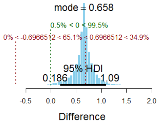
Figure 50. Posterior distribution displaying a 95% HDI, comparison to zero, and ROPE for the CP Algorithm analysis of ratings of prioritizing/preplanning control actions.
