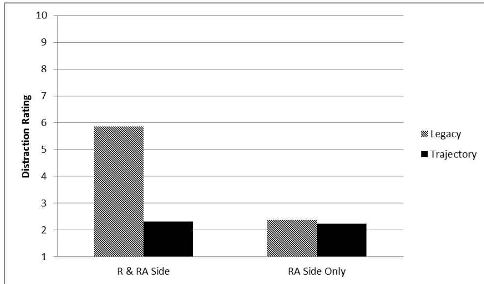
Figure 23. Graph of the mean estimates from the CP Location by CP Algorithm analysis of distraction ratings.
