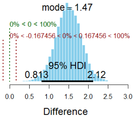
Figure 35. Posterior distribution displaying a 95% HDI, comparison to zero, and ROPE for CP Location analysis of usefulness ratings.
