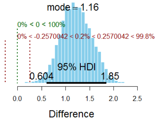
Figure 61. Posterior distribution displaying a 95% HDI, comparison to zero, and ROPE for the CP Location analysis of ratings of overall CP use.
