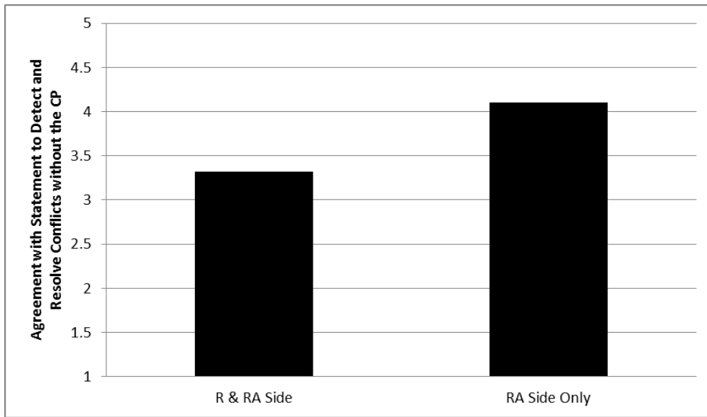
Figure 34. CP Location analysis of the strategy statement to detect and resolve conflicts without the CP (1 = Never; 5 = Always).
