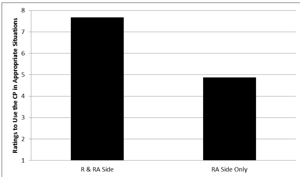
Figure 64. Graph of the mean estimates from the CP Location analysis of ratings of using the CP in appropriate situations.
