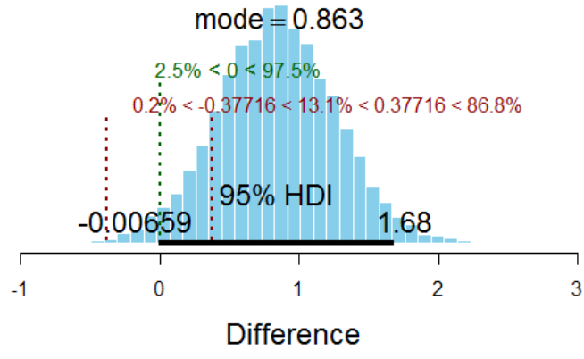
Figure 41. Posterior distribution displaying a 95% HDI, comparison to zero, and ROPE for CP Location analysis of the strategy statement to believe CP Alert but validate with other data.
