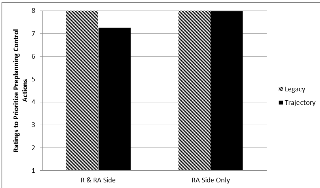
Figure 52. Graph of the mean estimates from the CP Location by CP Algorithm analysis of ratings of prioritizing/preplanning control actions.
