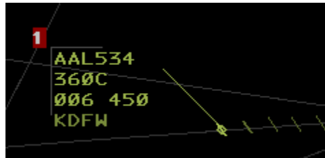
Figure 6. ERAM aircraft representation, including a Full Data Block, displaying the portal fence (gray line on the left and top of the Full Data Block) and the Safety Portal for a single potential conflict.
