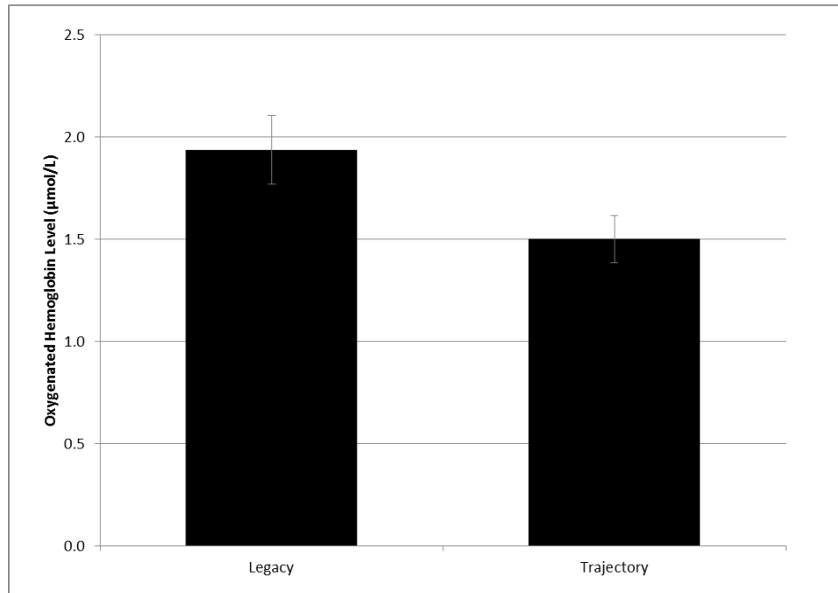
Figure 12. Mean oxygenated hemoglobin levels from fNIRS, by Algorithm condition.
