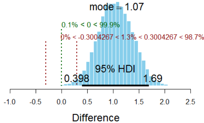
Figure 55. Posterior distribution displaying a 95% HDI, comparison to zero, and ROPE for the CP Location analysis of ratings of using the CP in appropriate situations.
