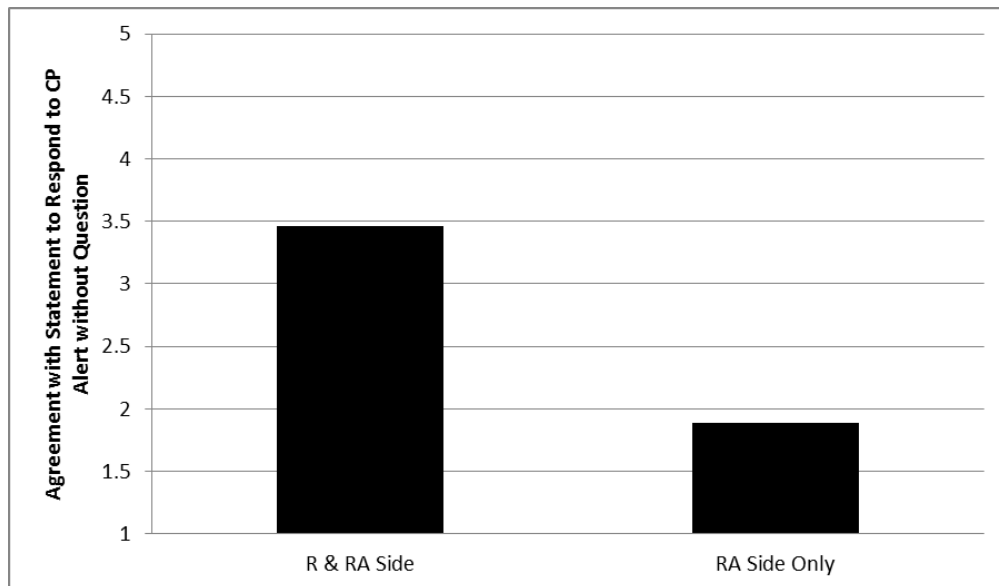
Figure 40. Graph of the mean estimates from the CP Location analysis of the strategy statement to respond to CP Alert without question (1 = Never; 5 = Always).
