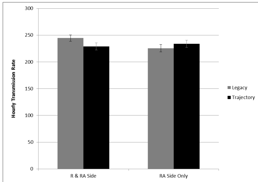
Figure 77. Mean transmissions per hour on PTT by Location and Algorithm.
