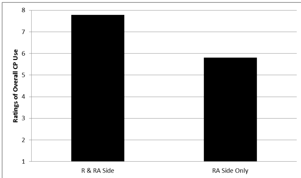
Figure 62. Graph of the mean estimates from the CP Location analysis of the ratings of overall CP use.
