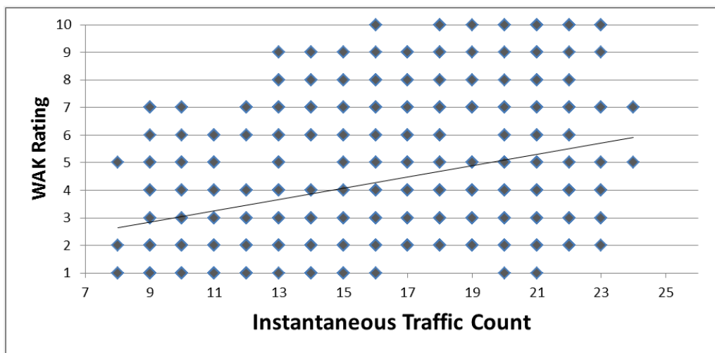
Figure 11. WAK rating as a function of instantaneous traffic count.
