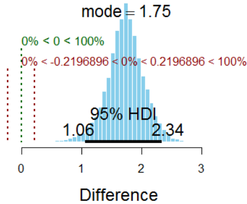
Figure 65. Posterior distribution displaying a 95% HDI, comparison to zero, and ROPE for the CP Location analysis of ratings of taking full advantage of the CP in a timely and efficient manner.
