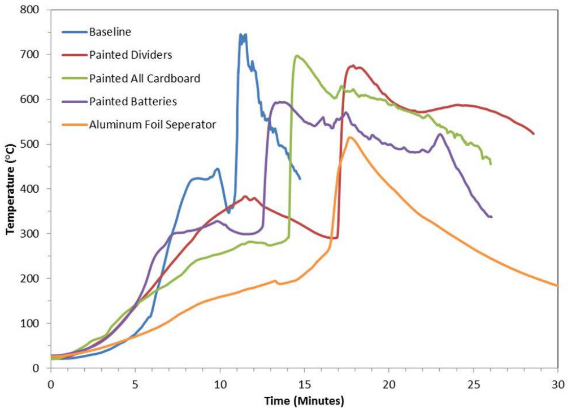
Figure 53. Timelines for first cell to enter thermal runaway
