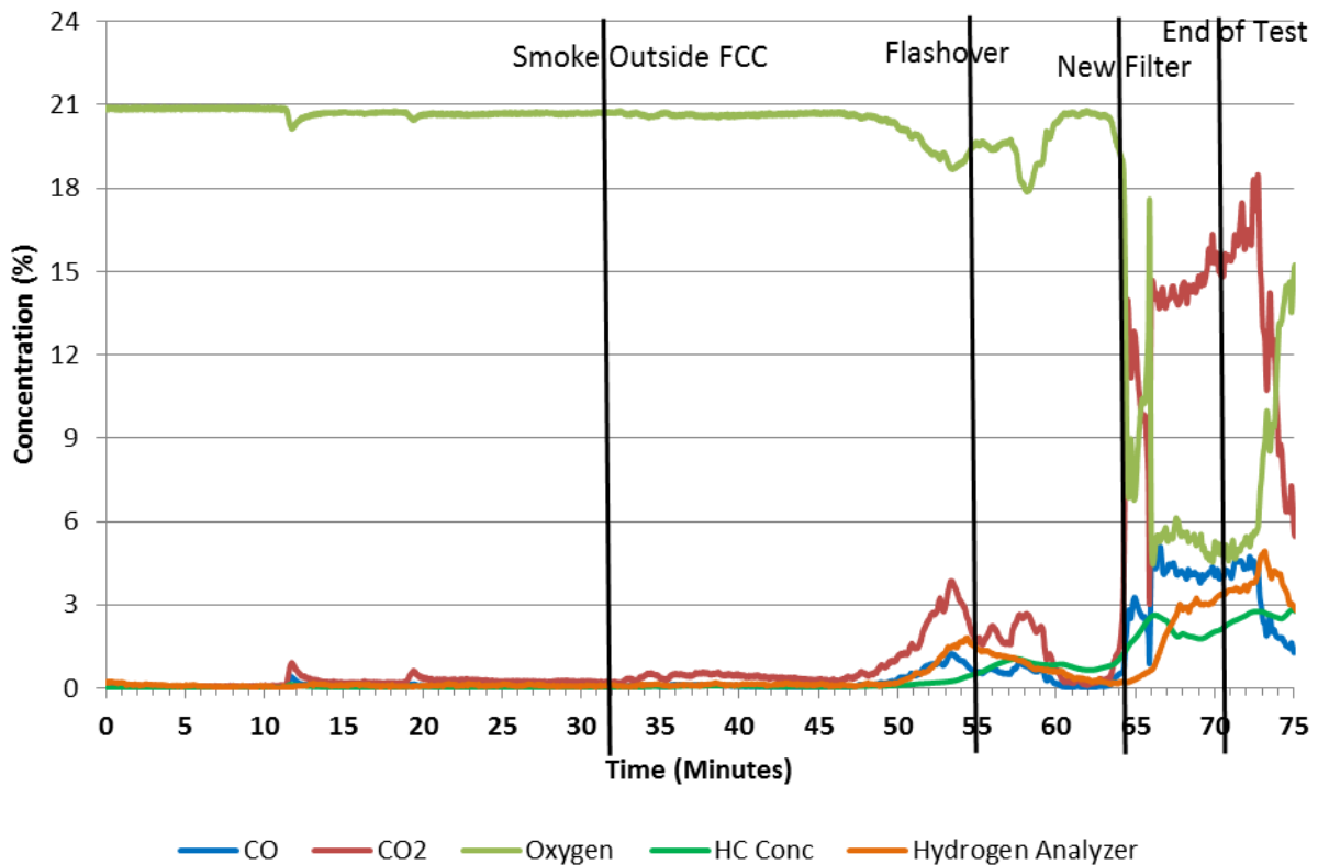
Figure 27. Gas analysis of the 5000 lithium-ion cell fire test
