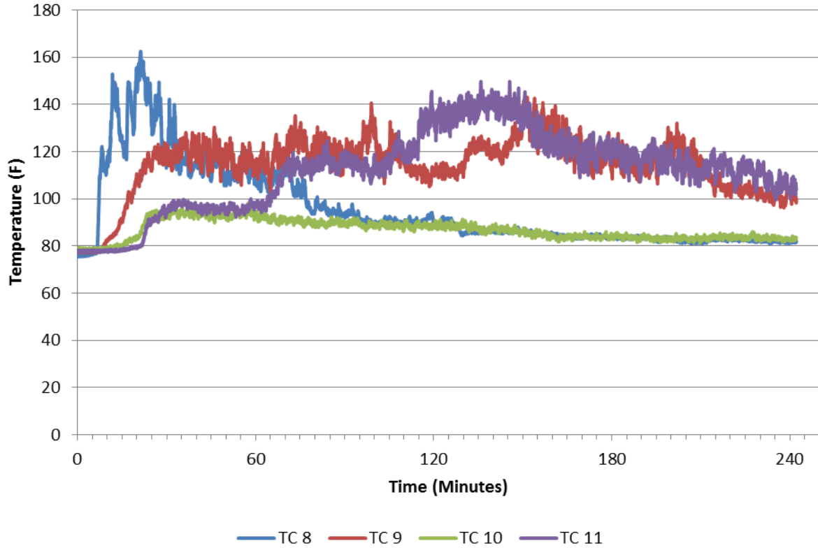
Figure 25. Results from a full-scale fire test of an FCC
