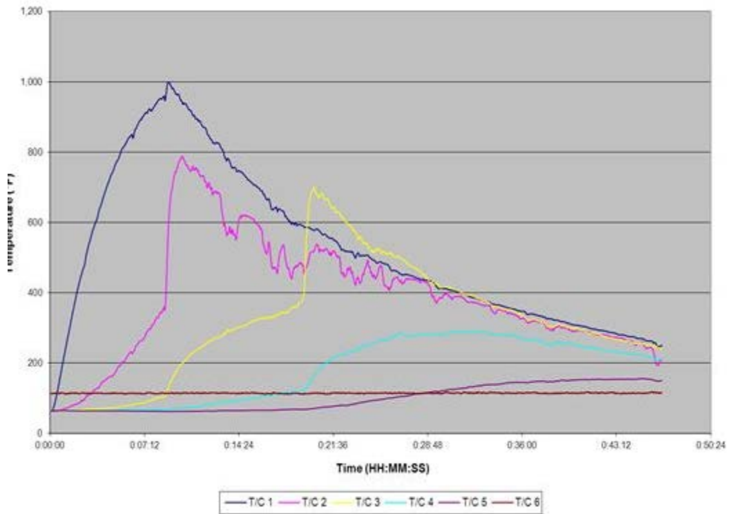
Figure 12. The LiCoO 2 18650 cell SOC thermal runaway propagation tests
