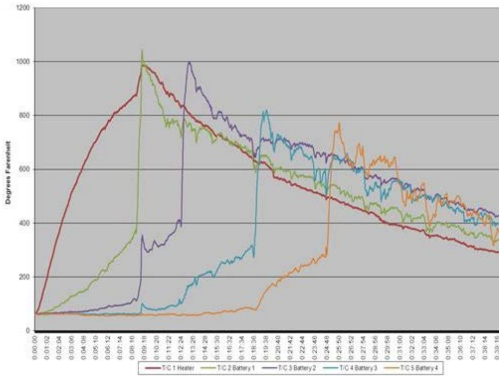
Figure 12. The LiCo 2 18650 cell SOC thermal runaway propagation tests (continued)
