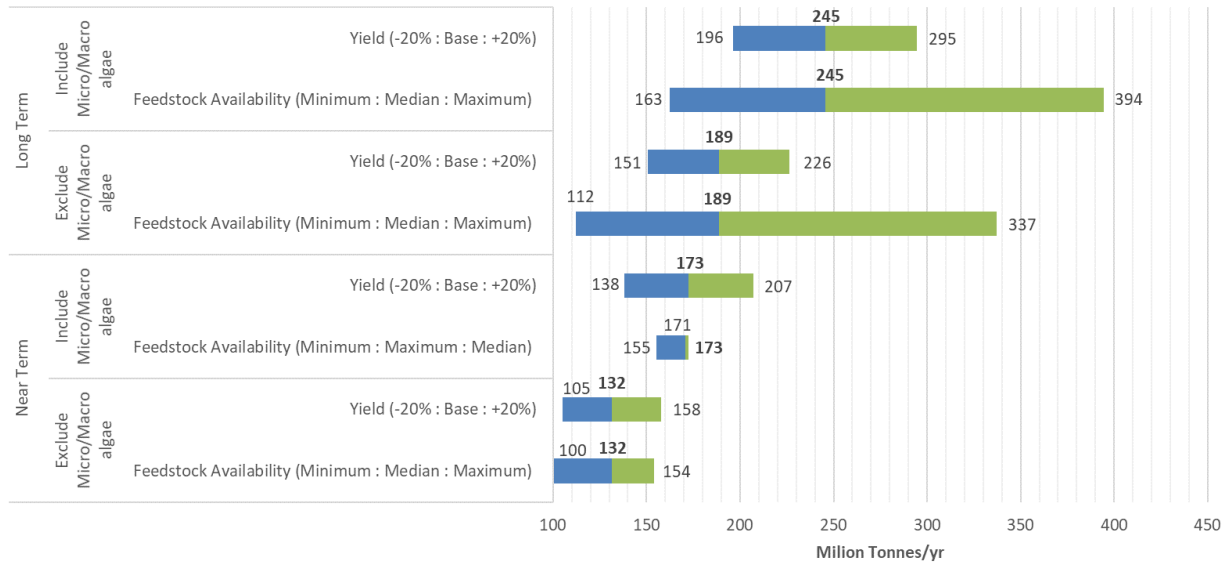
Figure 30. Sensitivity analysis for total biofuel production on a per-ton basis. Median (baseline case) for each scenario is shown in bold.
