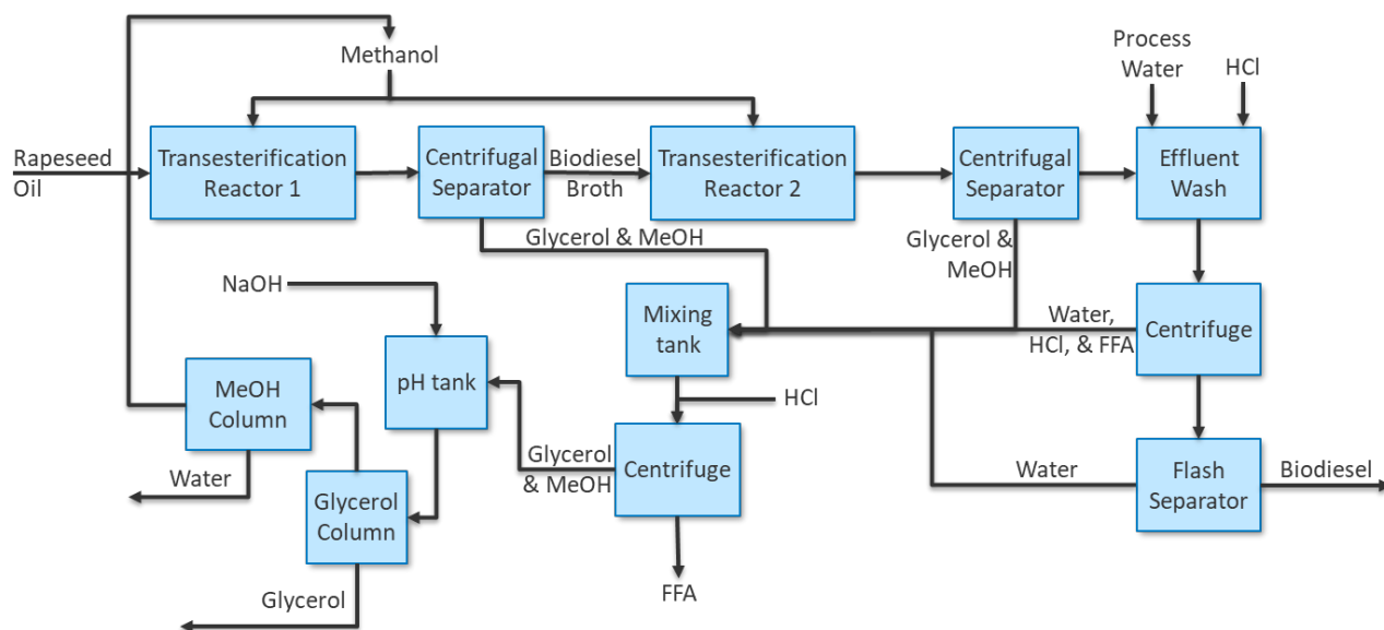
Figure B2. Simplified block flow diagram for biodiesel production from rapeseed oil via alkali catalysts
