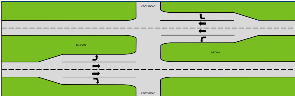
Figure 1.1 - Standard At-Grade Expressway Intersection Layout
