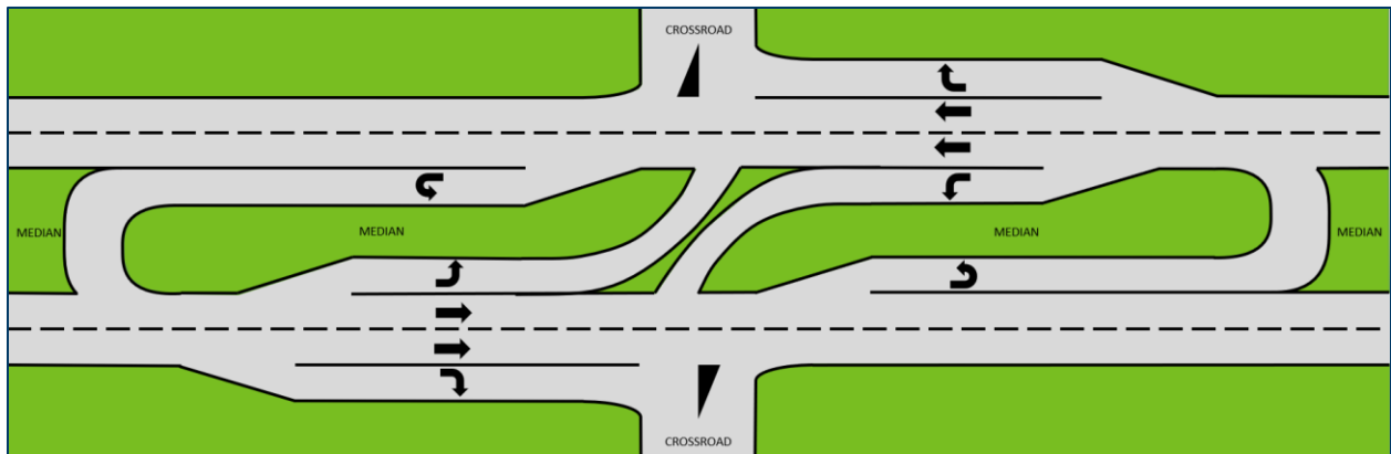
Figure 1.2 - Standard At-Grade Expressway Intersection Layout
