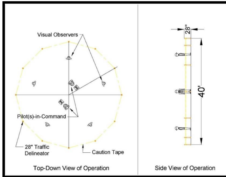
Figure 2 Flight Site Configuration
