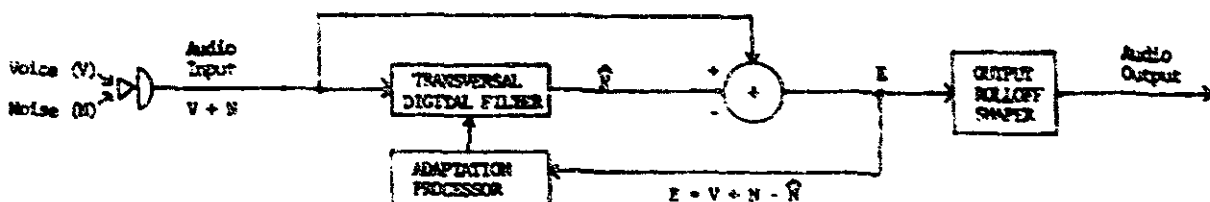
Fig. 4 Deconvolution filter design where \hat{N} is the estimated noise. (Courtesy of Digital Audio Corporation.)
