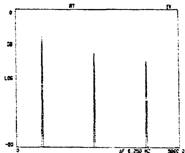
Fig. 3 FFT display of 800-Hz square wave (0-5-kHz range)
