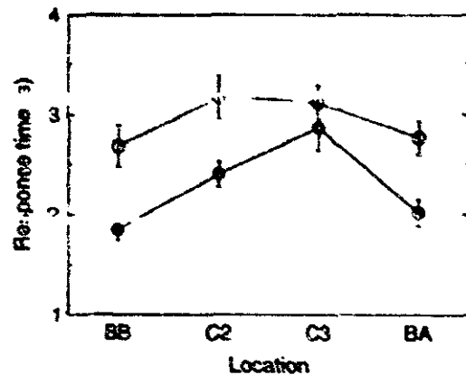
Figure 4. Mean response time to the simple (e) and complex (o) sentences of the RITLS for four subjects at four locations (BB=Base Camp before the climb, C2=Camp Two, C3=Camp Three, BA=Base Camp after the climb). Error bars show standard error.
