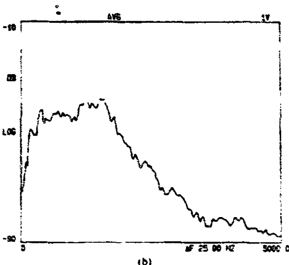
Fig. 8. FFT display of long-term spectrum (0-5-kHz range): (a) Particular male speaker (b) Particular male speaker on a typical forensic recording.
