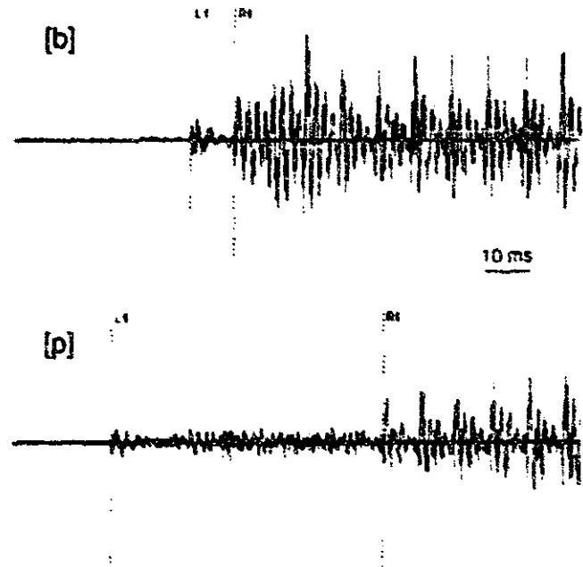
Figure 1. Speech waveform segments corresponding to a [b] and a [p] spoken by the same speaker under identical conditions. Cursors have been placed at the onset of the burst that was caused by opening the lips (LI) and at the onset of periodicity that indicates vocal fold vibration (RI). The marked interval, Voice Onset Timing (VOT) is used by speakers and listeners to differentiate the two types of consonants in word-initial positions.
