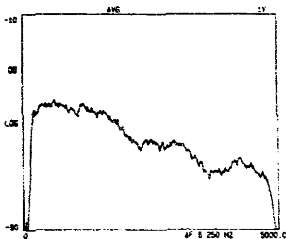
Fig. 10. FFT display of room recording after processing by deconvolutional filter (0-5 kHz range)
