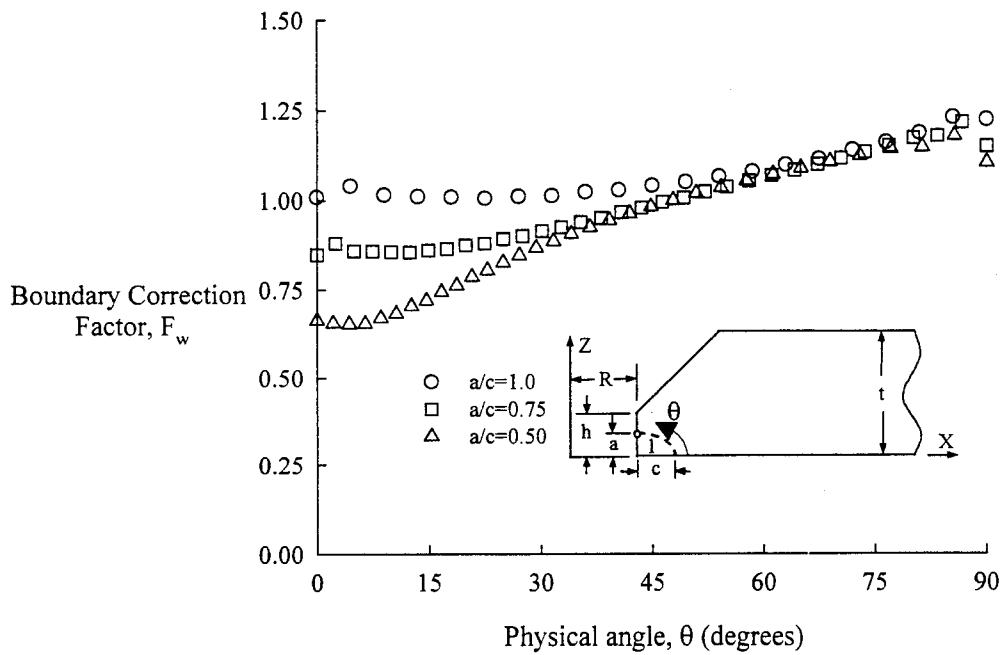
FIGURE 30. BOUNDARY CORRECTION FACTORS, F_w , FOR CRACK LOCATION 1 UNDER WEDGE LOADING, h/t = 0.25
