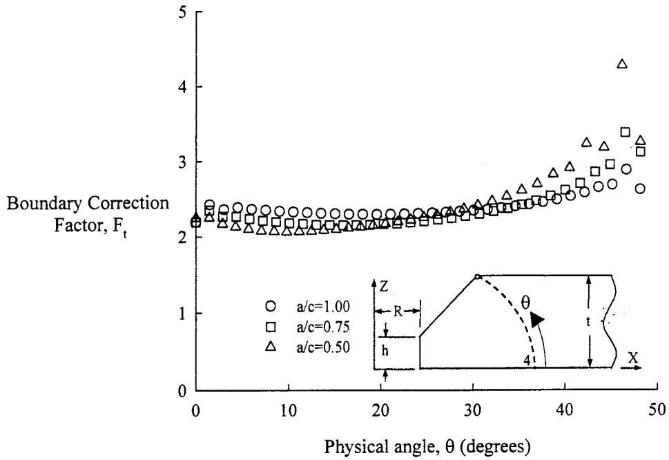
FIGURE 13. BOUNDARY CORRECTION FACTORS, F_t , FOR CRACK LOCATION 4 UNDER TENSION, h/t = 0.25
