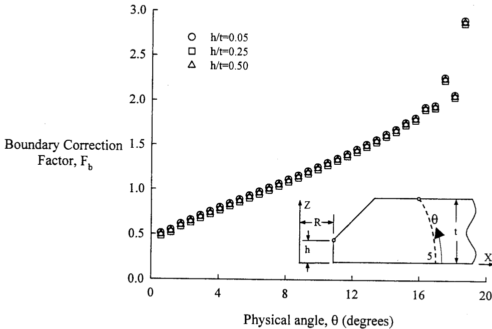
FIGURE 28. BOUNDARY CORRECTION FACTORS, F_b , FOR CRACK LOCATION 5 UNDER BENDING, h/t = 0.05, 0.25, 0.50 ; AND a/c = 1.0
