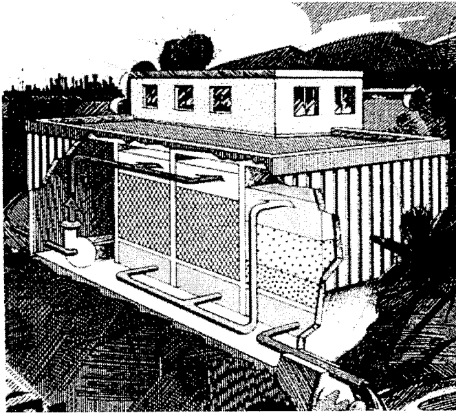
Fig 6: BIOPUR treatment plant
