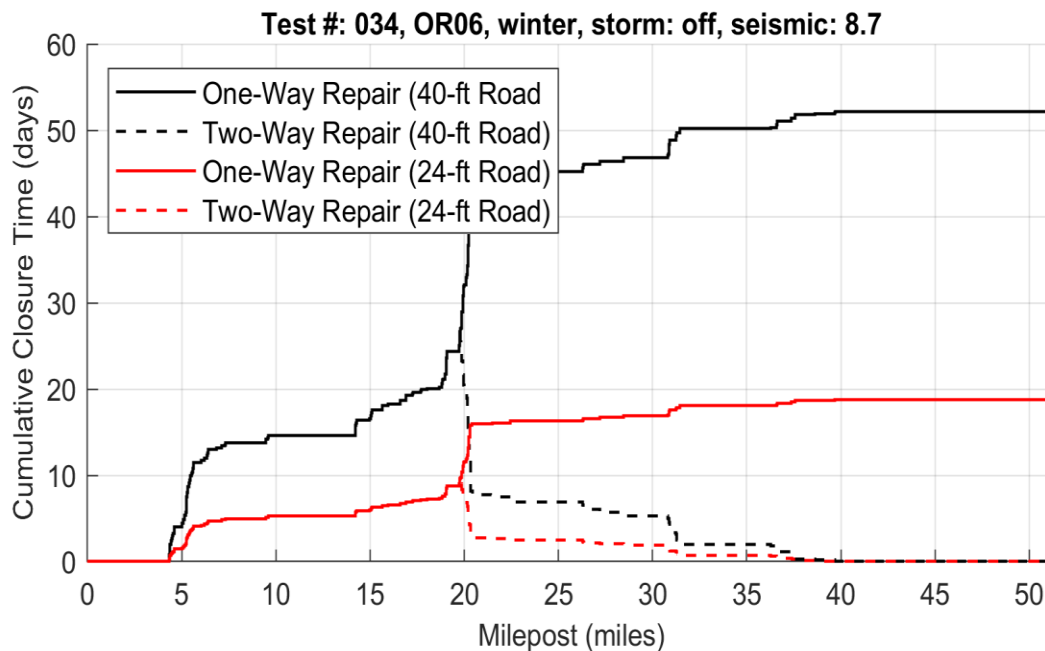
Figure 4.109: Profile of cumulative closure time for OR06: winter antecedent conditions, M8.7 earthquake (test #: 034).
