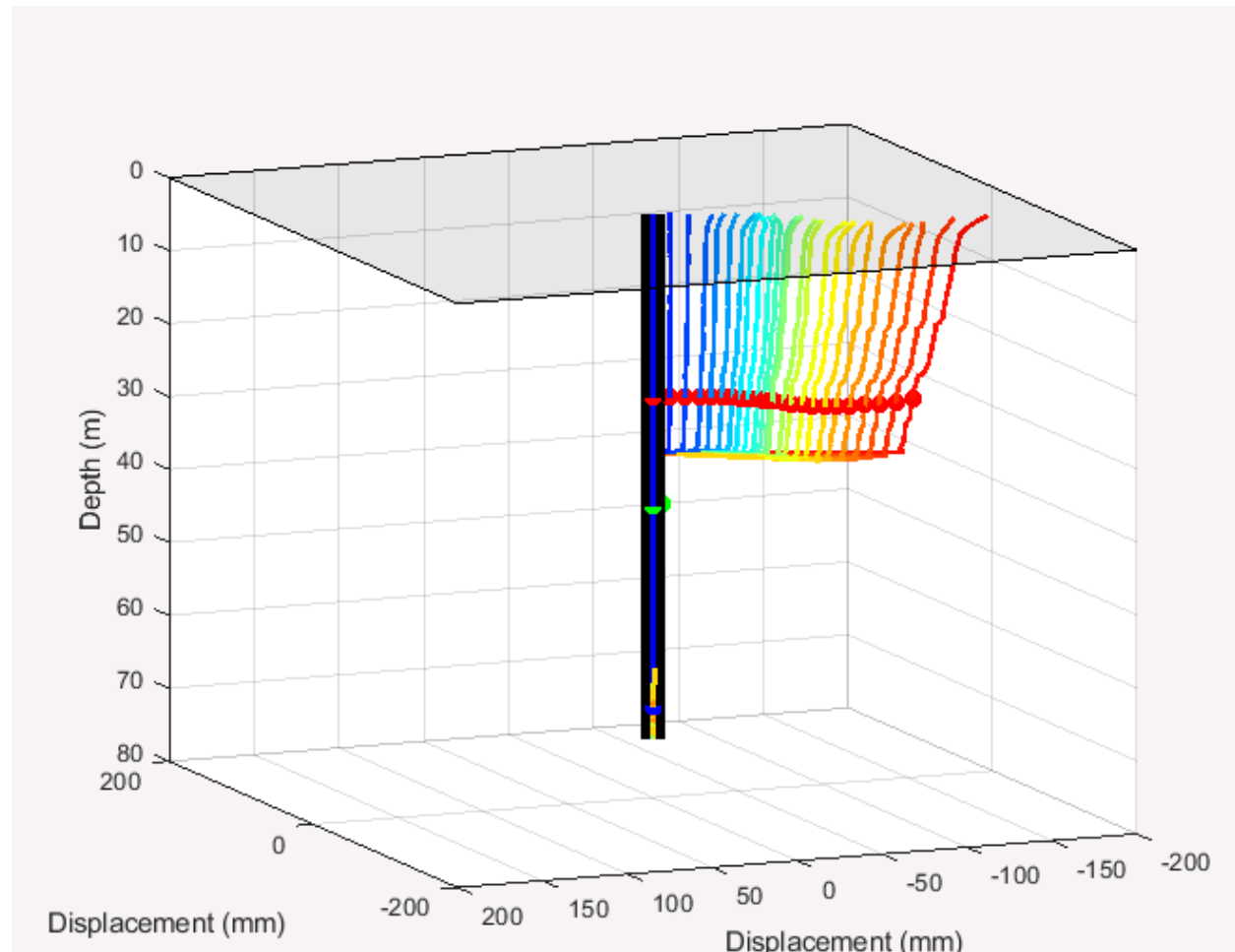
Figure 3.15: Time-dependent inclinometer profile from the Hooskanaden landslide.
