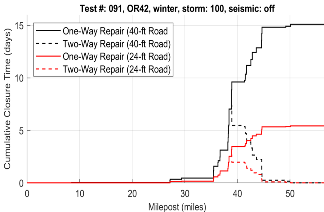
Figure 4.122: Profile of cumulative closure time for OR42: winter, 100-year rainfall event (test #: 091).
