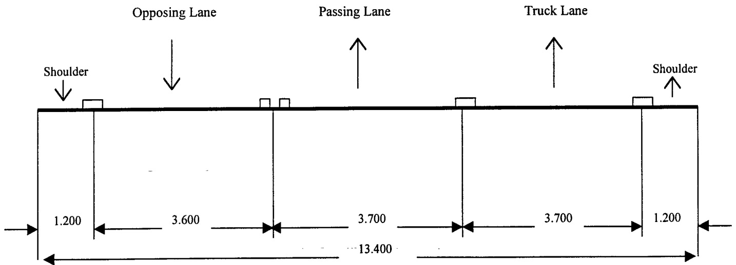
Figure 2-2: Three Lane Highway Cross Section in Canada
