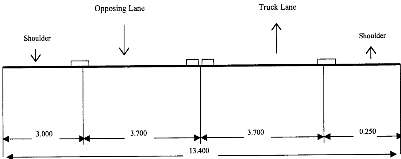
Figure 2-1: Current Two-Lane Rural Highway Cross-section
