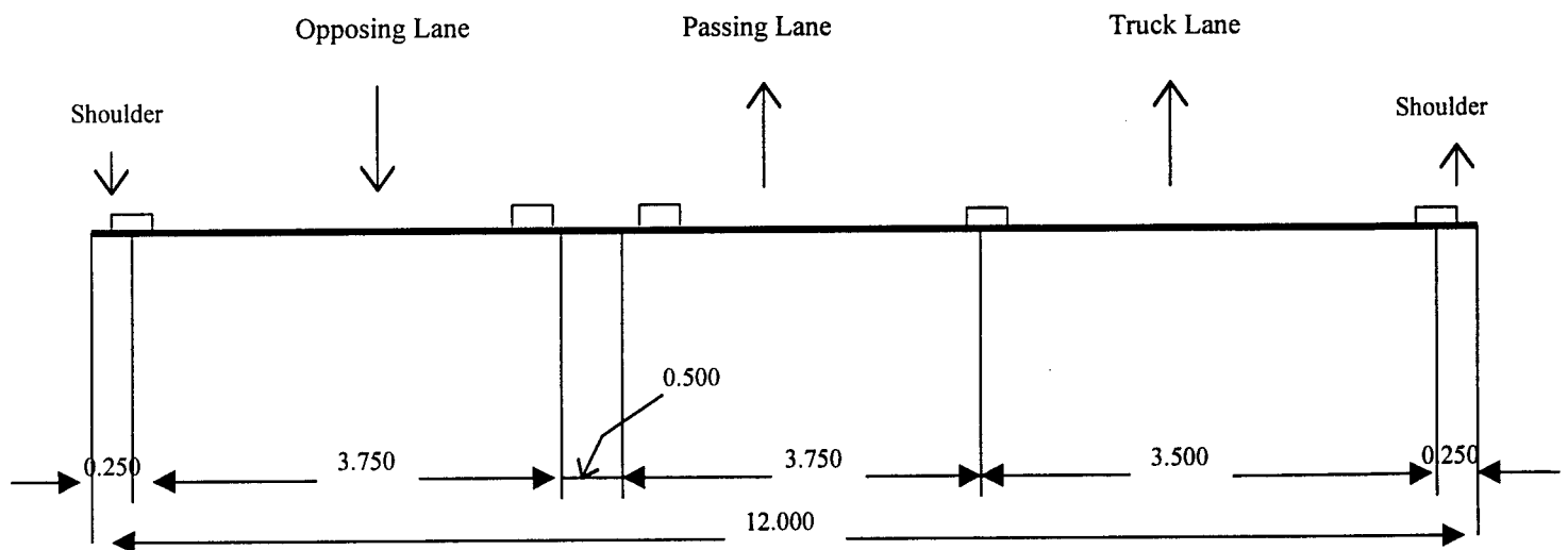
Figure 2-3: Three Lane Highway Cross Section in Germany
