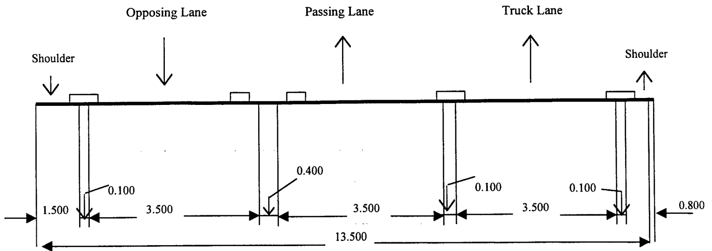
Figure 2-4: Three Lane Highway Cross Section in Mexico
