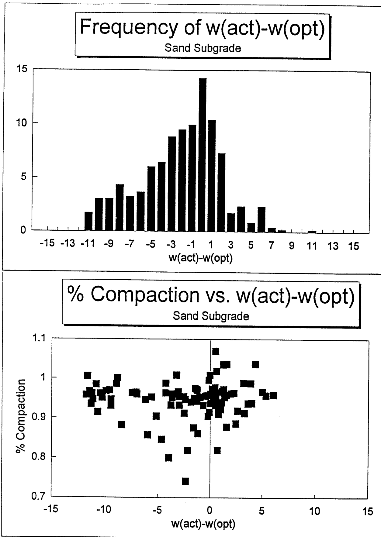
Figure 51. Histogram and comparison of selected volumetric properties of sandy subgrades supporting pavements without any stabilized subgrade layer.
