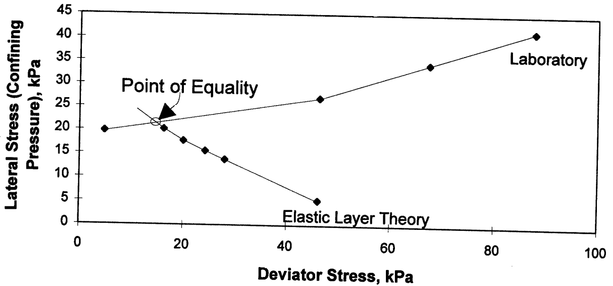
Figure 28. Graphical illustration for procedure used to determine the stress states to be used in the laboratory so that the measured and backcalculated moduli are equal.
