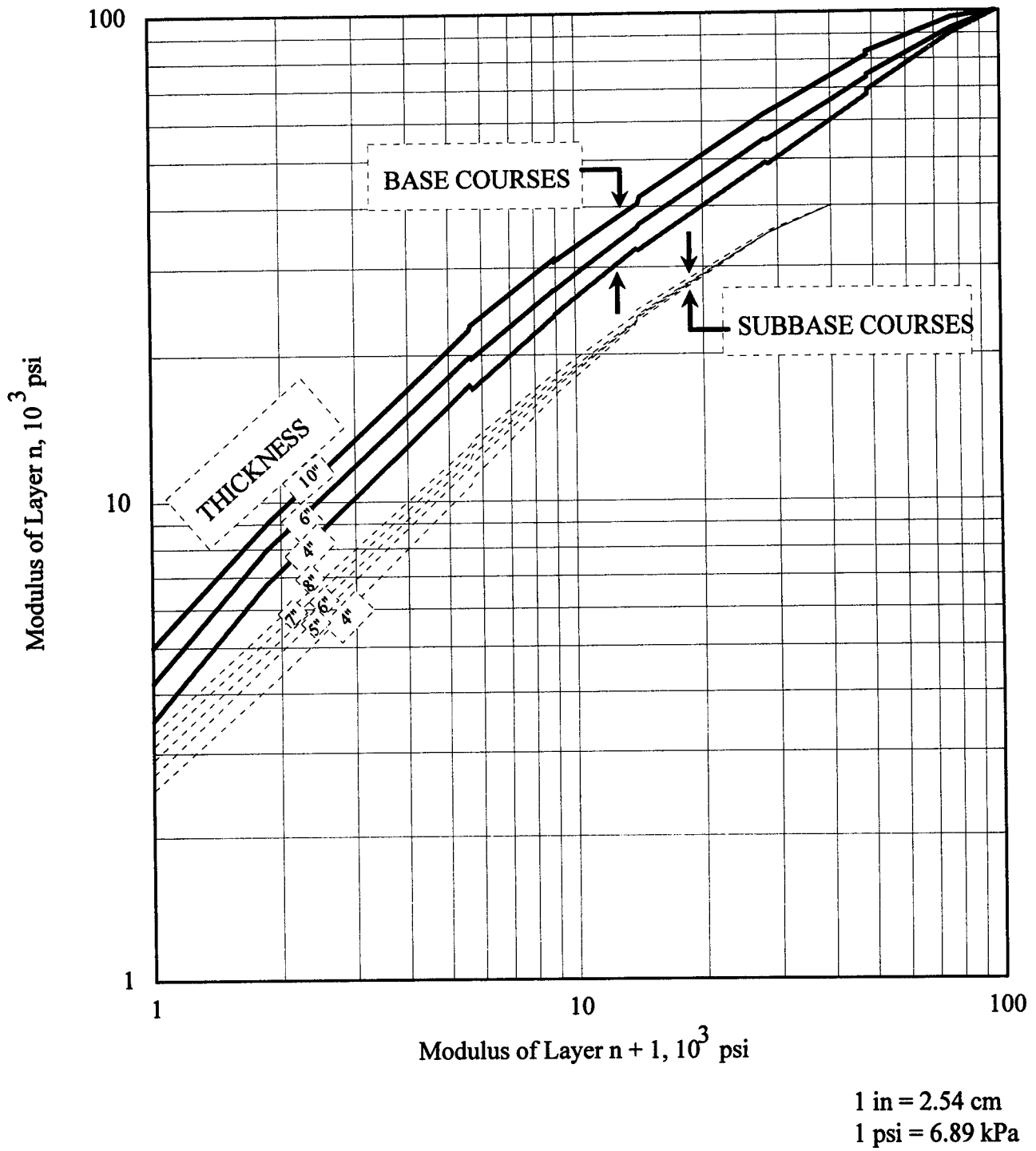
Figure 22. Limiting modulus criteria of unbound base and subbase layers (26).
