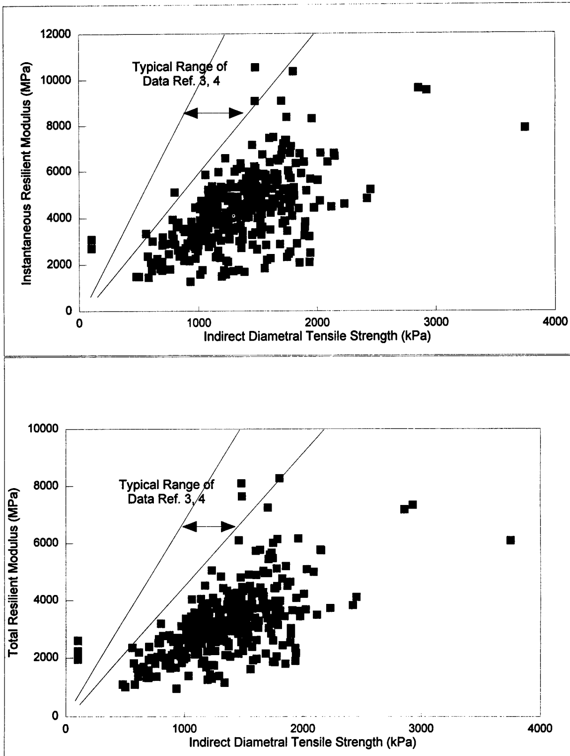
Figure 5. Relationship between indirect tensile strength and total resilient modulus for asphalt concrete materials/mixtures.
