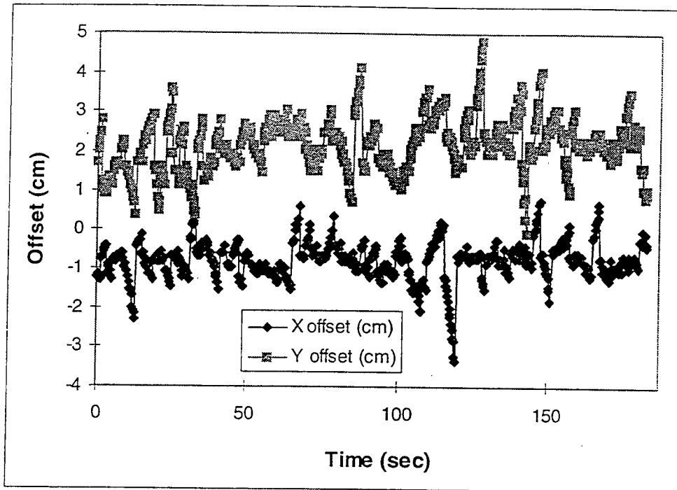
Figure 2.13 11/09/95 Static DGPS offset from true at nail 63, run 1
