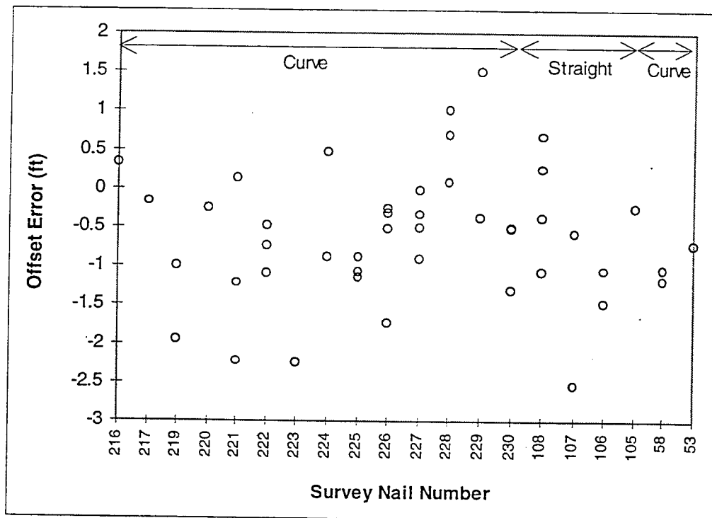
Figure 3.9 Latency adjusted DGPS dynamic error in the direction of motion at all nails: 3/1/96 and 3/5/96 (No data at nails 218 and 57-54)
