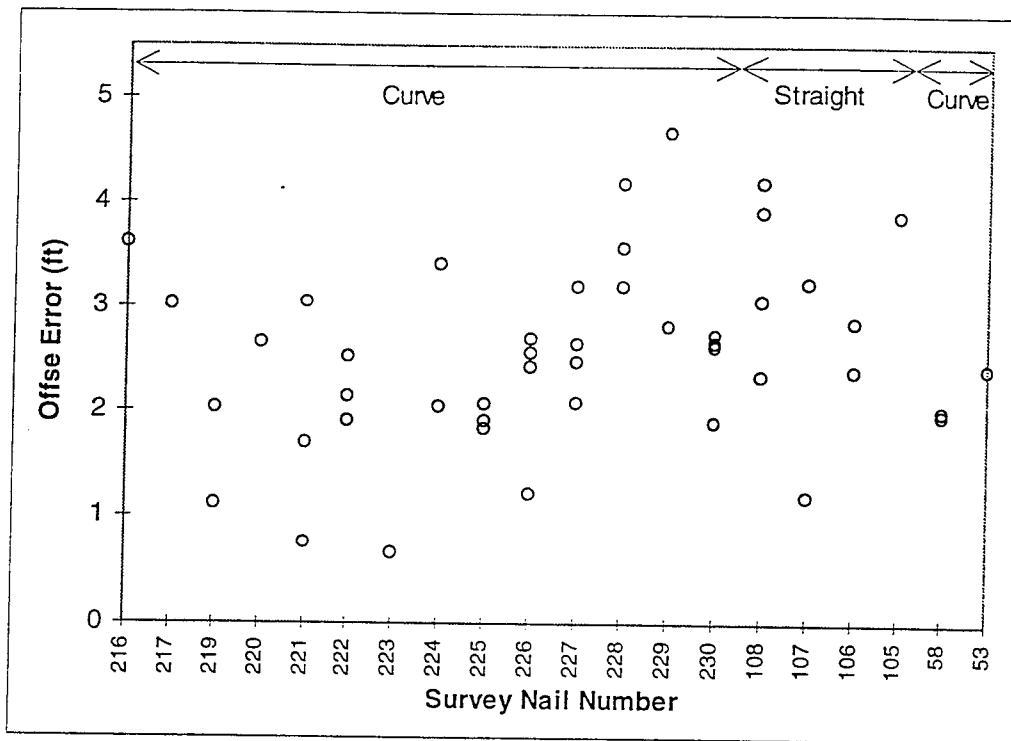
Figure 3.8 Raw DGPS dynamic error in the direction of motion at all survey nails: 3/1/96 and 3/5/96 (No data at nails 218 and 57-54)
