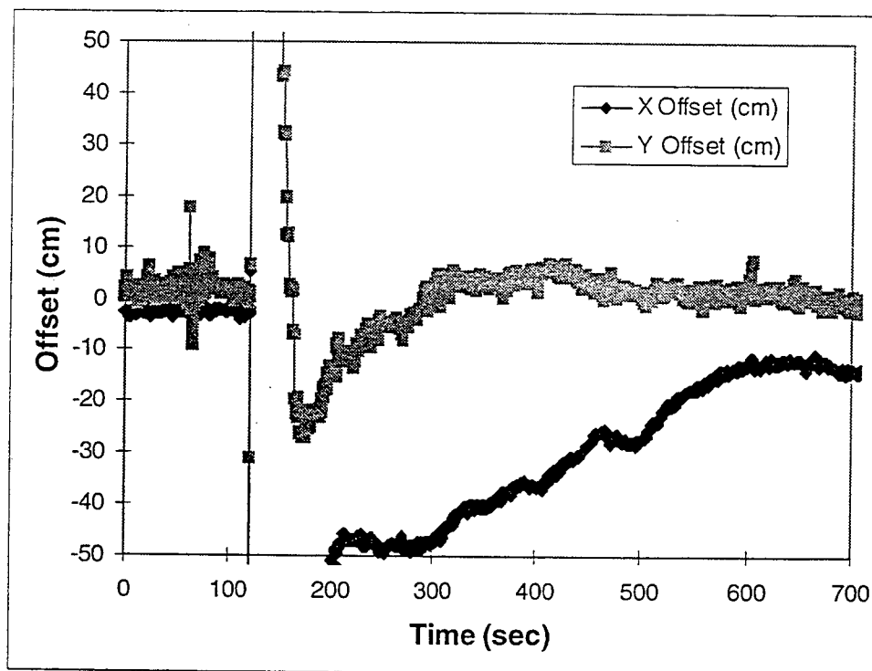
Figure 2.31 11/09/95 Close-up of static DGPS convergence, recovery following full cover at survey nail 101
