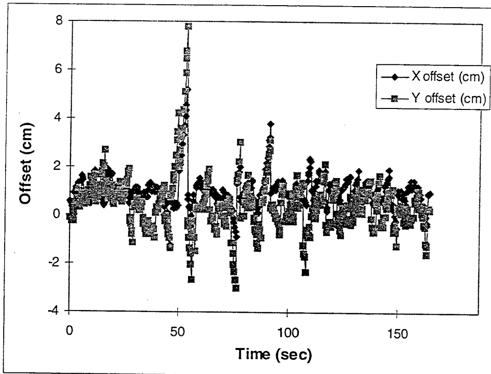
Figure 2.14 11/09/95 Static DGPS offset from true at nail 63, run 2 (approx. 1 hr. after run 1)
