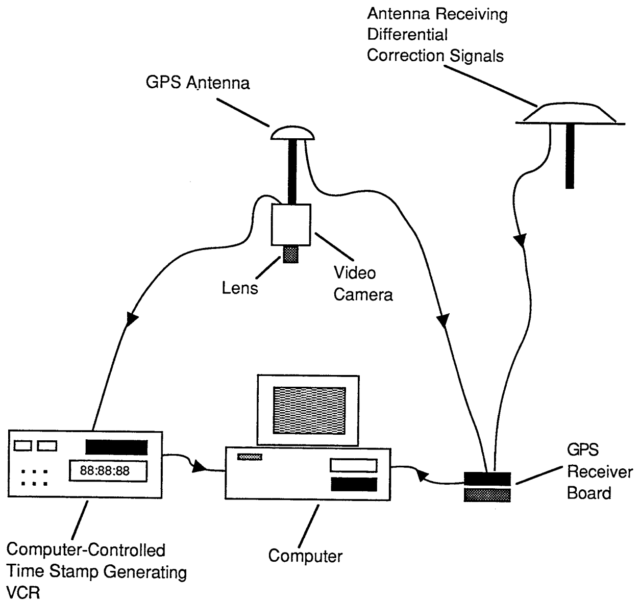
Figure 3.4 Data acquisition for dynamic DGPS evaluation
