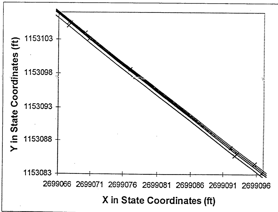
Figure 3.14 10/26/95 Close-up of straight section of 6 laps at Mn/ROAD. Tick mark indicates GPS data collected at that point.
