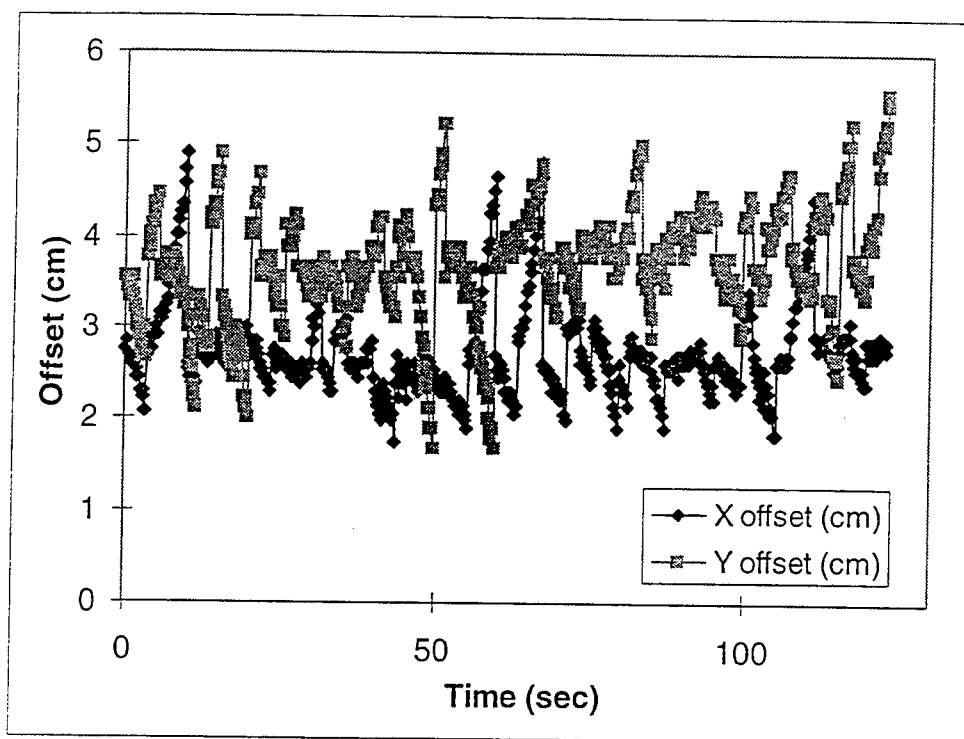
Figure 2.11 9/26/95 Survey nail 175 DGPS offset from true (5 samples/sec collected).
