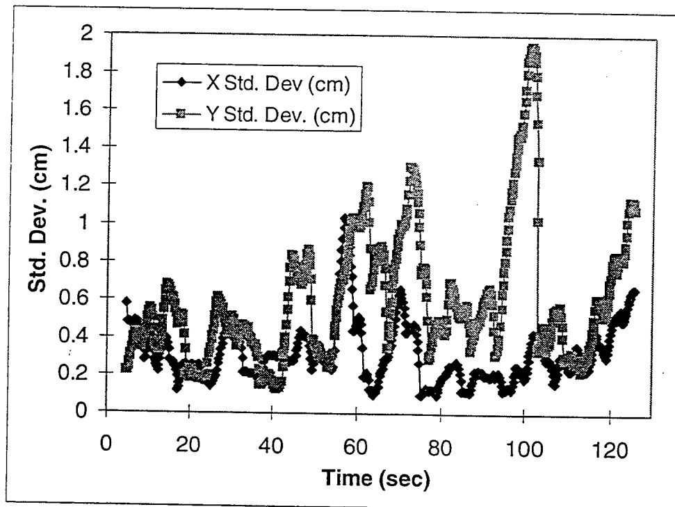
Figure 2.10 9/26/95 Survey nail 101 DGPS running 25 pt standard deviation
