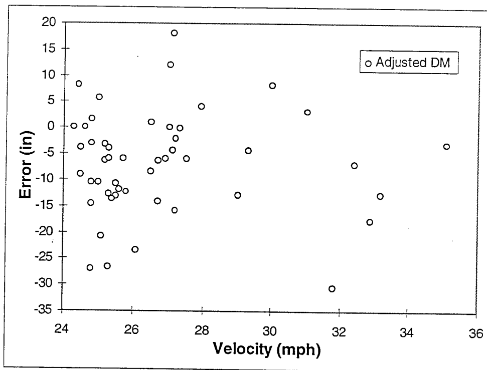
Figure 3.12 Latency adjusted DGPS dynamic error in the direction of motion vs. velocity: 3/1/96 and 3/5/96 collected in the mid afternoon
