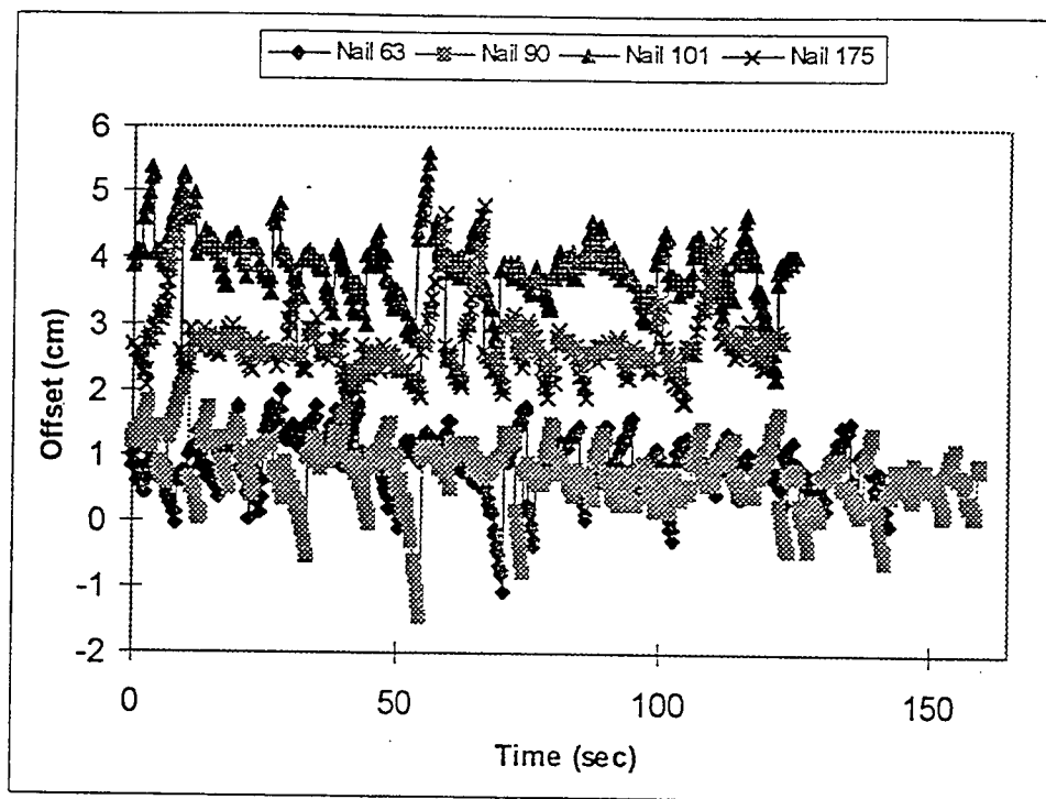
Figure 2.3 9/26/95 Static DGPS X offset from true at four survey nails (5 samples/sec collected).
