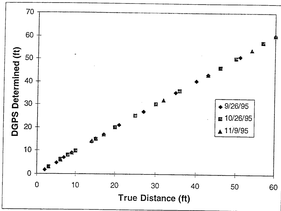
Figure 2.28 DGPS short distance measurements during 3 test sessions
