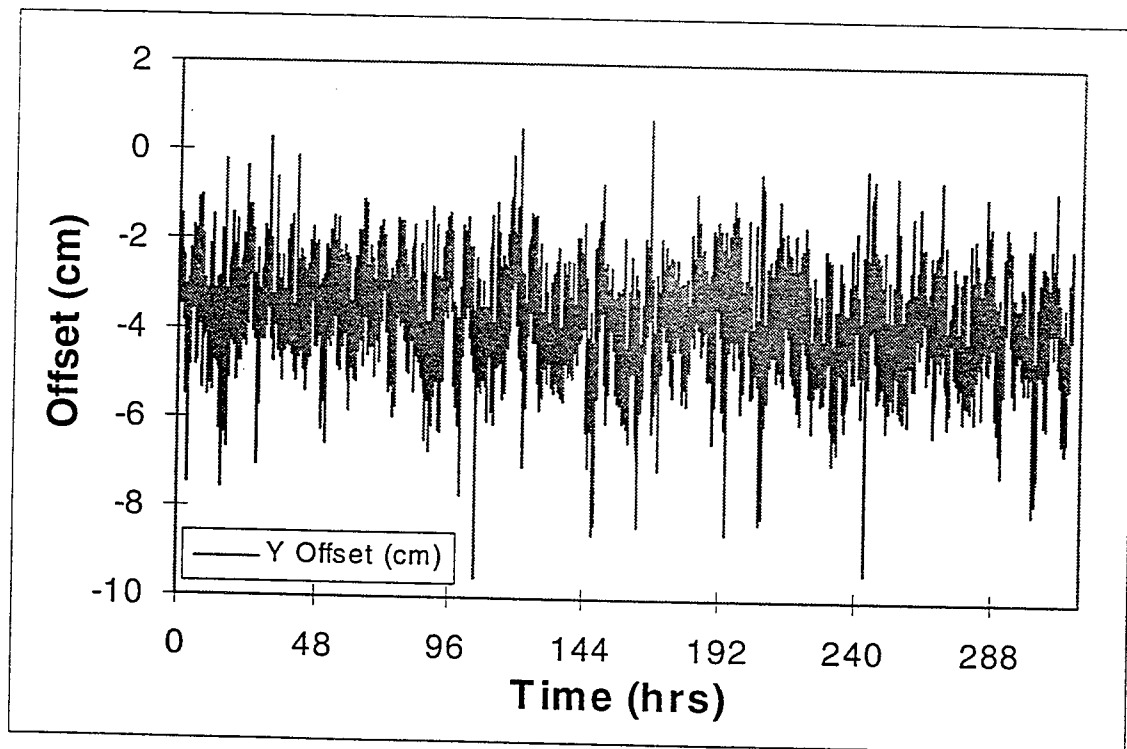
Figure 2.23 Close-up of Y offset during 13 day continuous DGPS log at monument. Data collected at 5 min intervals.
