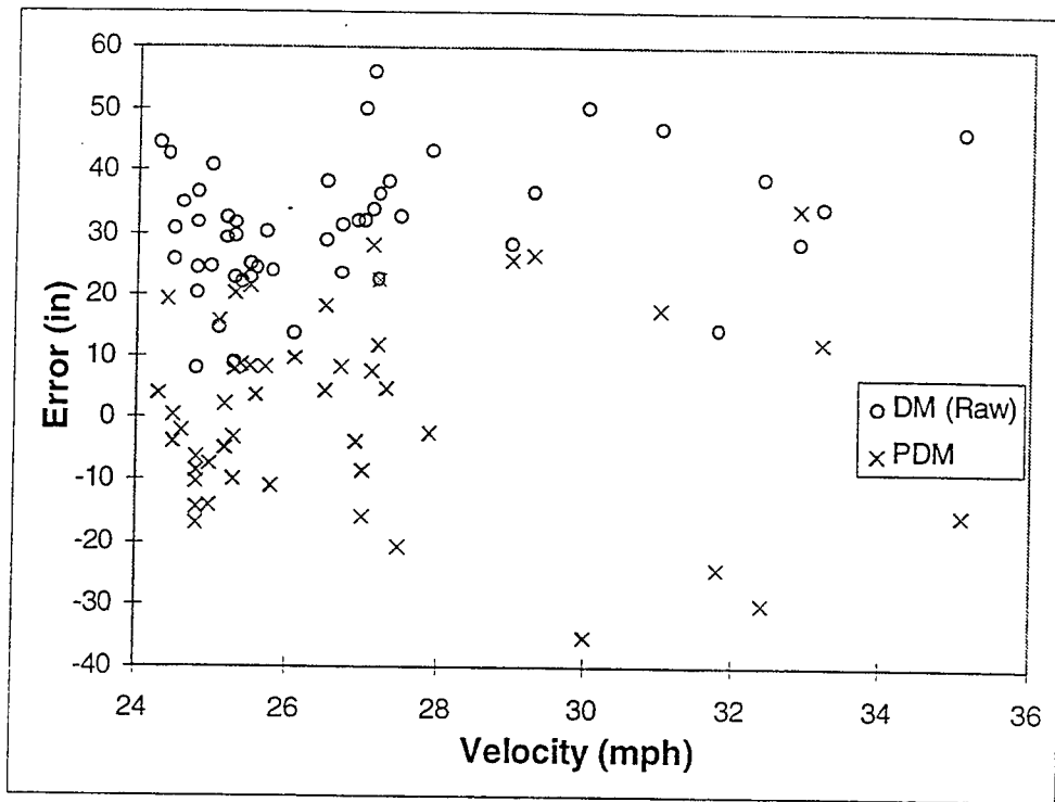
Figure 3.11 Raw DGPS dynamic error vs. velocity: 3/1/96 and 3/5/96 collected in the mid afternoon
