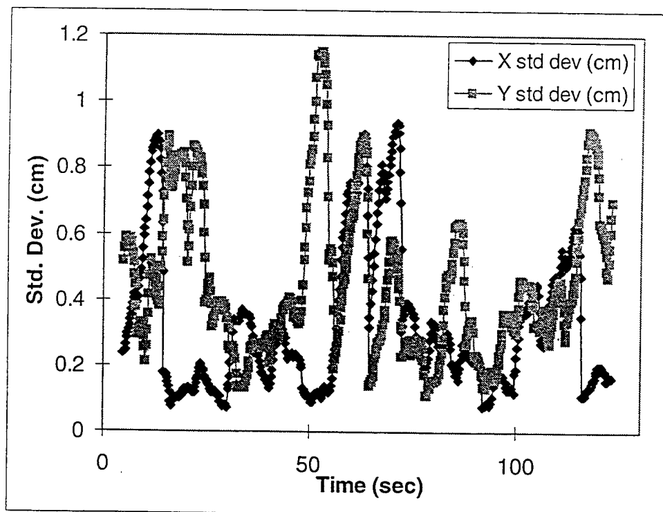
Figure 2.12 9/26/95 Survey nail 175 DGPS running 25 pt standard deviation
