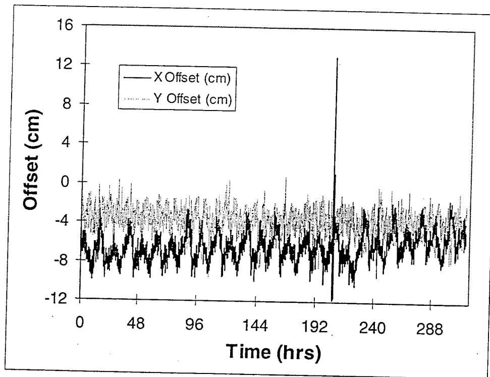
Figure 2.21 13 day continuous DGPS log at monument: position offset from true. Data collected at 5 min intervals.
