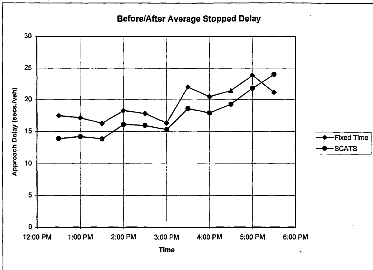
Figure 7.4 Before/After Delay Comparison for Orchard Lake Road Northbound Through Traffic (Orchard Lake Road & Walnut Lake Road Intersection)
