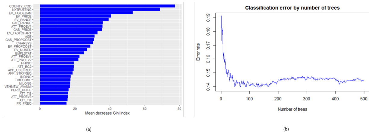
Figure 4. Variable importance (a) and Classification error by number of trees (b)
