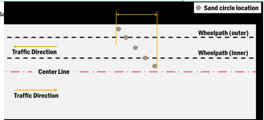
Figure 4.5. Sand circle test
