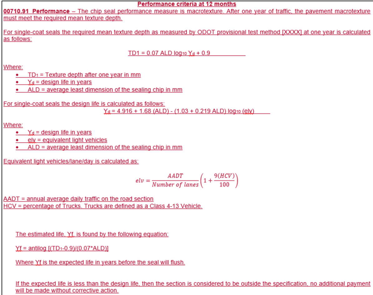
Figure 3.23. Proposed performance criteria to be added to the specification
