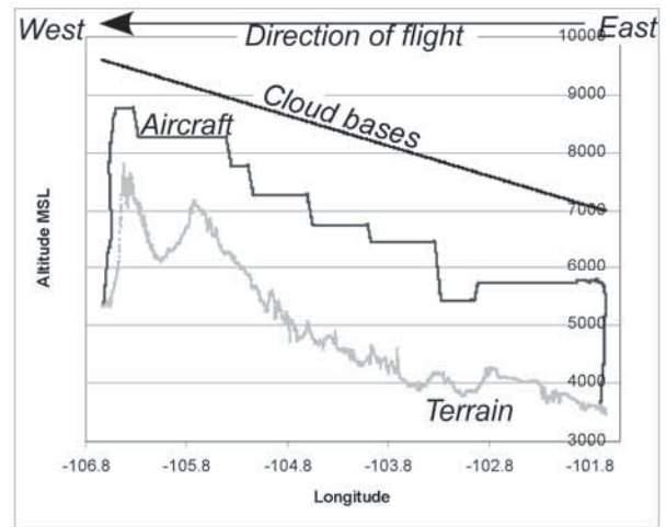
Figure 3. Typical altitude profile, showing maintenance of both ground and cloud clearance.
