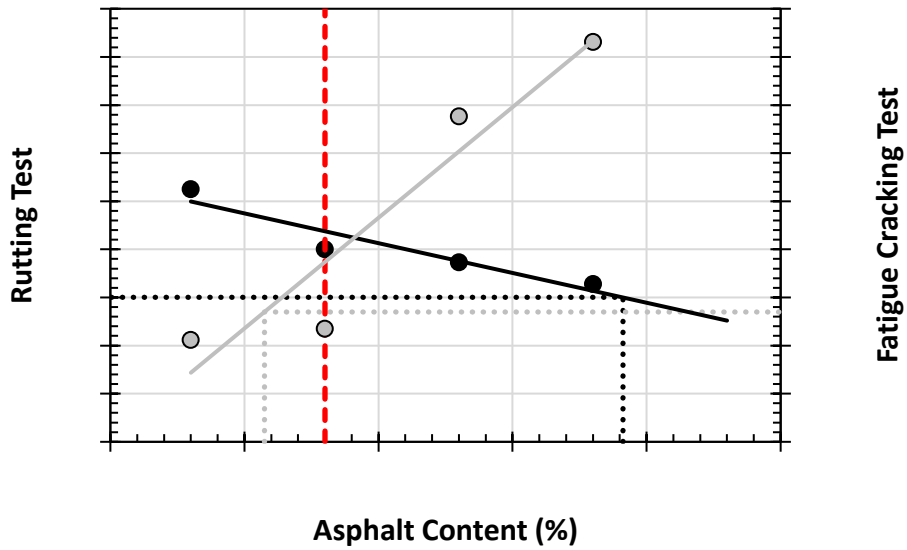
Figure 18 – Example of Balanced Mix Design Graph
