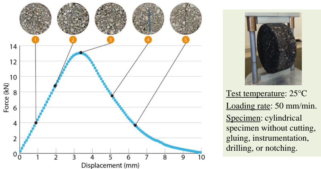
Figure 12 - IDEAL-CT: Specimen, Fixture, Test Conditions, and Typical Result
