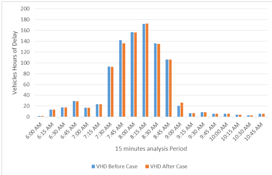
Exhibit 14 Vehicles Hours of Delay for 15 Minute Analysis Periods With & Without Ramp Metering
