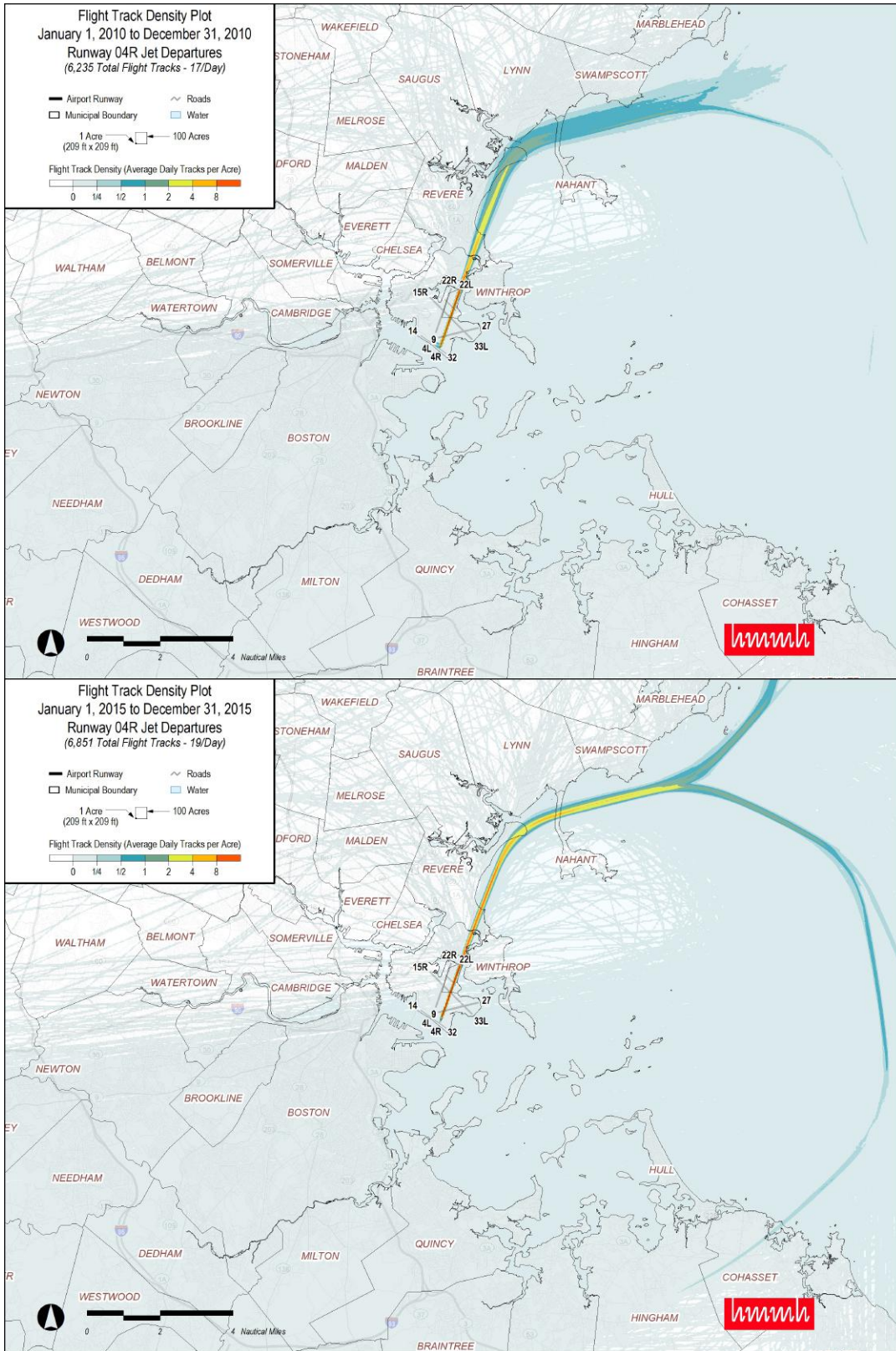
Figure 36. Runway 4R departure flight track densities from 2010 (top) and 2015 (bottom)
