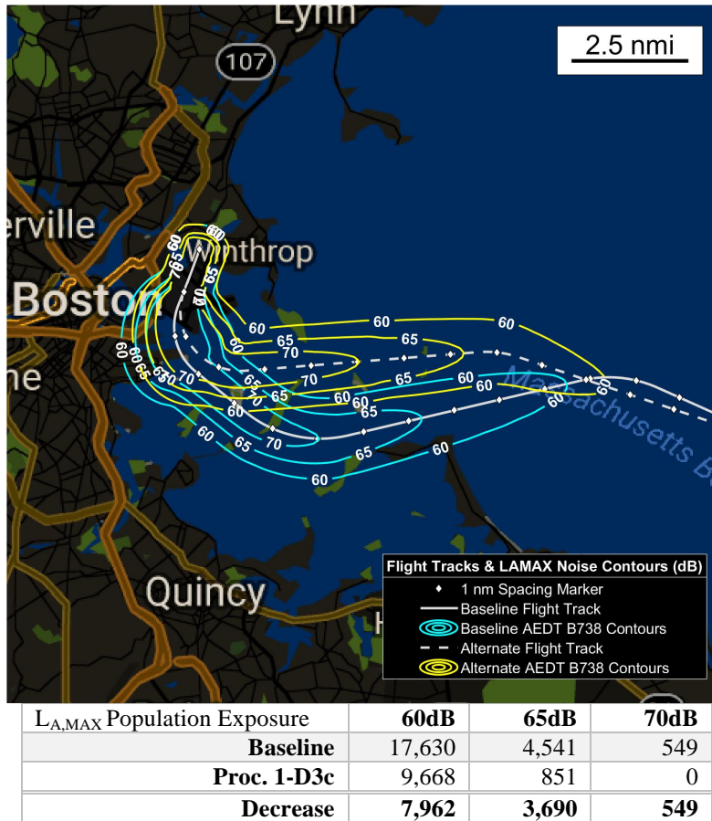
Figure 23. Noise exposure reduction for the Boeing 737-800 departing runway 22R climbing via the BLZZR4 departure on an AEDT-standard climb profile compared to procedure 1-D3c
