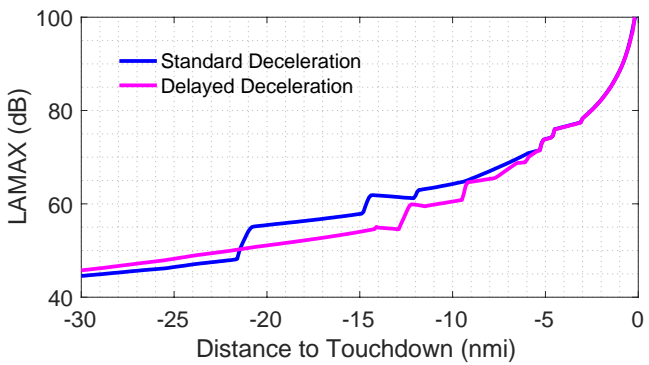
Figure 20. Comparison of Total Noise Levels Under the Flight Track for the Standard and Delayed Deceleration, Boeing 737-800 Approaches
