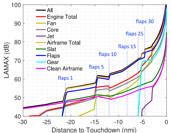
Figure 18. Noise Levels Under the Flight Track for Different Noise Components for a Standard Deceleration, Boeing 737-800 Approach
