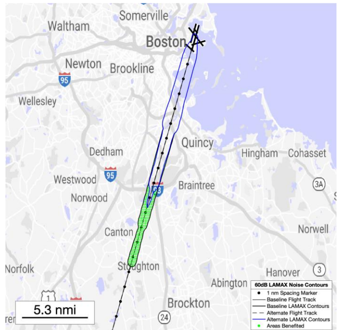
Figure 21. L_{A,MAX} Contours For Boeing 737-800 Performing an ILS Approach with a 4000ft Level Segment Compared to a Delayed Deceleration Approach into BOS Runway 4R
