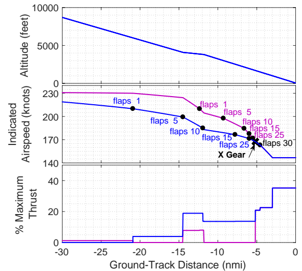
Figure 17. Comparison of Altitude, Velocity, and Thrust Profiles for a Boeing 737-800 Standard Deceleration and Delayed Deceleration Approach
