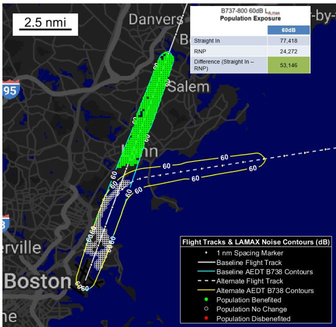
Figure 12. BOS 22L RNAV Approach with RNP Overlay Noise Benefits for Boeing 737-800
