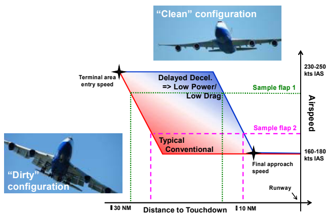
Figure 16. Delayed Deceleration Approach Concept from Ref. [16]
