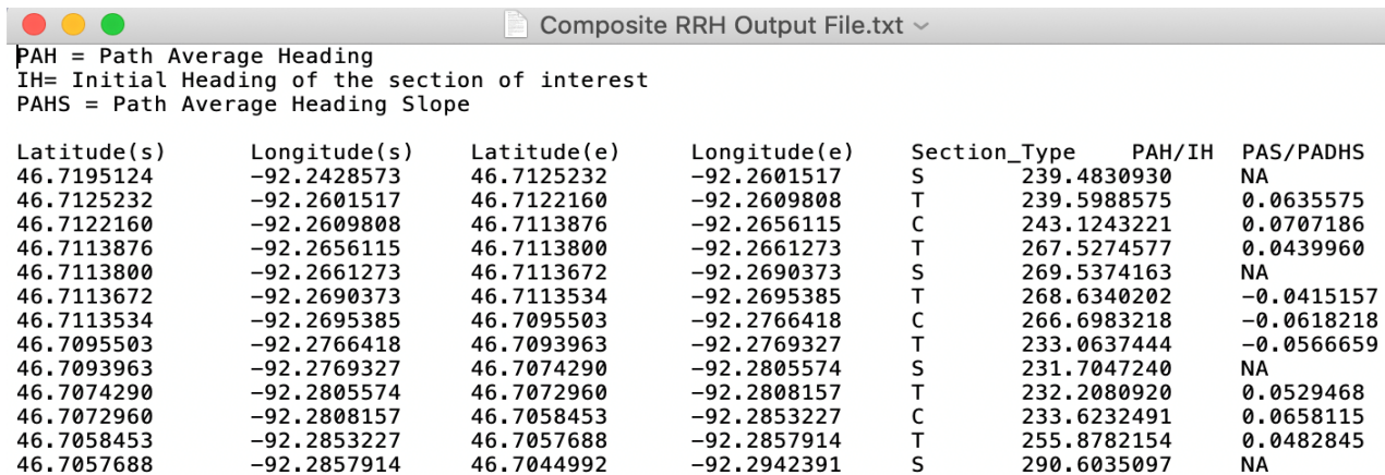
Figure 2.7 Screenshot of a typical output file containing optimized parameters of each section in a composite RRH
