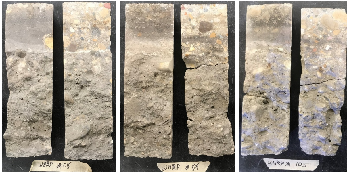
Figure F.2 I-39 Silane-Treated Core Samples, as-received left, cleaned right
