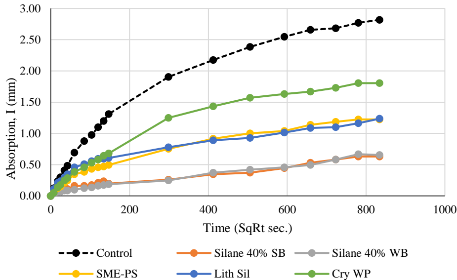
Figure 4.1 Absorption Results for Initial Penetrating Sealer Products
