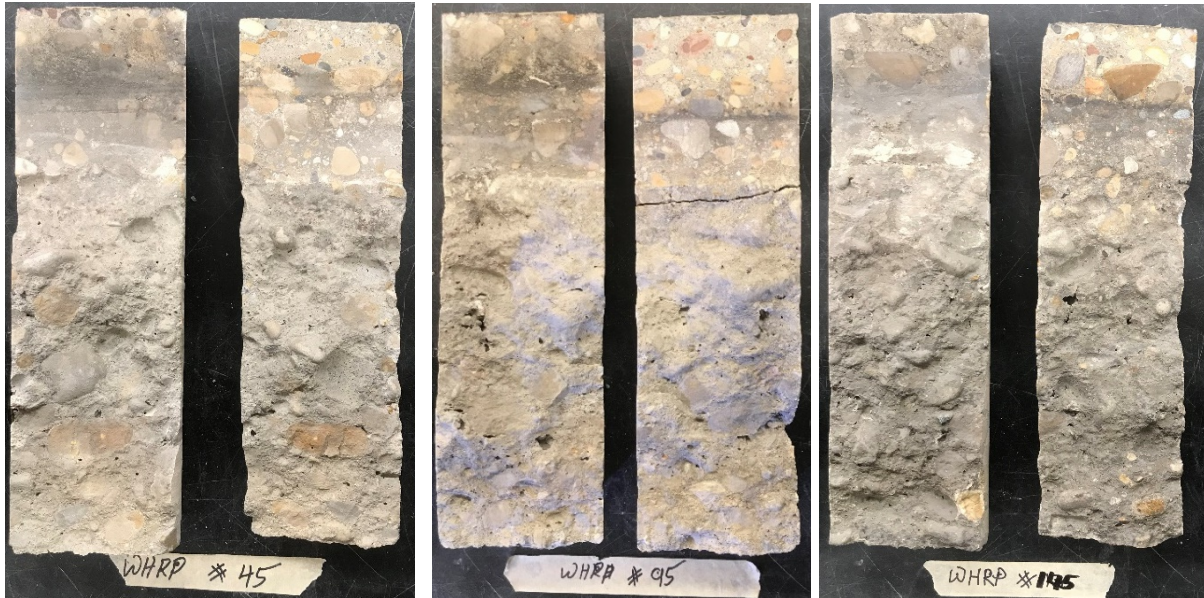
Figure F.1 I-39 Control Core Samples, as-received left, cleaned right
