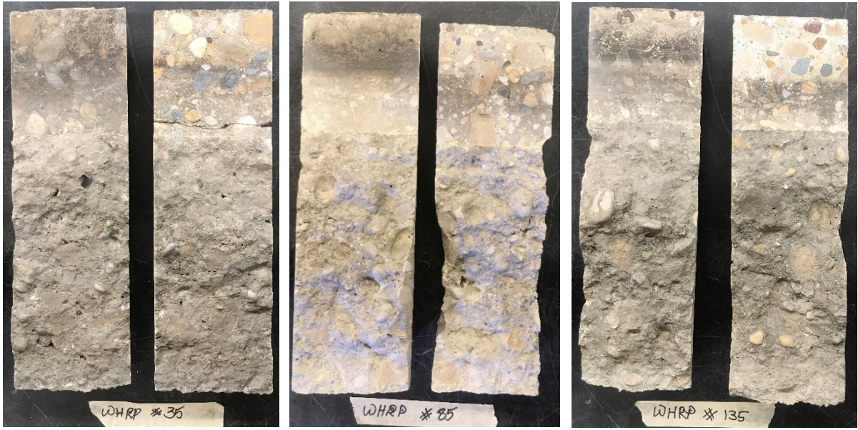
Figure F.5 I-39 Lithium Silicate Mixture-Treated Core Samples, as-received left, cleaned right
