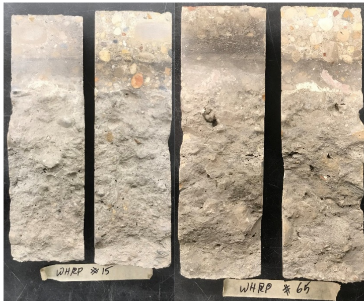
Figure F.3 I-39 Siloxane Mixture-Treated Core Samples, as-received left, cleaned right
