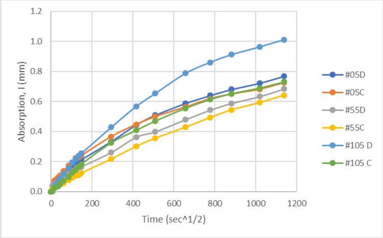
Figure F.8 I-39 Silane-Treated Core Absorption
