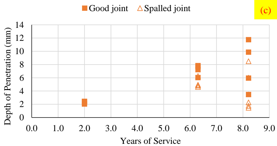
Figure 3.7 Service Life (a) Contact Angle, (b) Absorption, (c) Depth of Penetration
