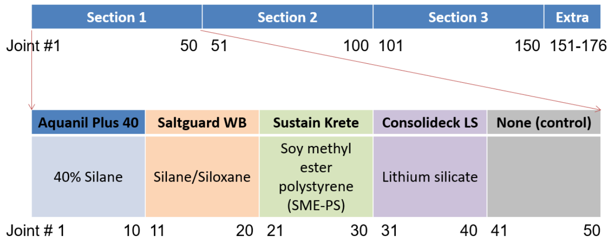
Figure 5.1 Experimental Design of Field Study
