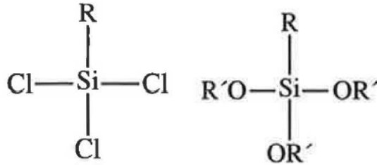
Figure 2.2 (a) chlorosilane (b) silane and siloxane
