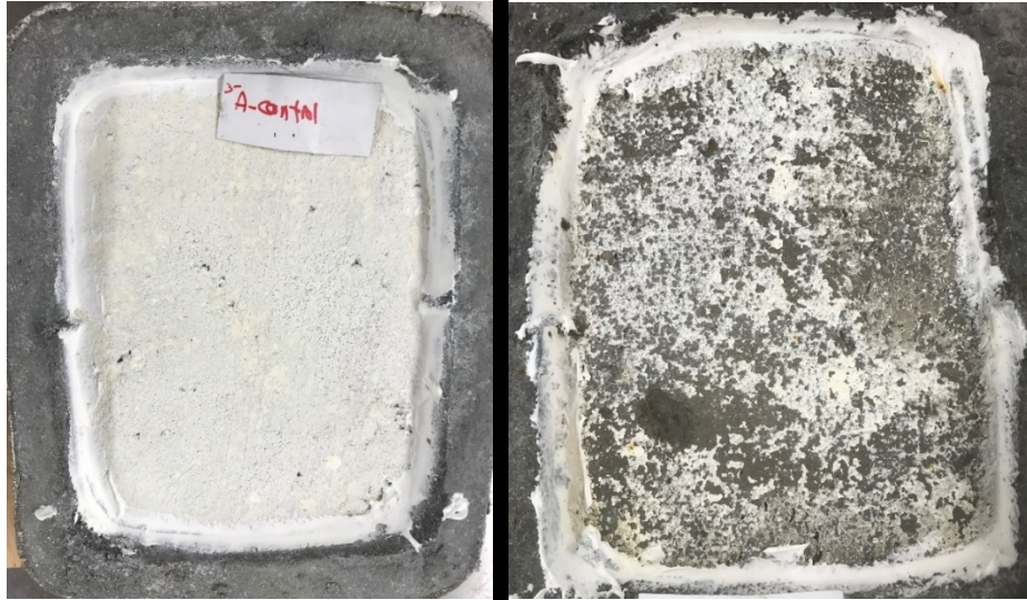
Figure 4.7 “A” Control Deicer Scaling Performance (Left 0 cycles-0, Right 50 cycles-3)
