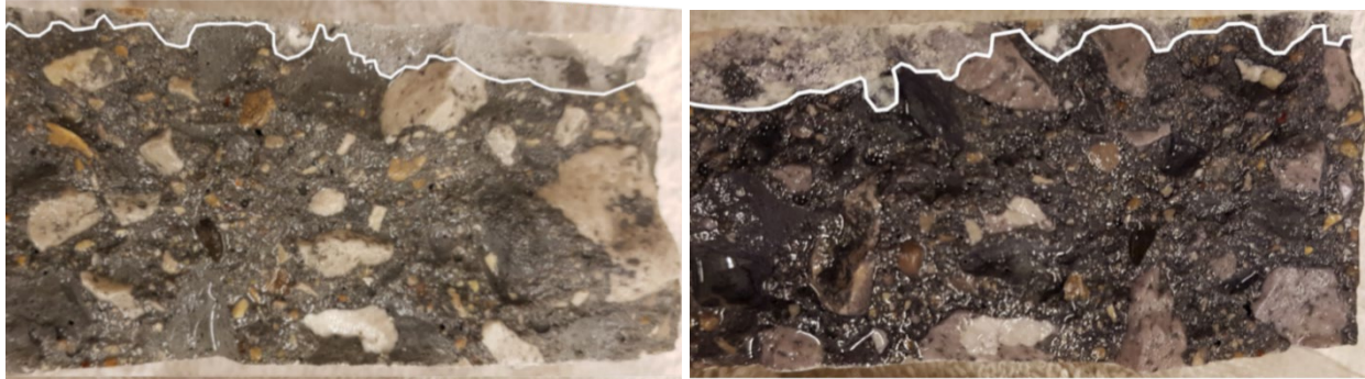
Figure 4.3 Example Depth of Penetration for Silane Treated Specimens (Left: water, Right: blue fabric dye)
