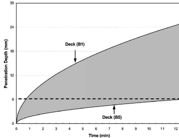
Fig. 4. Silane penetration depth against time
