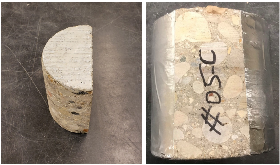
Figure F.6 Preparation of Core Samples for Absorption Testing, epoxy-coating surface (left) and aluminum tape on shoulders and exposed top (right)
