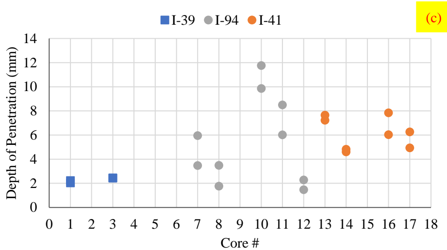
Figure 3.6 Presence of Sealer (a) Contact Angle, (b) Absorption, (c) Depth of Penetration
