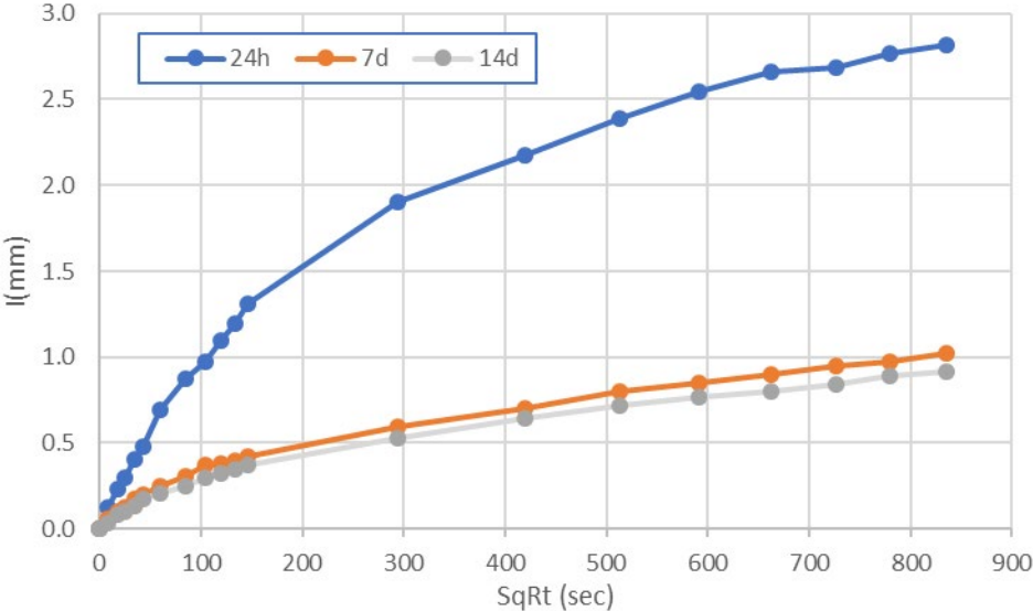
Figure C.1 Phase I Mortar Absorption Results as a Function of Curing Time (Times shown are length of moist curing before the prerequisite 14d drying time required by ASTM C1585 prior to testing)
