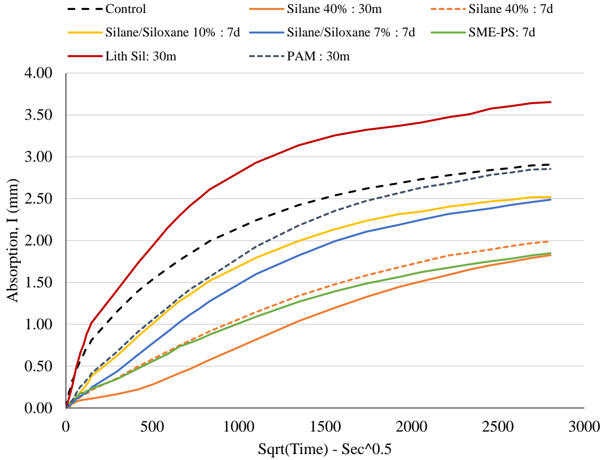
Figure 4.5 Wis "A" Absorption Results
