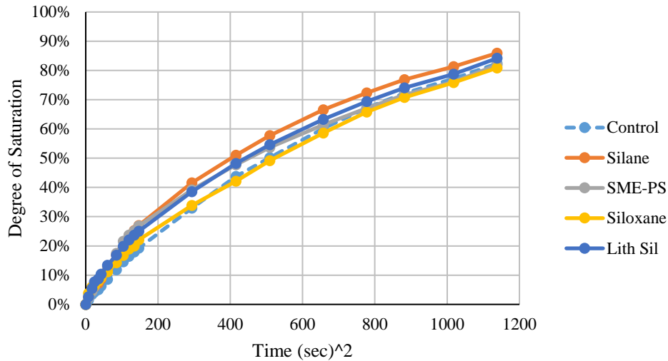
Figure 5.11 Absorption Performance of I-39 Core Samples
