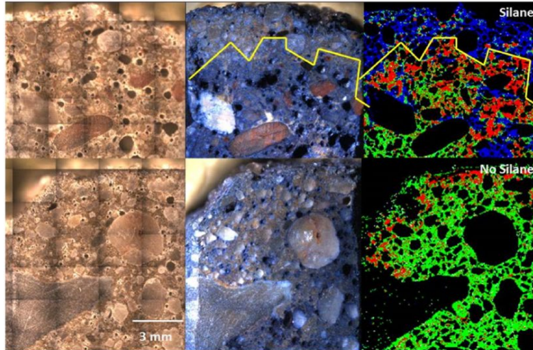
Fig. 9. Example of comparing a sample that contains silane to a sample that does not. (Top left) optical image of sample containing silane (top middle) optical image of sample containing silane stained with dye (top right) cement paste cluster map for sample containing silane (bottom left) optical image of sample not containing silane (bottom middle) optical image of sample not containing silane stained with dye (bottom right) cement paste cluster map for sample not containing silane. Note: The average sulfur concentration level for different colors in paste cluster map is provided in Table 2.
