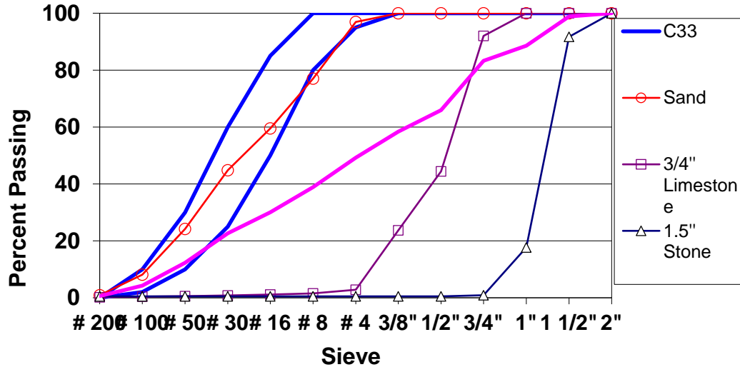
Figure B.1 Aggregate Gradations
