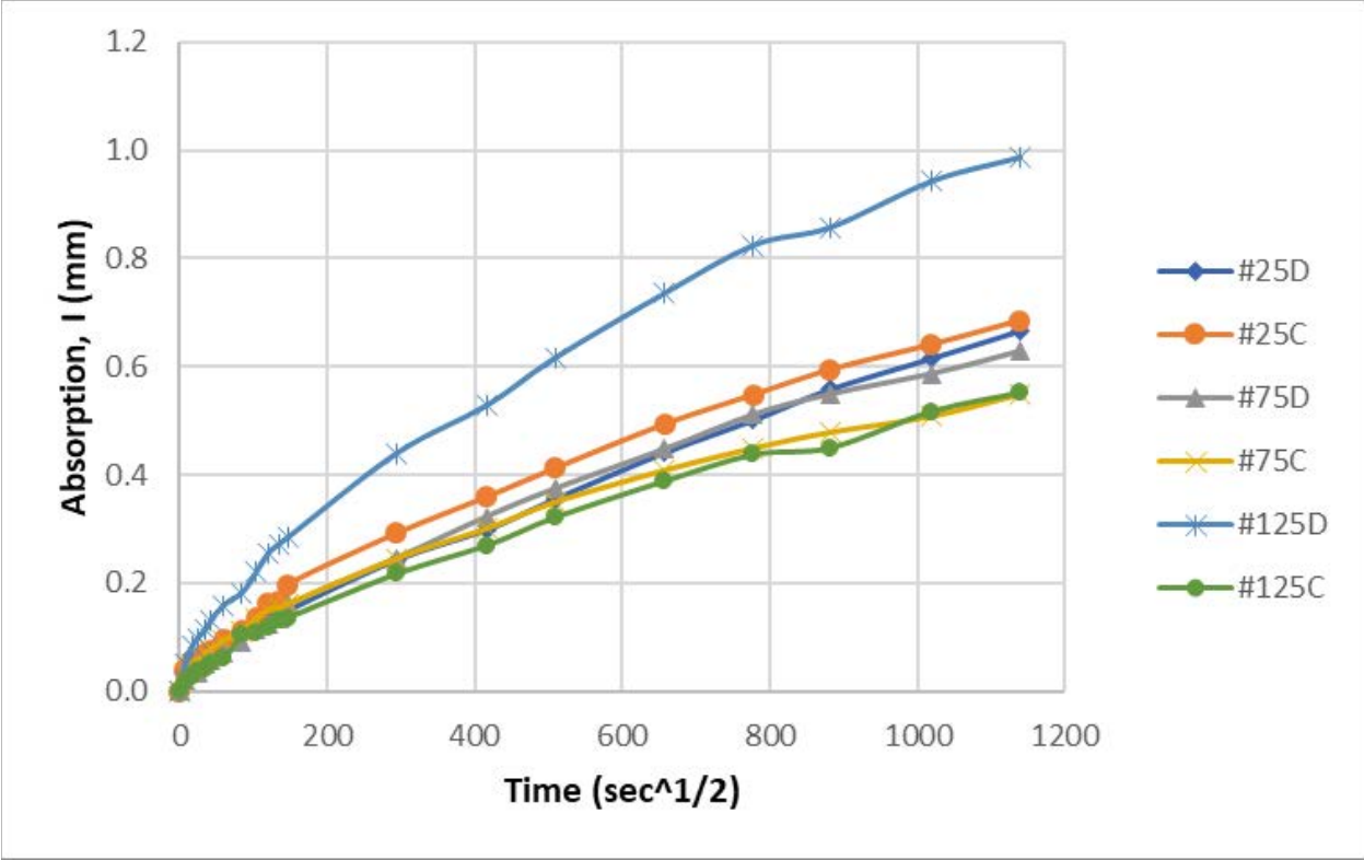
Figure F.9 I-39 SME-PS-Treated Core Absorption
