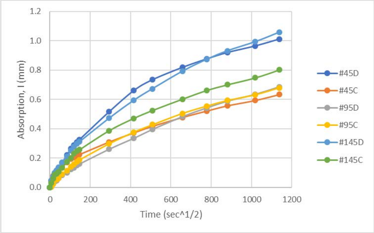
Figure F.7 I-39 Untreated Control Core Absorption
