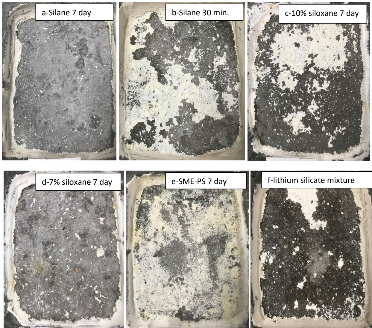
Figure 4.8 Deicer Scaling Performance of Wis “A” Concrete (50 cycles)
