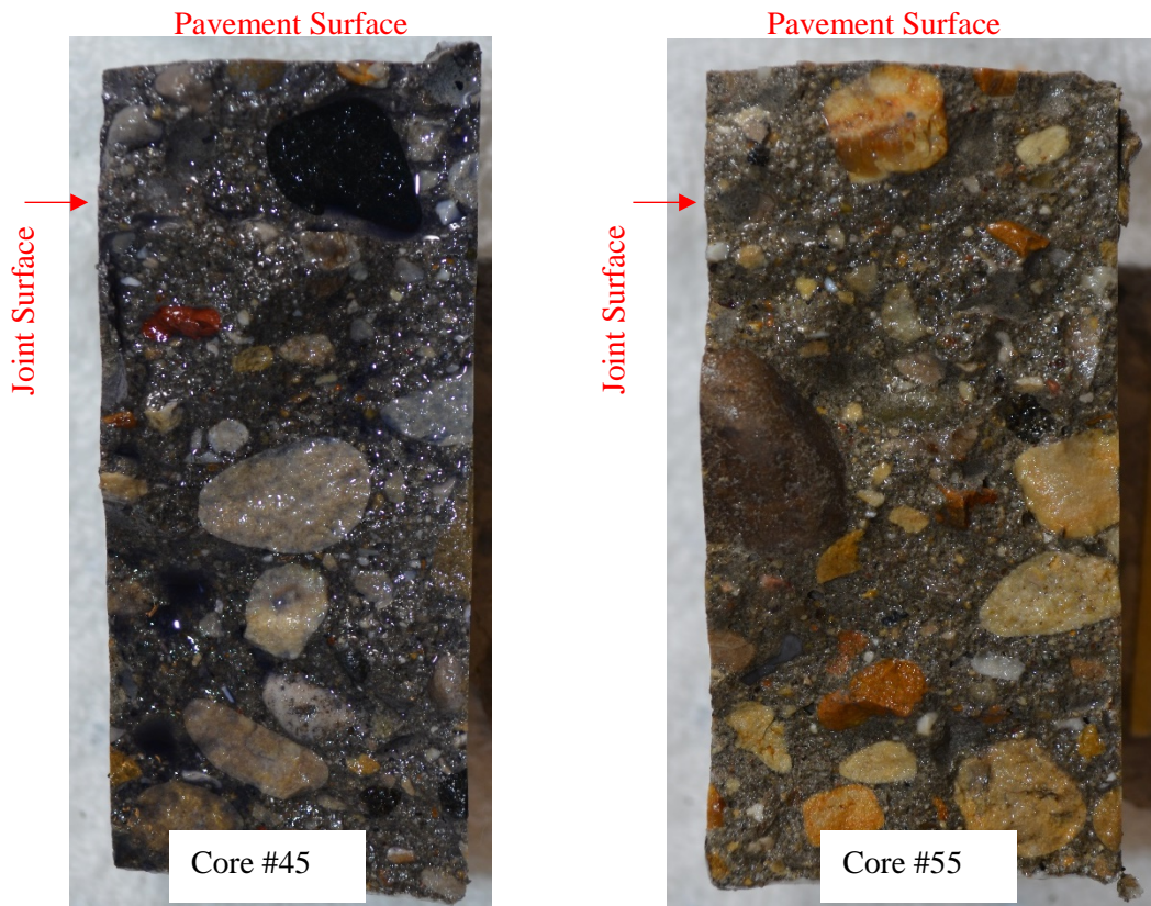
Figure 5.12 Depth of Penetration of Core Samples from I-39
