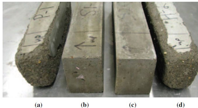
FIGURE 7 Freeze–thaw samples after 280 cycles: (a) plain, (b) SME-PS, Dose 1, (c) SME-PS, Dose 2, and (d) SBS. Untreated (plain) samples and SBS-treated samples show significant cover loss. SME-PS-treated samples show no visual damage.
