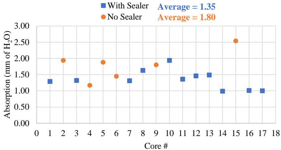
Figure A.3 Absorption of Core Samples from I-94, I-41, and I-39
