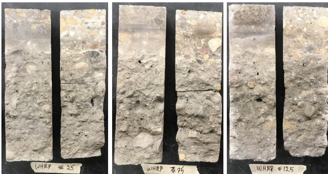
Figure F.4 I-39 SME-PS Treated Core Samples, as-received left, cleaned right
