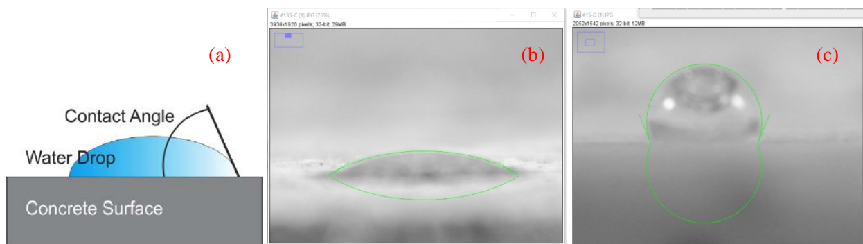
Figure 3.3 (a) Definition of contact angle (b) Contact angle=32.5° for core #135 (c) Contact angle =112.5° for core #15
