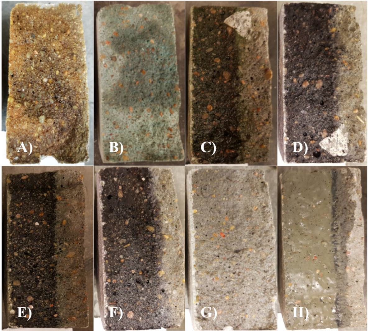
Figure C.2 Preliminary Dye Testing for Depth of Penetration (A) Cola AS, B) Azure Blue AS, C) Green Apple LRD, D) Navy Blue LRD, E) Dark Green PRD, F) Navy Blue PRD, G) Blue FC, H) Antique Gray WB
