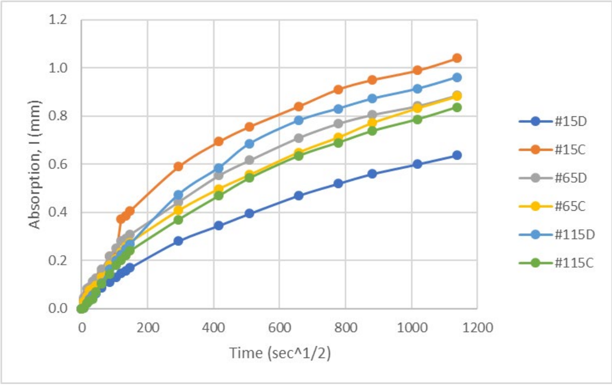
Figure F.10 I-39 Siloxane Mixture-Treated Core Absorption
