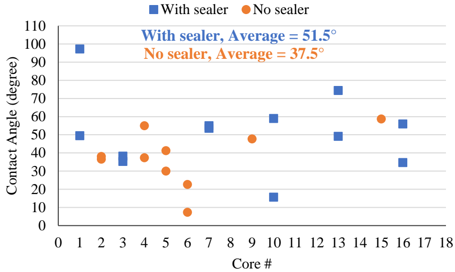
Figure A.2 Contact Angle of Core Samples from I-94, I-41, and I-39
