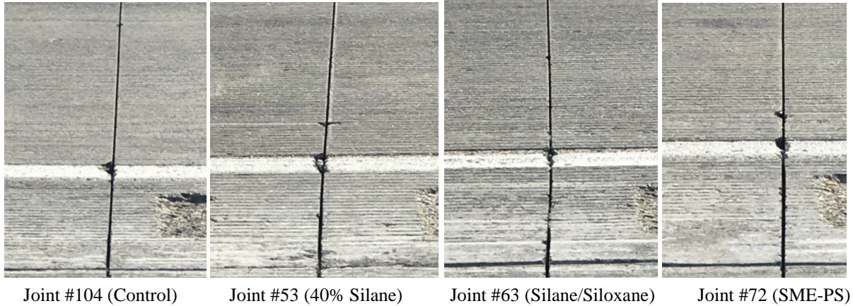
Figure 5.4 Examples of small spalling observed during the August site visit
