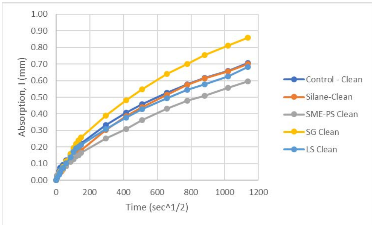
Figure F.11 I-39 Lithium Silicate Mixture-Treated Core Absorption
