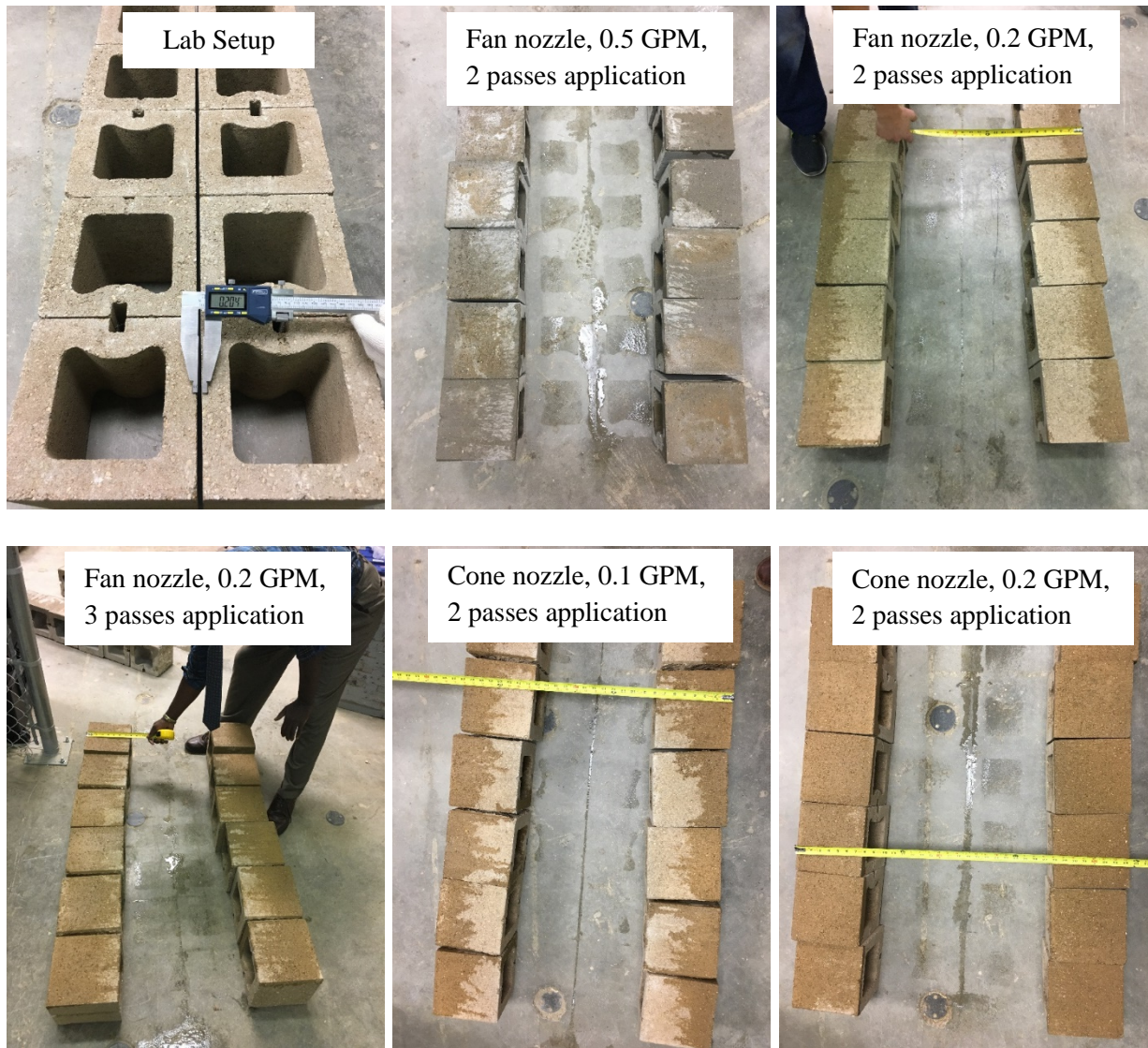
Figure 4.9 Coverage of Joint Face using Different Types of Nozzle and Opening Size
