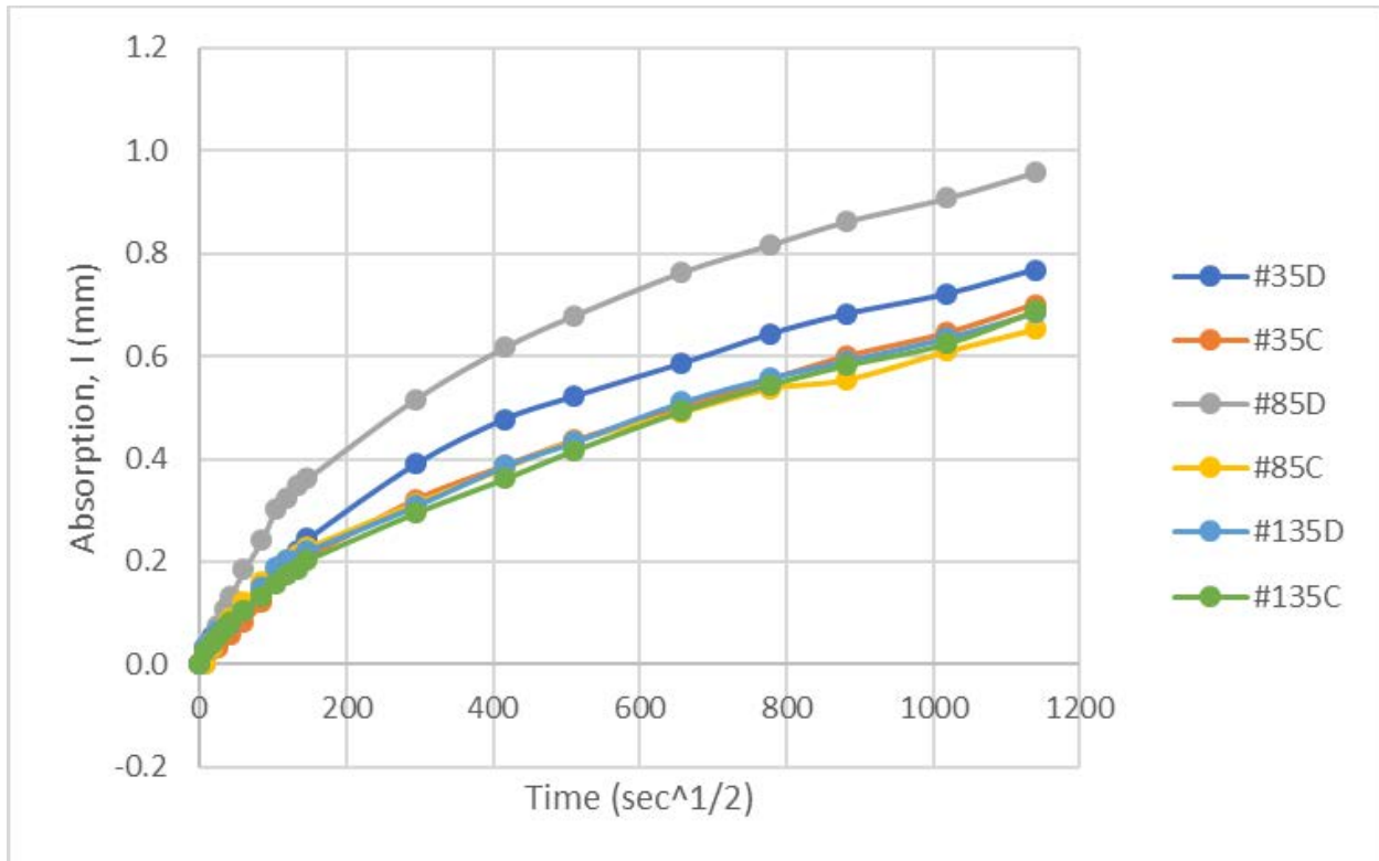
Figure F.11 I-39 Lithium Silicate Mixture-Treated Core Absorption
