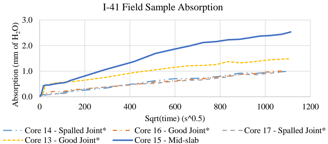
Figure A.1 Absorption of Core Samples from I-94, I-41, and I-39
