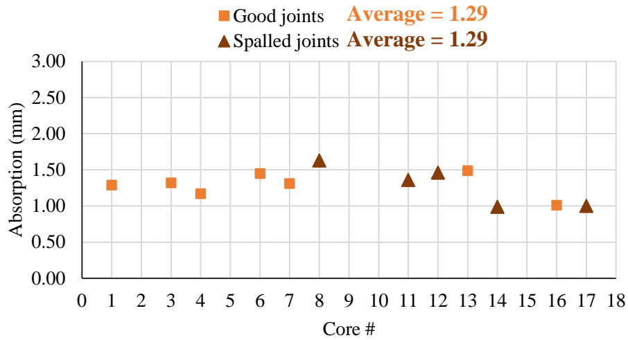
Figure A.5 Absorption of Good Joints and Spalled Joints from I-94, I-41, and I-39
