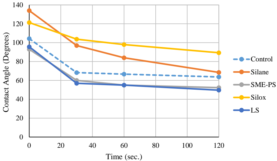
Figure 5.10 Change in Contact Angle with Time for the Cleaned Core Samples
