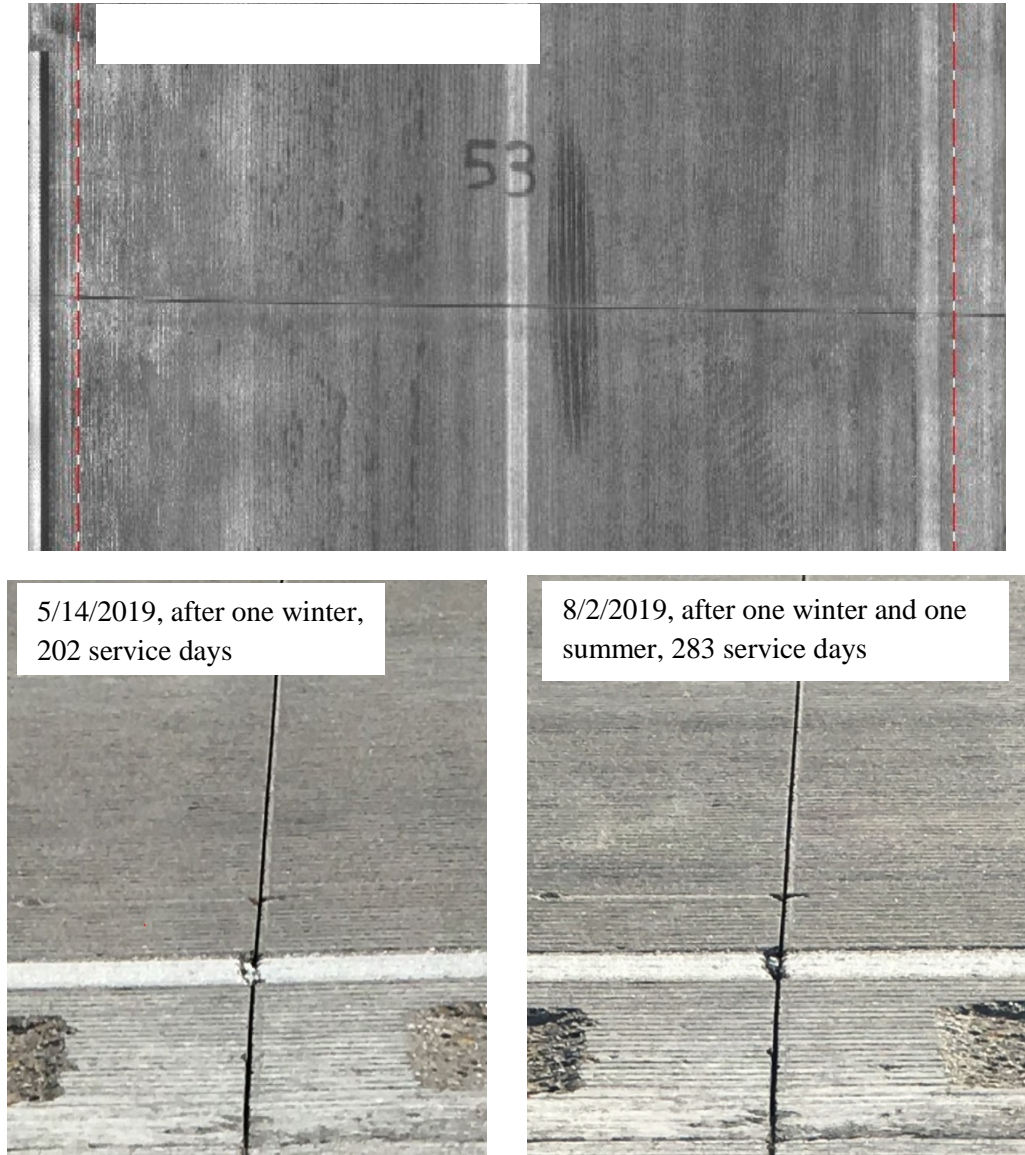
Figure 5.3 Field Performance of Joint #53
