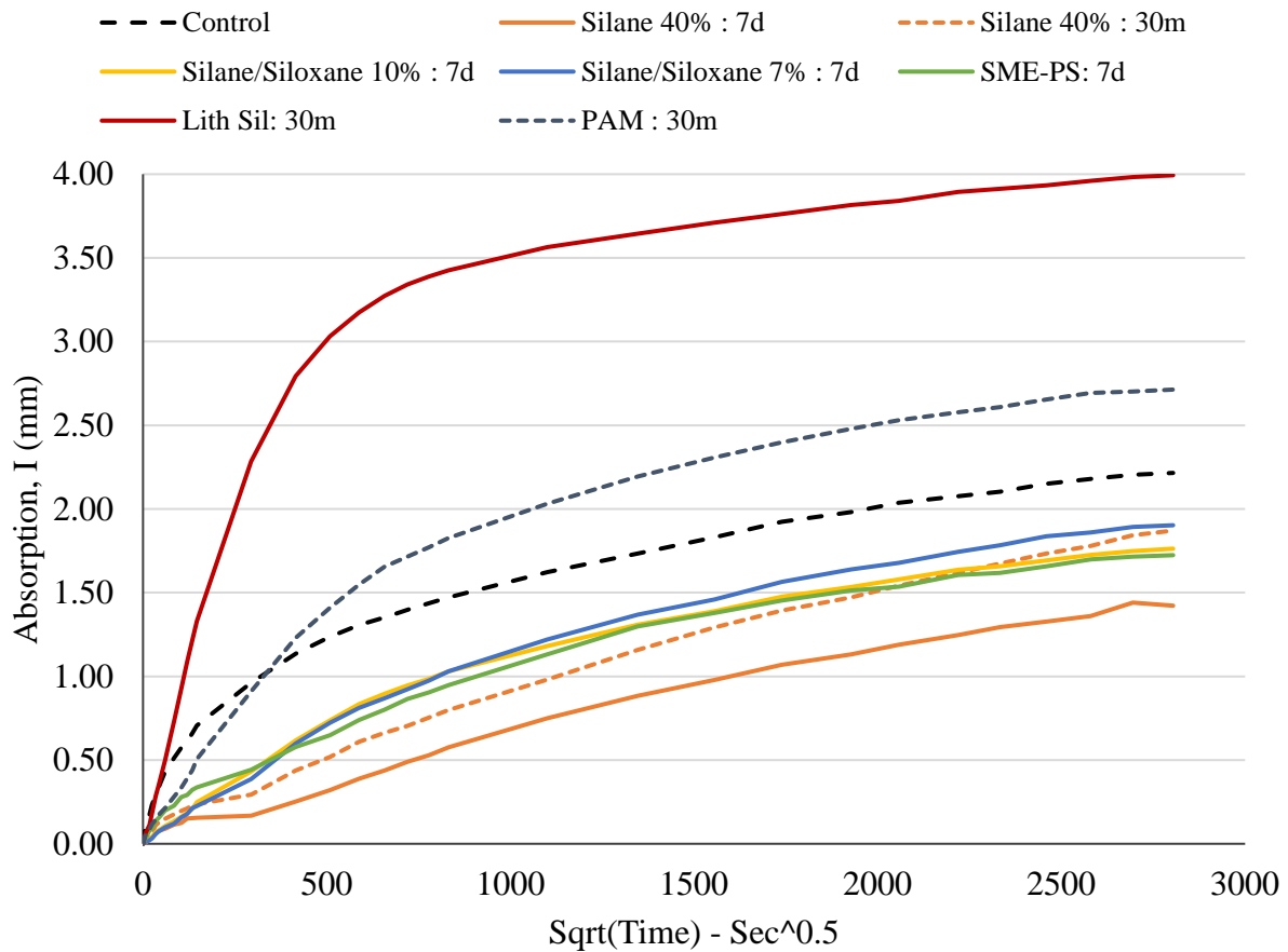
Figure 4.6 Wis “FA” Absorption Results
