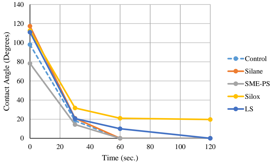
Figure 5.9 Change in Contact Angle with Time for the As-Received (Dirty) Core Samples
