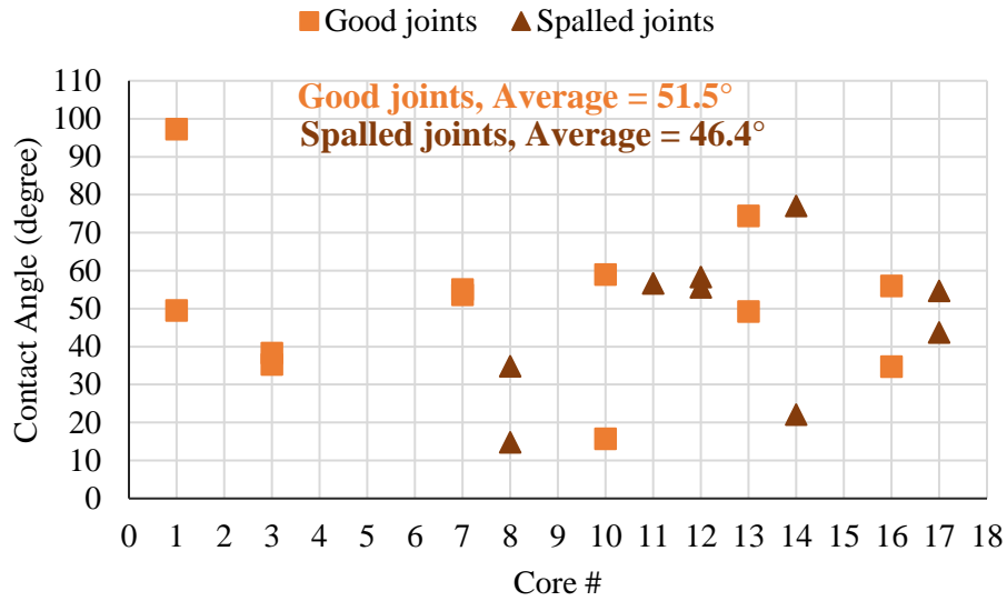
Figure A.4 Contact Angle of Good Joints and Spalled Joints from I-94, I-41, and I-39
