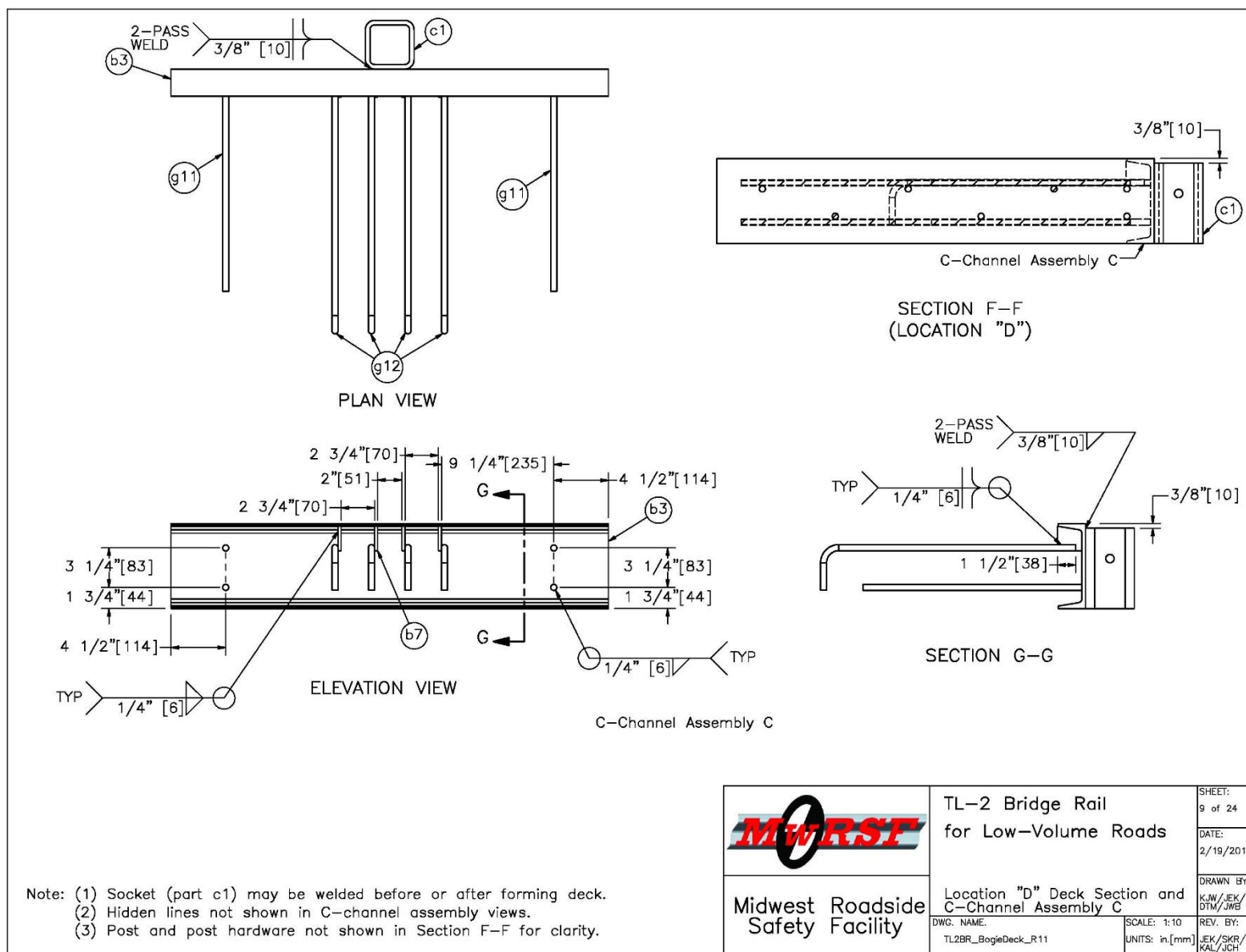
Figure 20. Bogie Testing Matrix and Setup, Location "D" Deck Section and C-Channel Assembly C
