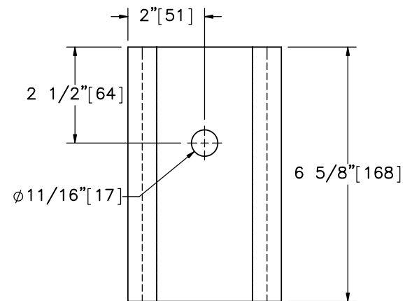
PROFILE VIEW
