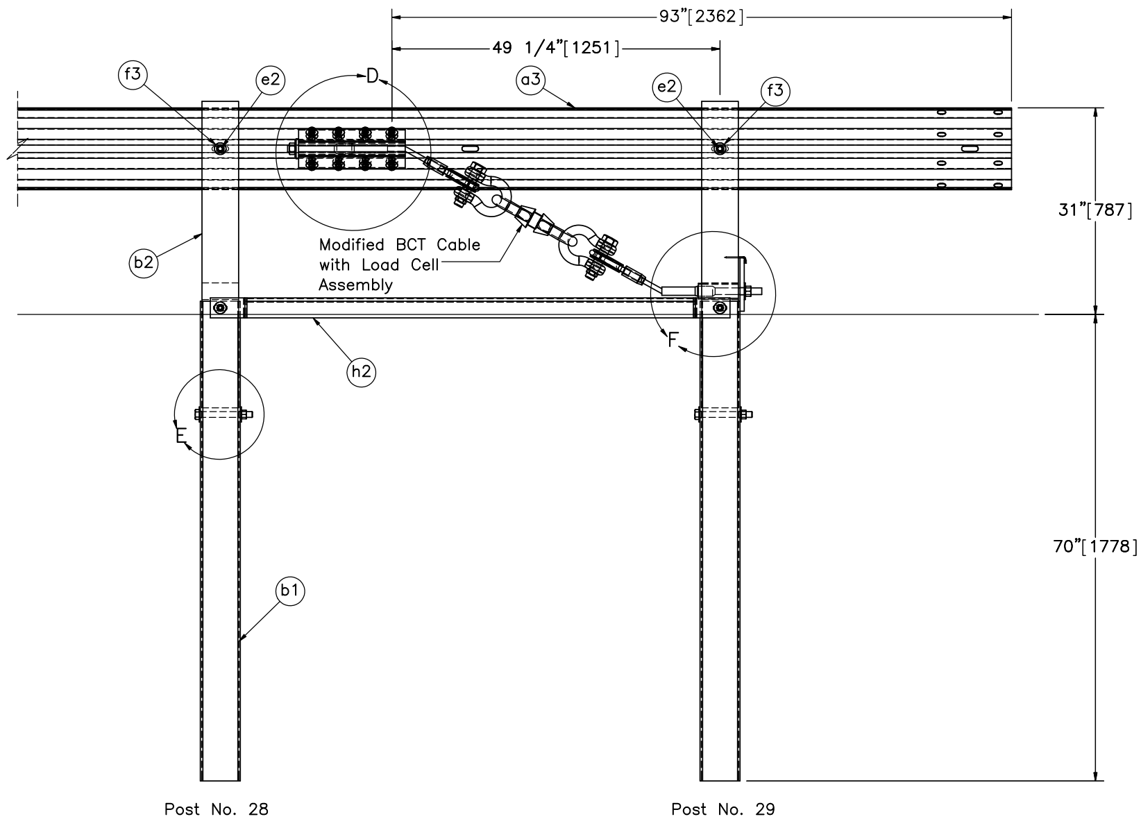
END SECTION DETAIL BACKSIDE (TYP)
