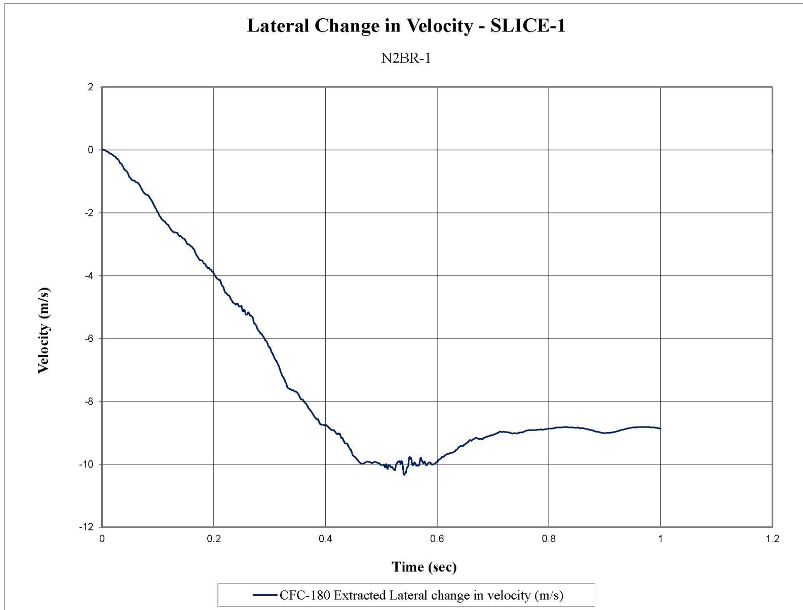
Figure G-5. Lateral Change in Velocity (SLICE-1), Test No. N2BR-1
