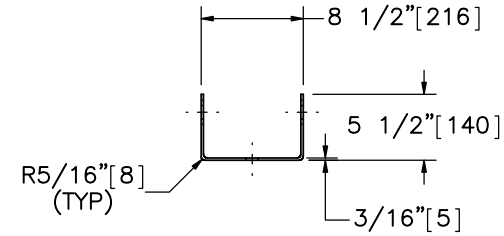
PLAN VIEW
