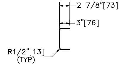
PROFILE VIEW
