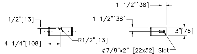
ELEVATION VIEW
