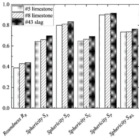
Figure 4.19 Results of morphology analyses of test aggregates using the MATLAB code for particles: (a) passing the 25 mm sieve and retained in the 19 mm sieve and (b) passing the 19 mm sieve and retained in the 12.5 mm sieve.
