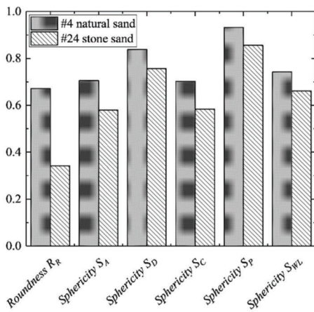
Figure 4.21 Results of morphology analyses of test sands using the MATLAB code for particles: (a) passing the 4.75 mm sieve and retained in the 2.36 mm sieve and (b) passing the 2.36 mm sieve and retained in the 1.18 mm sieve.
