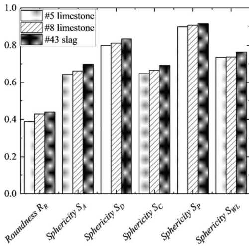
Figure 4.20 Results of morphology analyses of test aggregates using the MATLAB code for particles: (a) passing the 12.5 mm sieve and retained in the 9.5 mm sieve and (b) passing the 9.5 mm sieve and retained in the 4.75 mm sieve.
