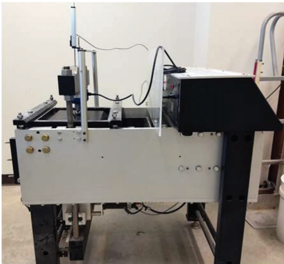
Figure 6.2 Large-scale direct shear machine manufactured by GeoComp.
