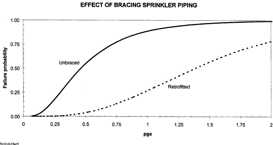
Figure 3-3 - Comparison of mean AS system fragility, with and without bracing
