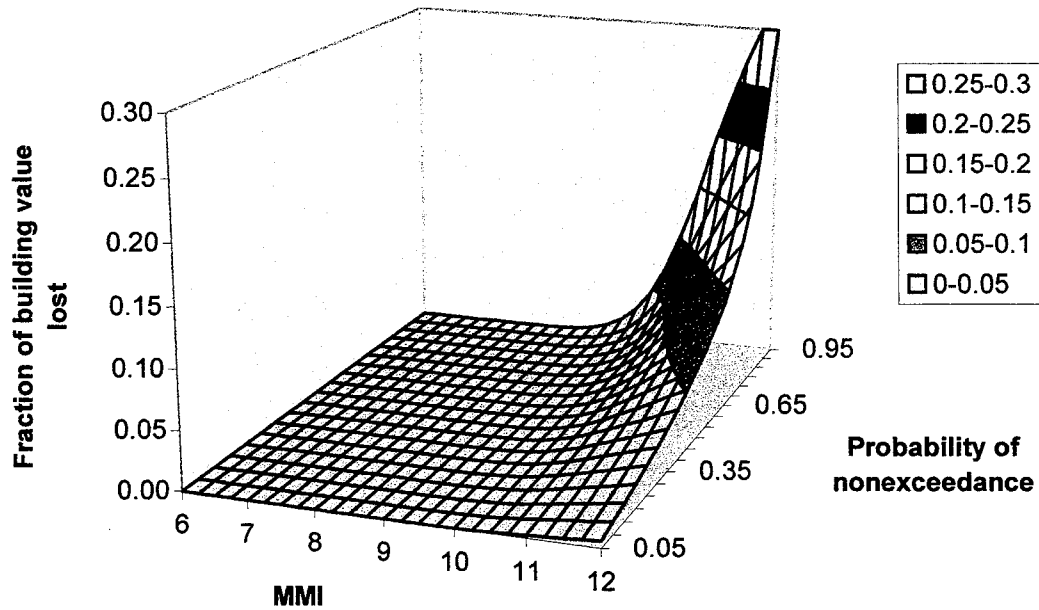
Figure 3-4 - Property vulnerability under unbraced conditions
