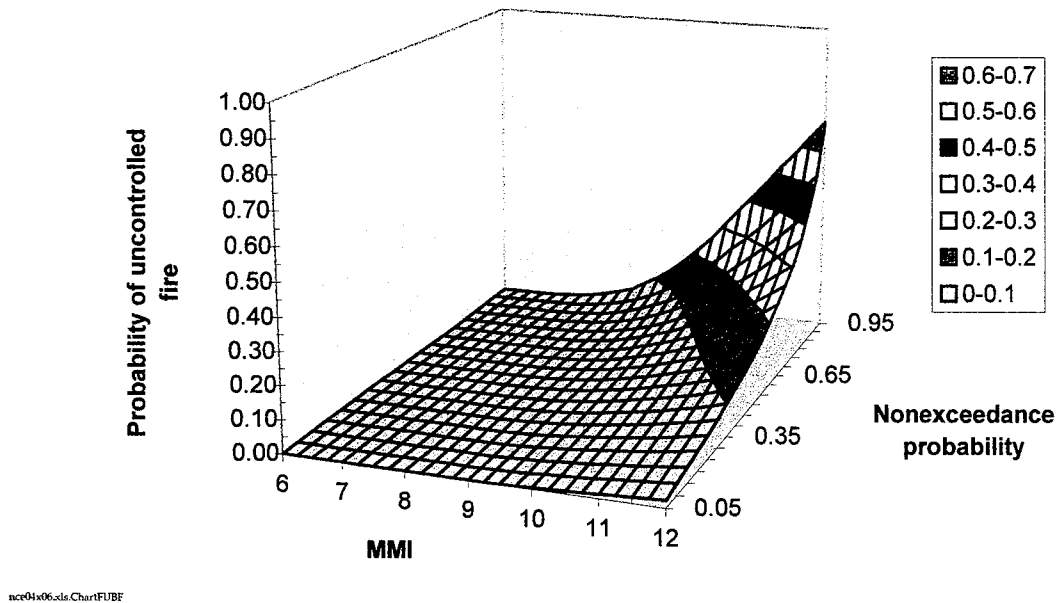
Figure 3-2 - Probability of uncontrolled building fire, unbraced conditions
