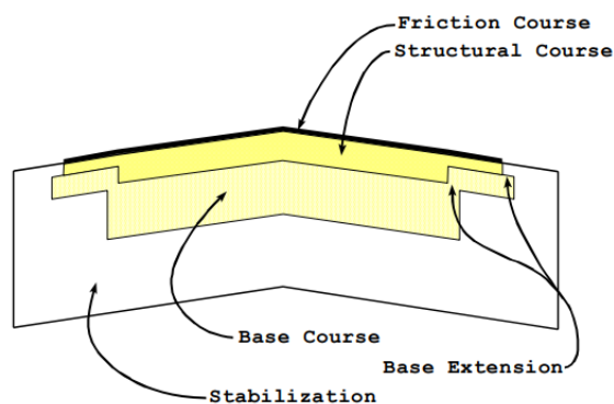
Figure 10-2. Roadway typical section.
