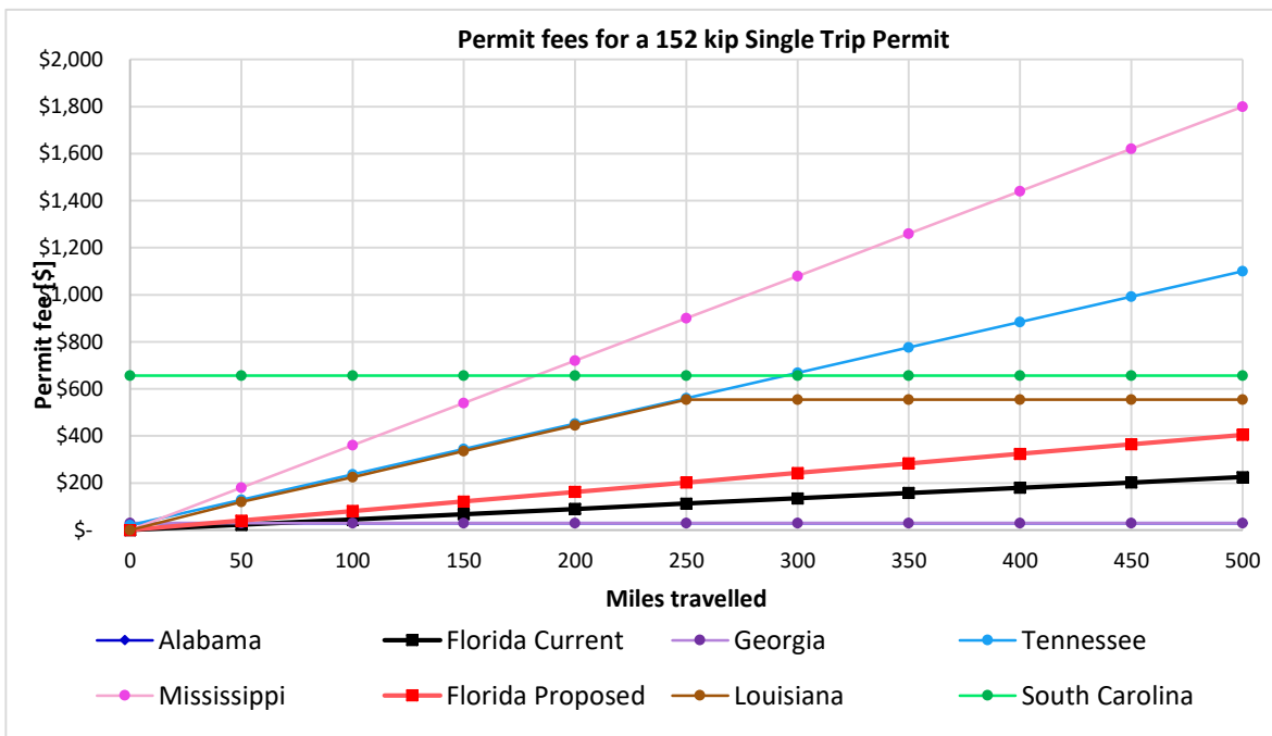
Figure 18-1. Comparative analysis of permit fees within states for single trip permits for the following GVW groups (e) up to 142 kip, (f) up to 152 kip, (g) up to 162 kip, (h) up to 199 kip, (i) above 199 kip (continued).
