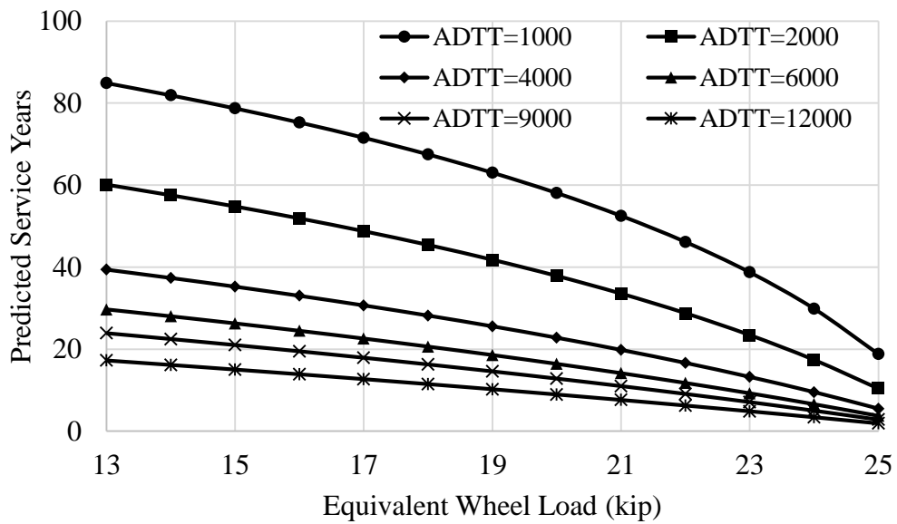
Figure 2-8. The predicted service life of deck under given wheel load and ADTT.
