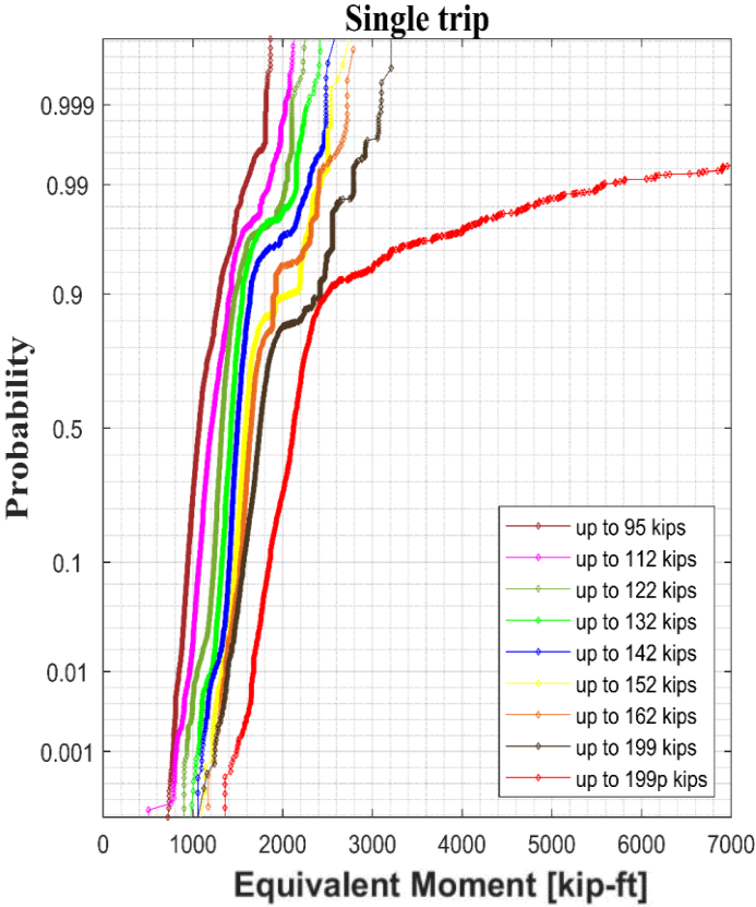
Figure 6-1. Equivalent moment distribution for a single trip.
