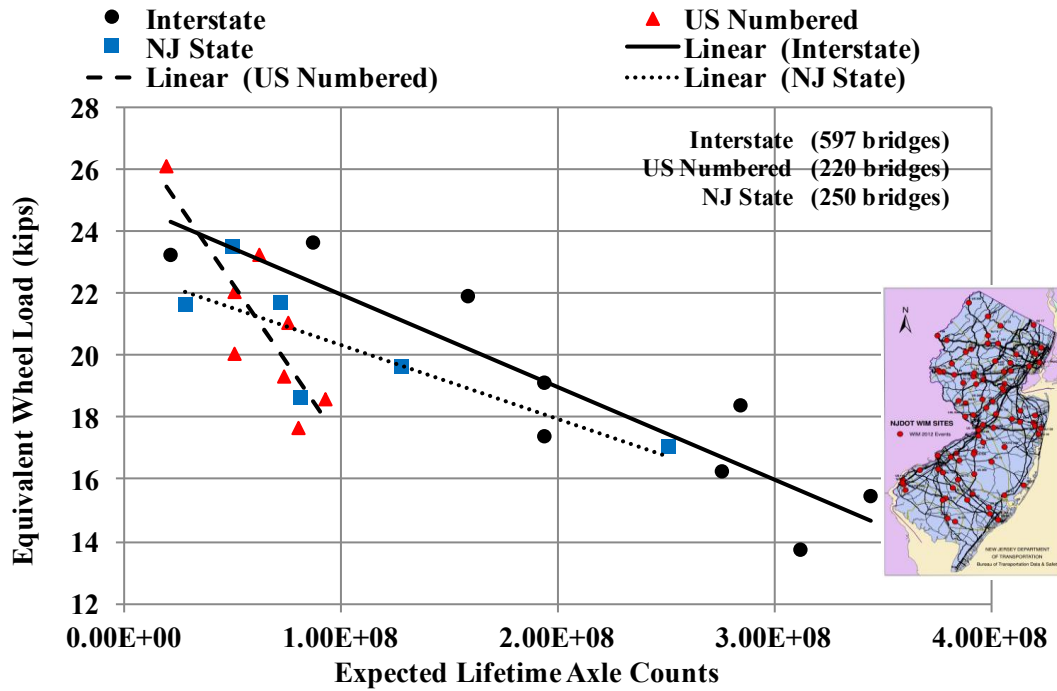
Figure 2-7. Correlation between wheel load and expected lifetime axle counts.
