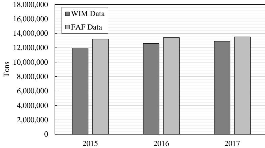
Figure 8.6: WIM and FAF comparison by year at Ashland (NB) and Klamath Falls (NB) WIM stations under assumption 1
