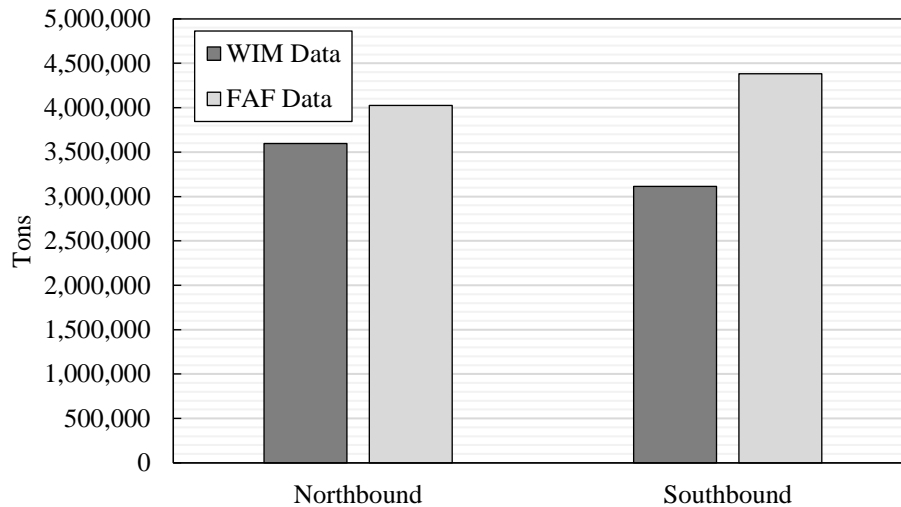
Figure 8.3: WIM and FAF weight comparison at Ashland and Klamath Falls WIM stations in 2012 under assumption 1
