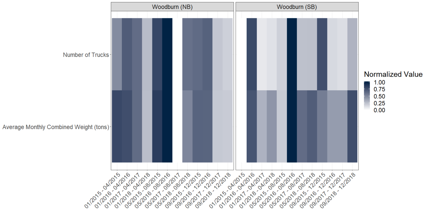
Figure 7.4: Volume and average monthly combined weight seasonal trends for (a) ODOT Class 12 to ODOT Class 19 and (b) ODOT Class 03 to ODOT Class 19 trucks at Woodburn WIM stations
