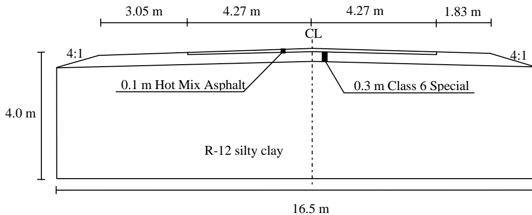
Figure 4 Pavement geometry and dimensions for Cells 33, 34, and 35 [22]
