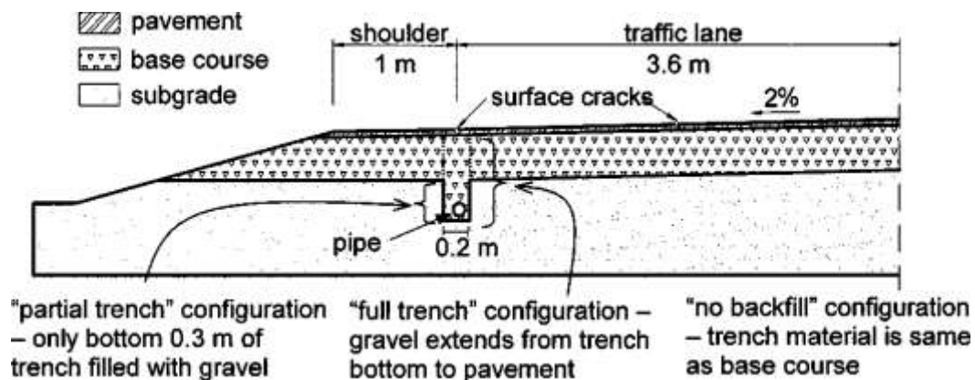
Figure 2 Configuration of modeled pavement section [21]
