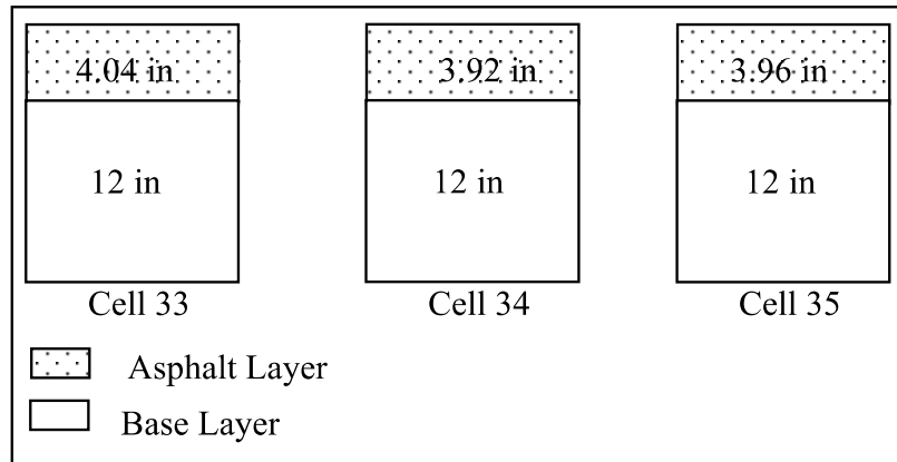
Figure 3 Thickness of base and hot mix asphalt layers for Mn/ROAD Cells 33-35 [22]
