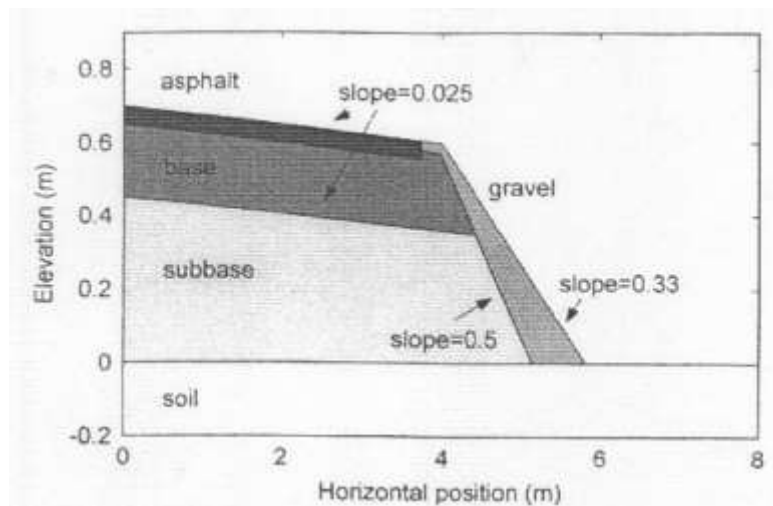
Figure 5 Cross-section of the modeled pavement section [27]
