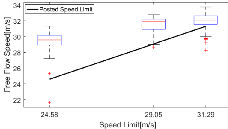
Fig. 8 Free Flow Speed vs. Posted Speed Limit for Highways
