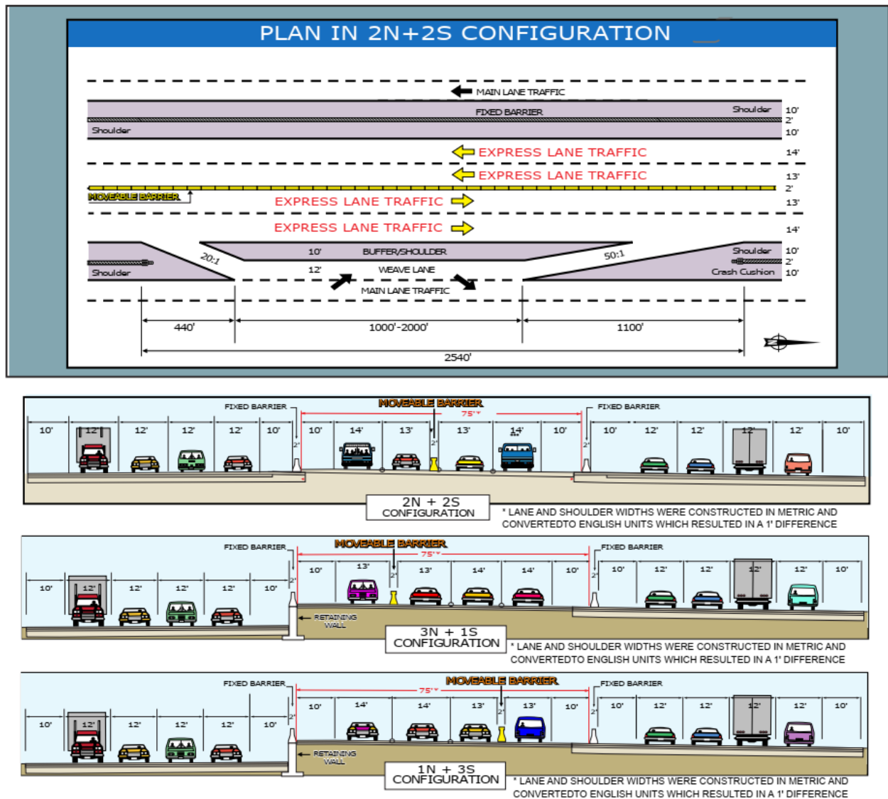
Figure 7. I-15 Express lanes existing 4-lane configurations [plans courtesy of Caltrans].
