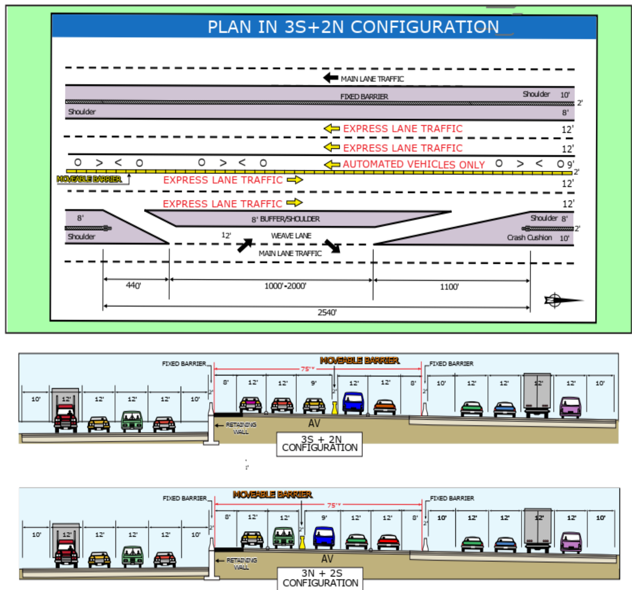
Figure 8. I-15 Express lanes configuration with reversible AV lane [plans courtesy of Caltrans].
