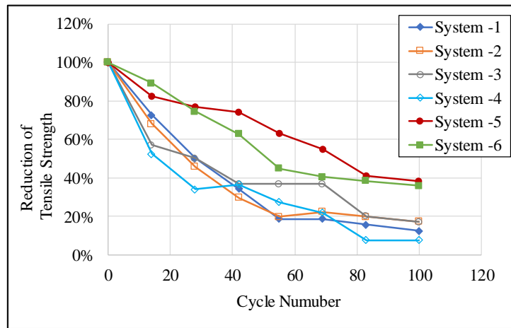
Figure 8 – Tensile strength percentage reduction versus exposure cycle, Balaguru et al. (2018)
