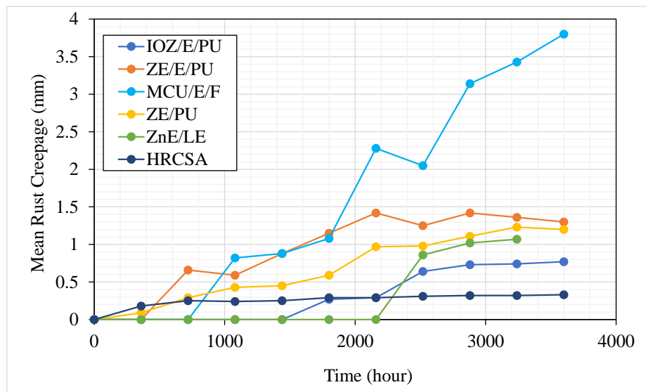
Figure 7 – Mean creepage value versus ALT time. (reproduced from Kodumuri and Lee, 2012)
