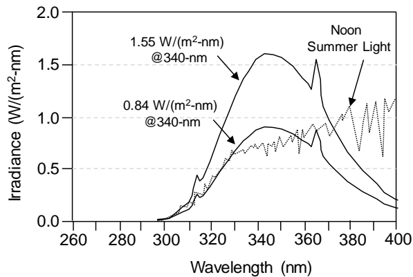
Figure 10 – Comparison of spectral power distribution between noon summer sunlight and UVA-340 lamps at two intensities. (Fedor and Brennan, 1994)
