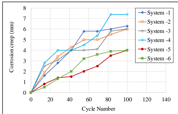
Figure 9 – Corrosion creep growth versus exposure cycle, Balaguru et al. (2018)
