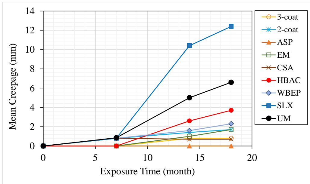
Figure 6 – Mean creepage value versus outdoor exposure time at McLean, Virginia, site. (reproduced from Yao et al., 2011)
