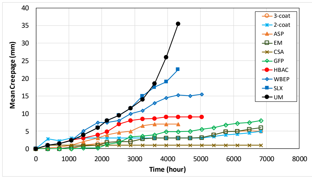
Figure 5 – Mean creepage versus exposure time in an accelerated laboratory test according to ASTM D5894 (replotted from Yao et al., 2011)
