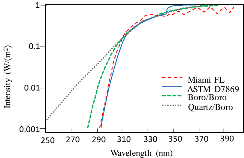
Figure 12 – The spectral power distribution of xenon lamp with different types of filters together with the noon-time sunlight in Miami, Florida. (replotted from Berry et al., 2018)
