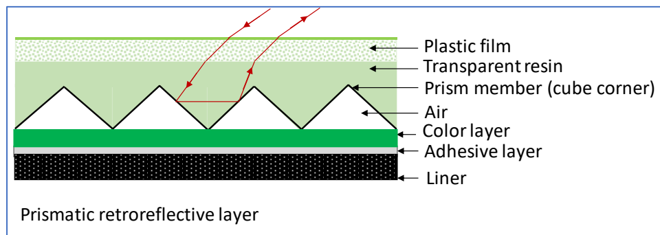
Figure 11 – A schematic of a retroreflective cube corner sheet
