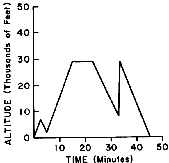
Figure 1. FAA Altitude Chamber Profile Type A.
