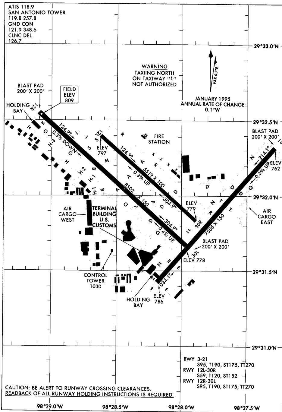
AIRPORT DIAGRAM 97030
