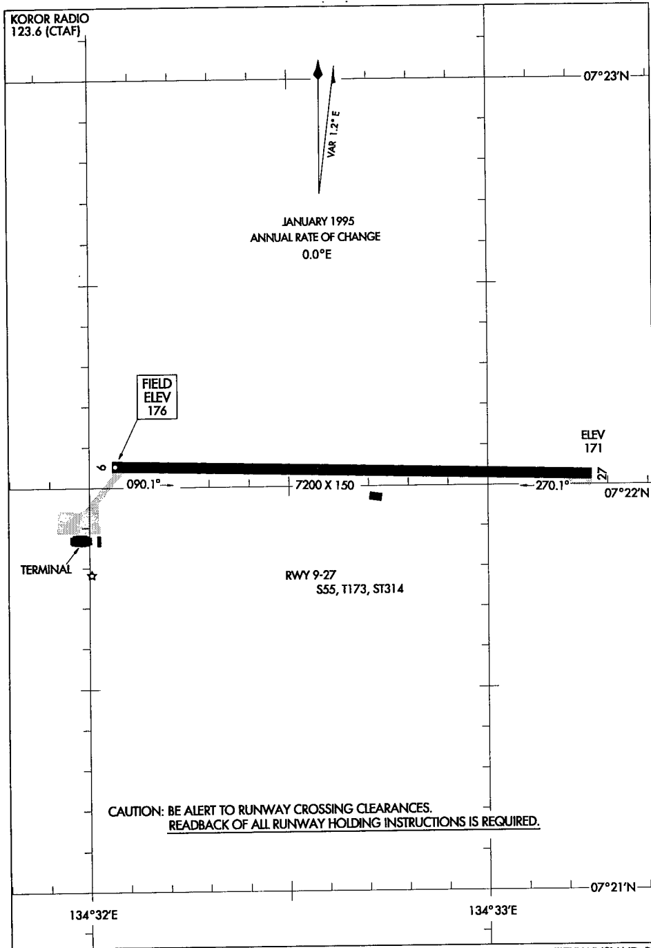
AIRPORT DIAGRAM 97254
