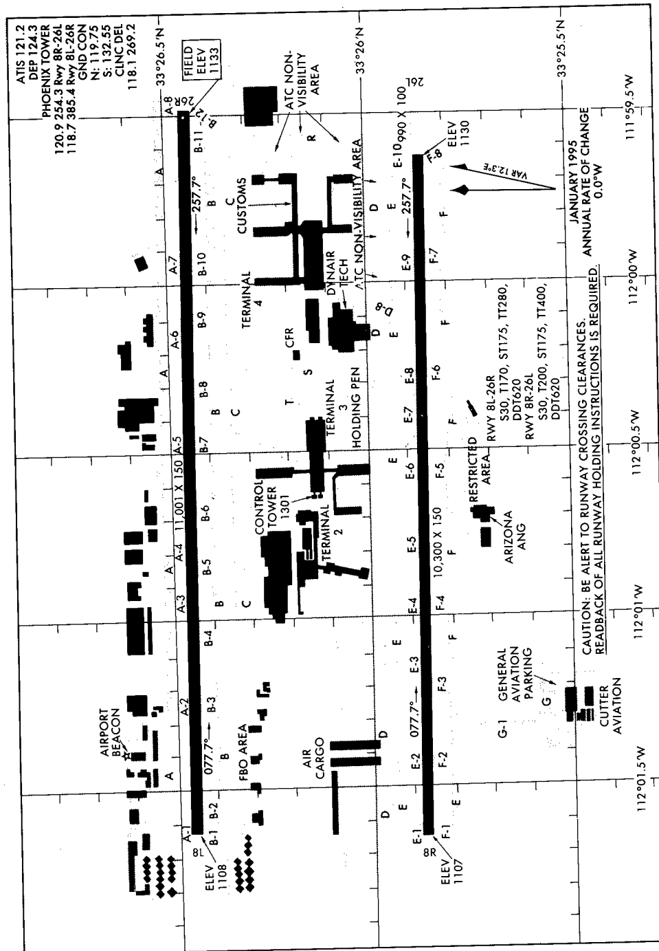
AIRPORT DIAGRAM 97142
