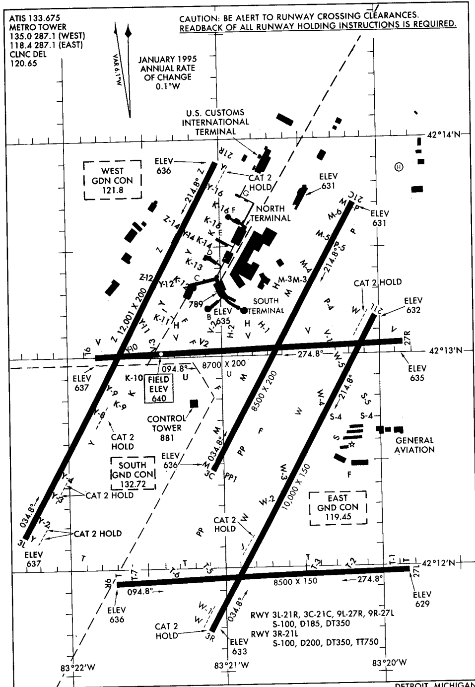
AIRPORT DIAGRAM 97030
