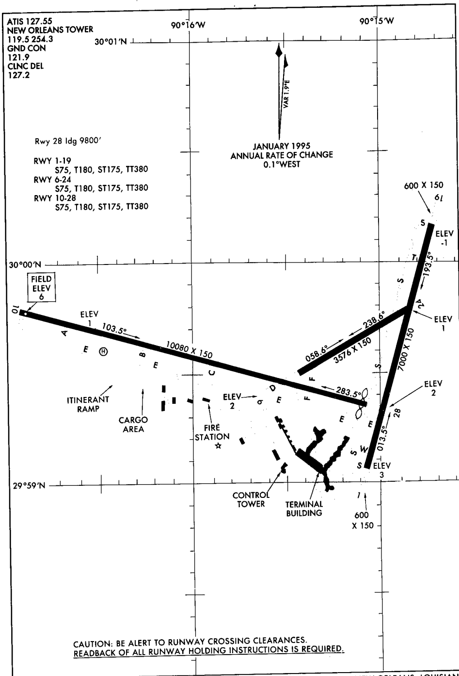
AIRPORT DIAGRAM 97030
