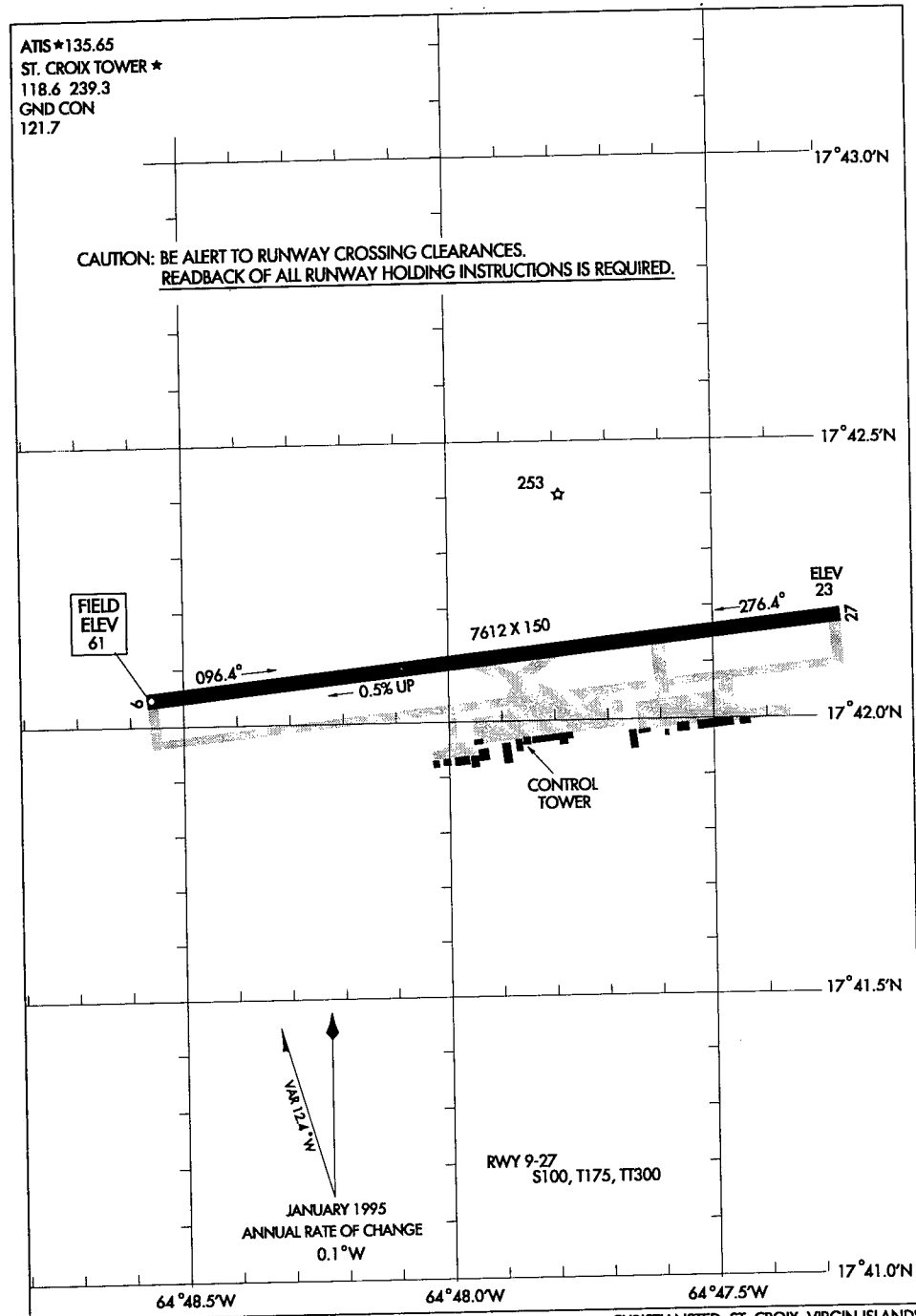
AIRPORT DIAGRAM 97254
