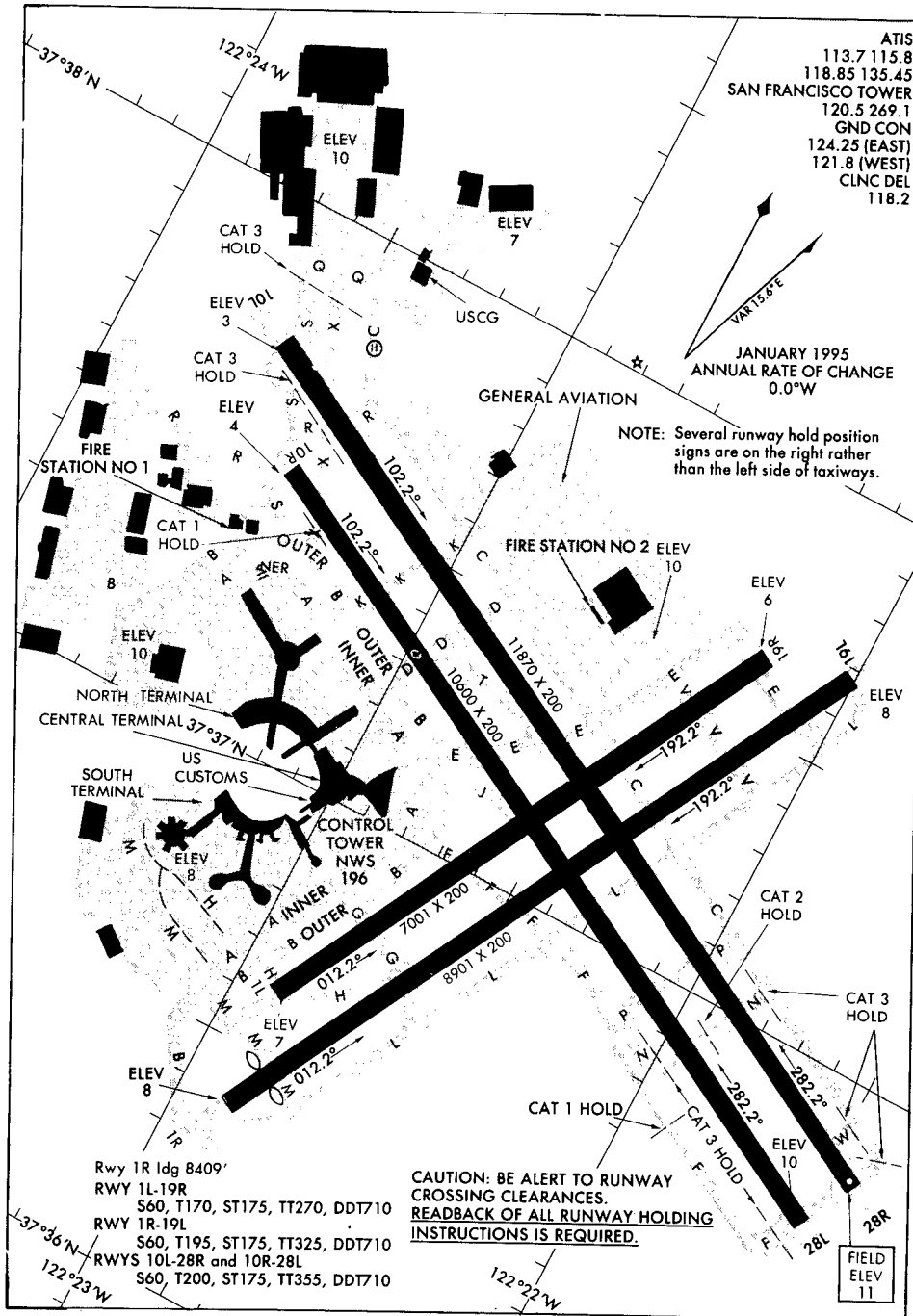
AIRPORT DIAGRAM 97254
