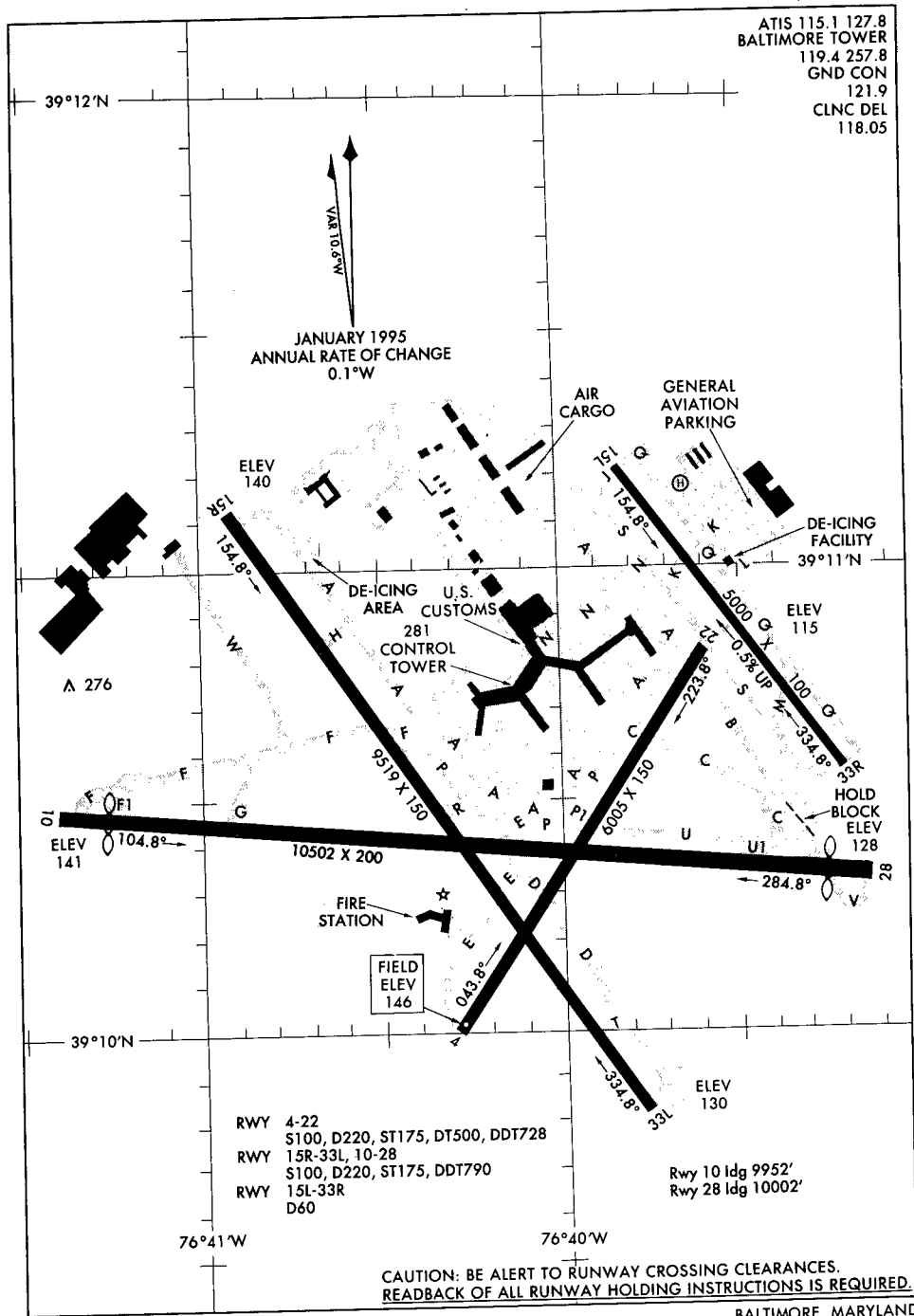
AIRPORT DIAGRAM 98057
