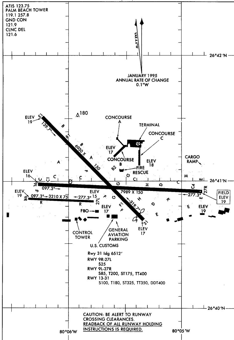
AIRPORT DIAGRAM 98281
