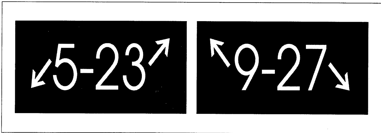
Holding Position Sign for a Taxiway that Intersects the Intersection of Two Runways
