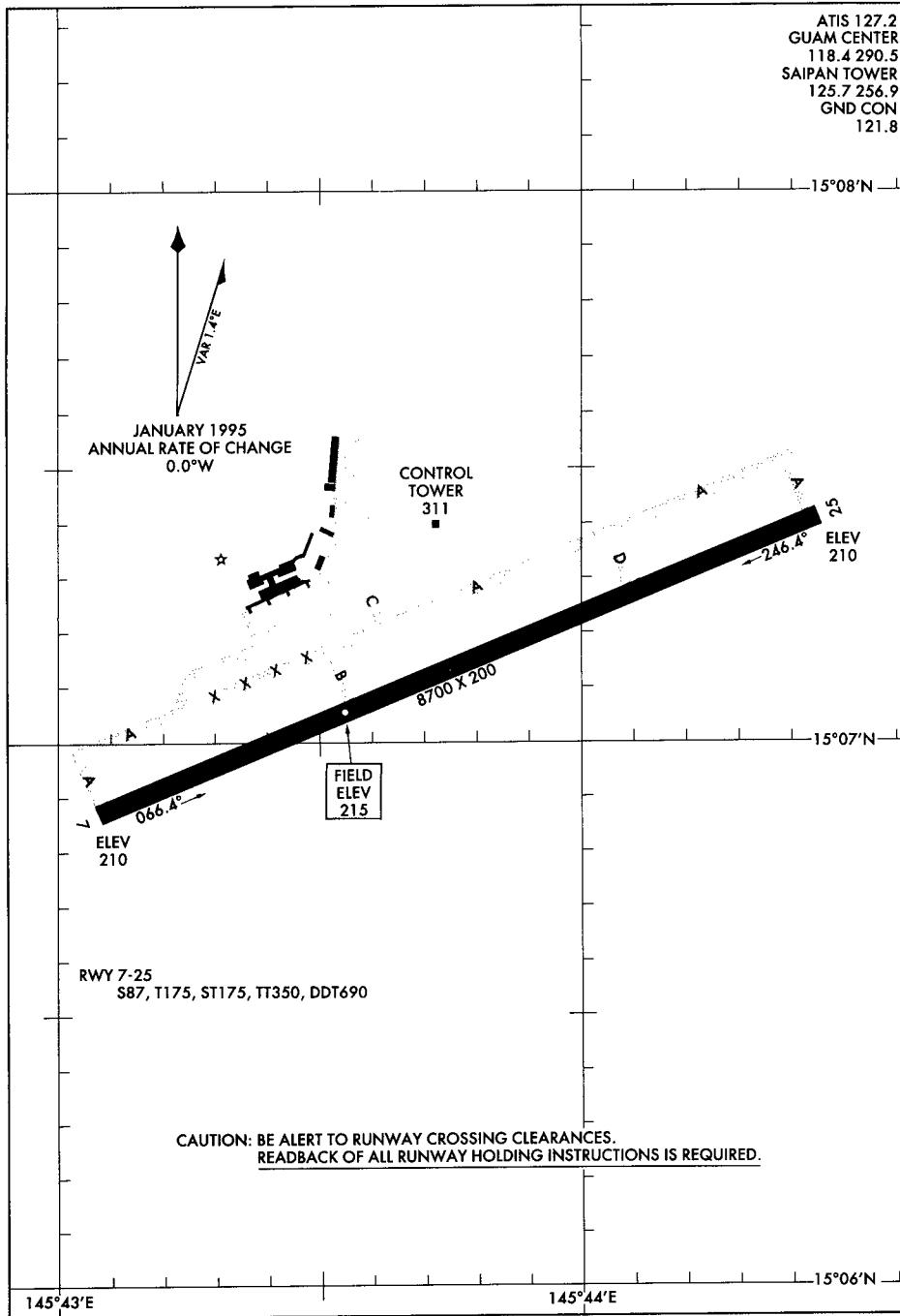
AIRPORT DIAGRAM 98169
