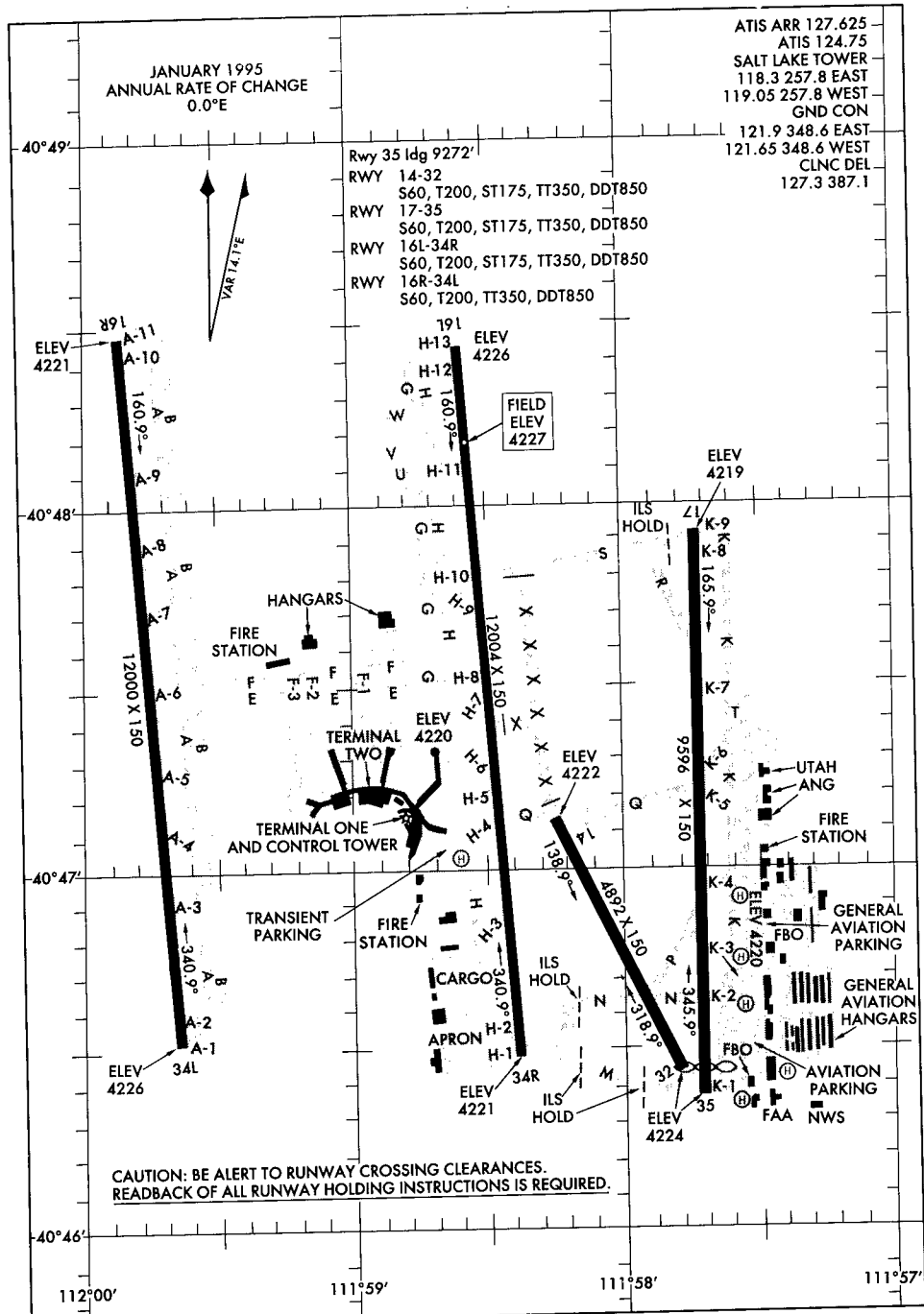
AIRPORT DIAGRAM 98057
