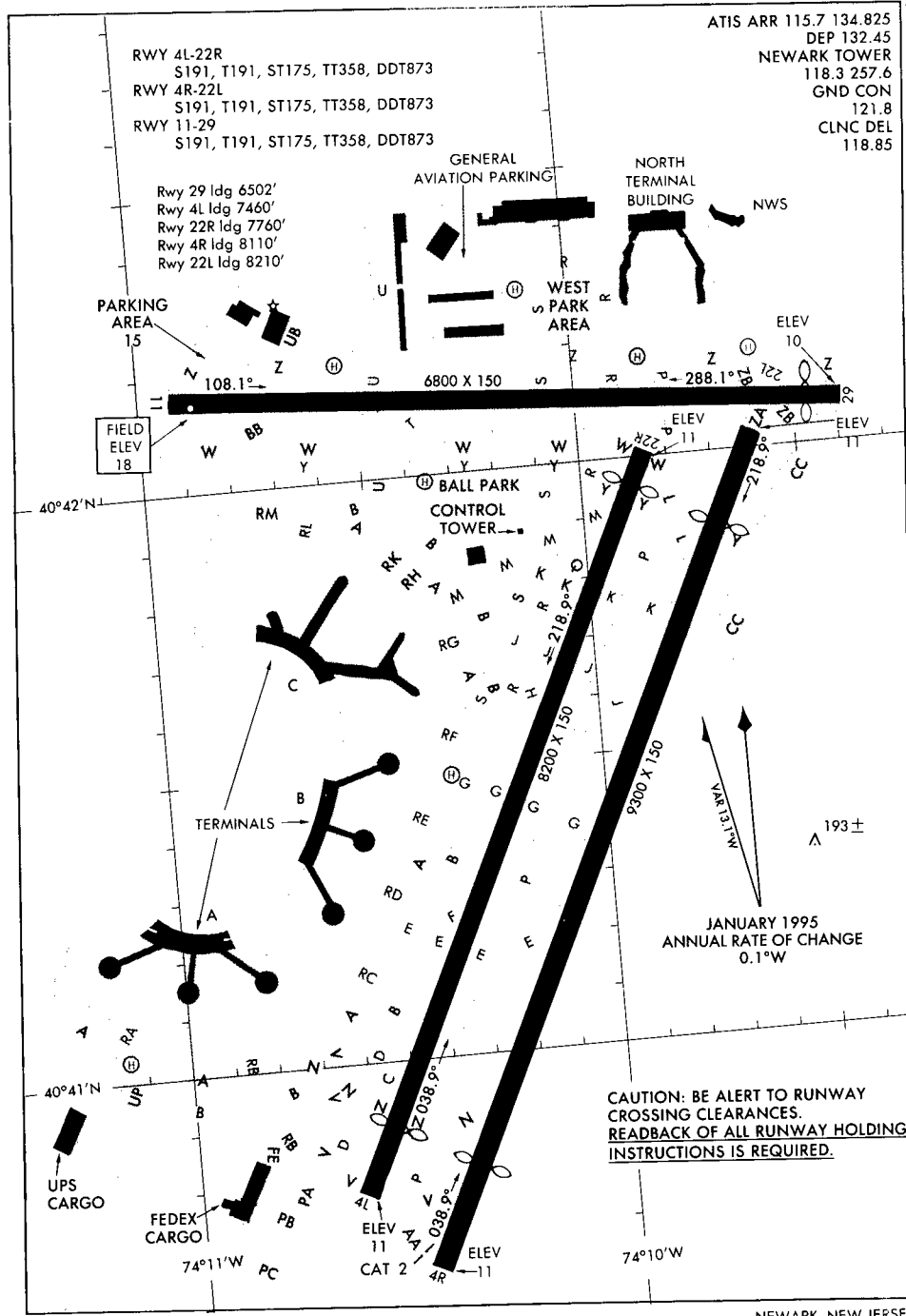
AIRPORT DIAGRAM 97030
