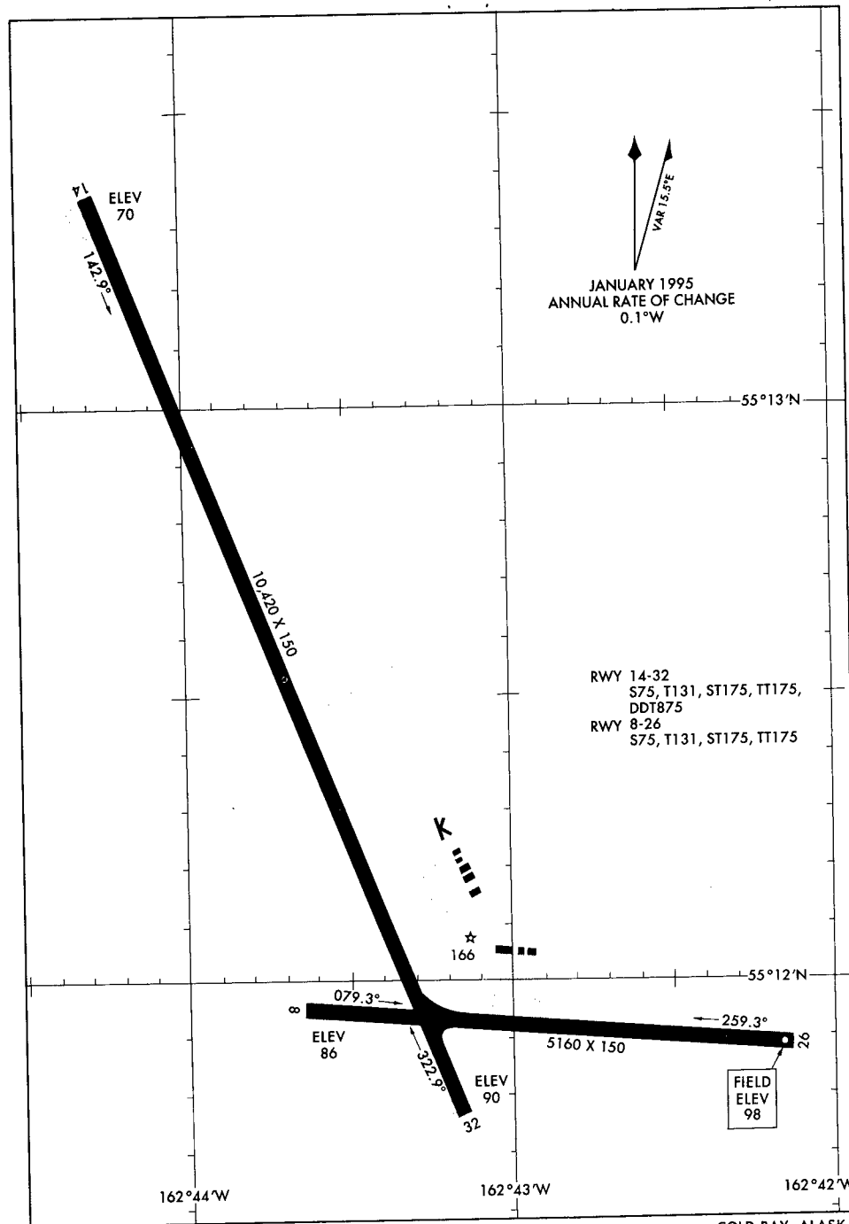
AIRPORT DIAGRAM 98057
