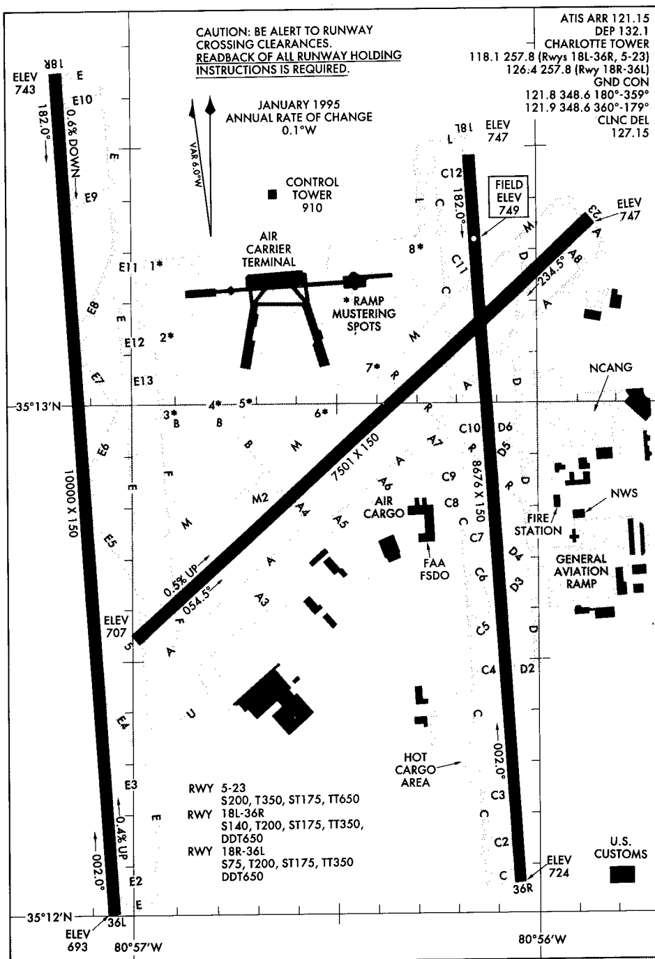
AIRPORT DIAGRAM 98169
