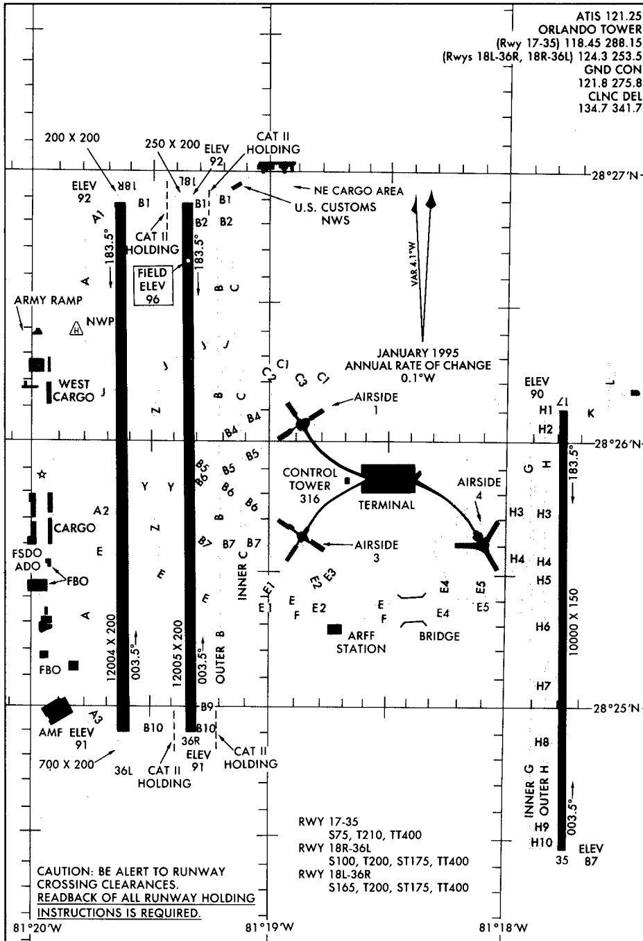
AIRPORT DIAGRAM 98113
