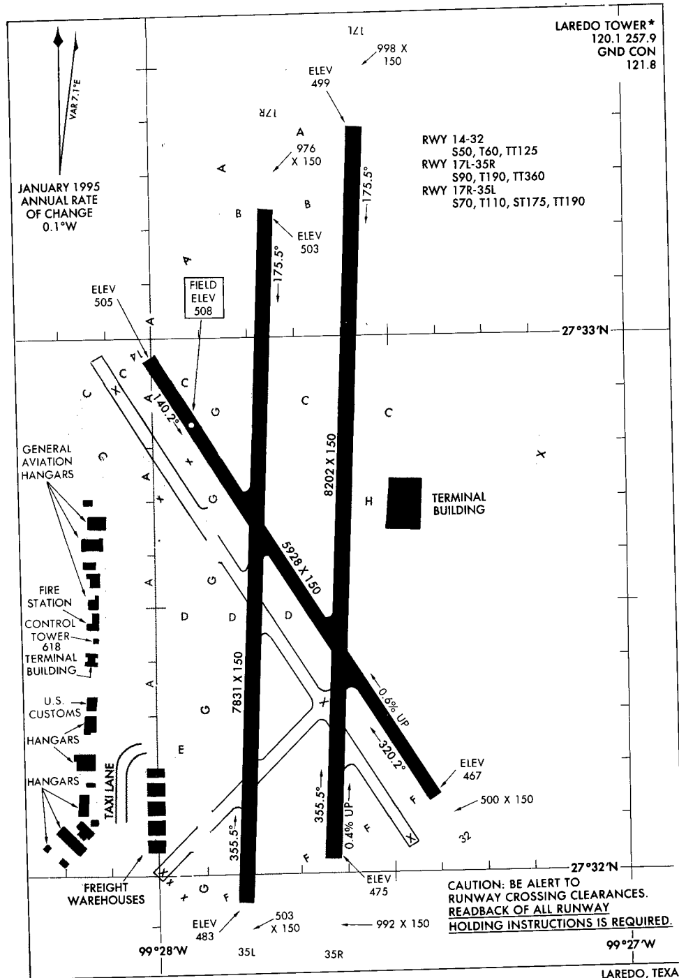
AIRPORT DIAGRAM 98113
