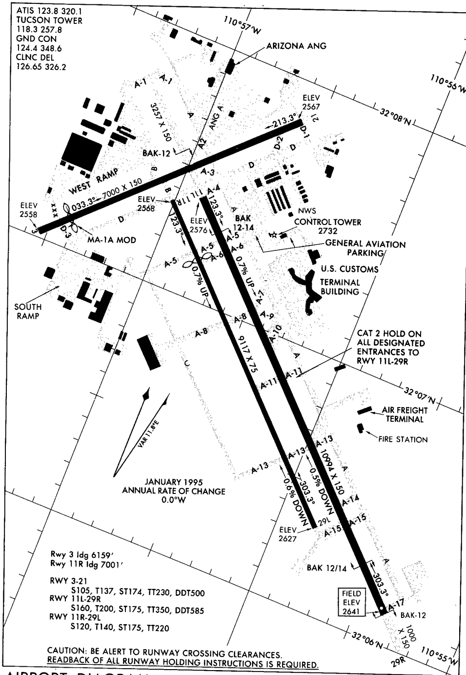
AIRPORT DIAGRAM
