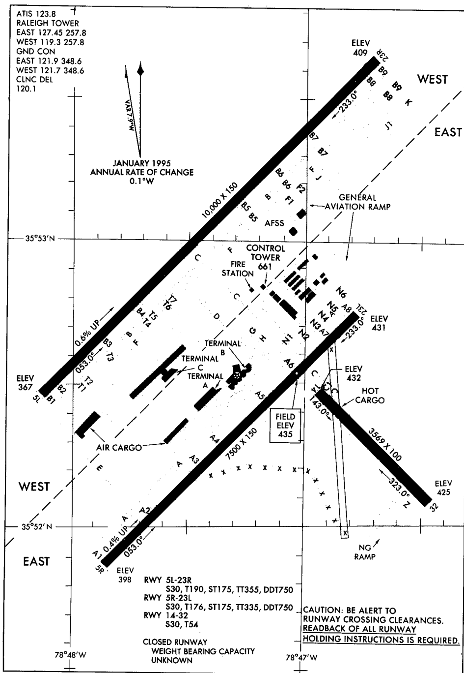
AIRPORT DIAGRAM 98225
