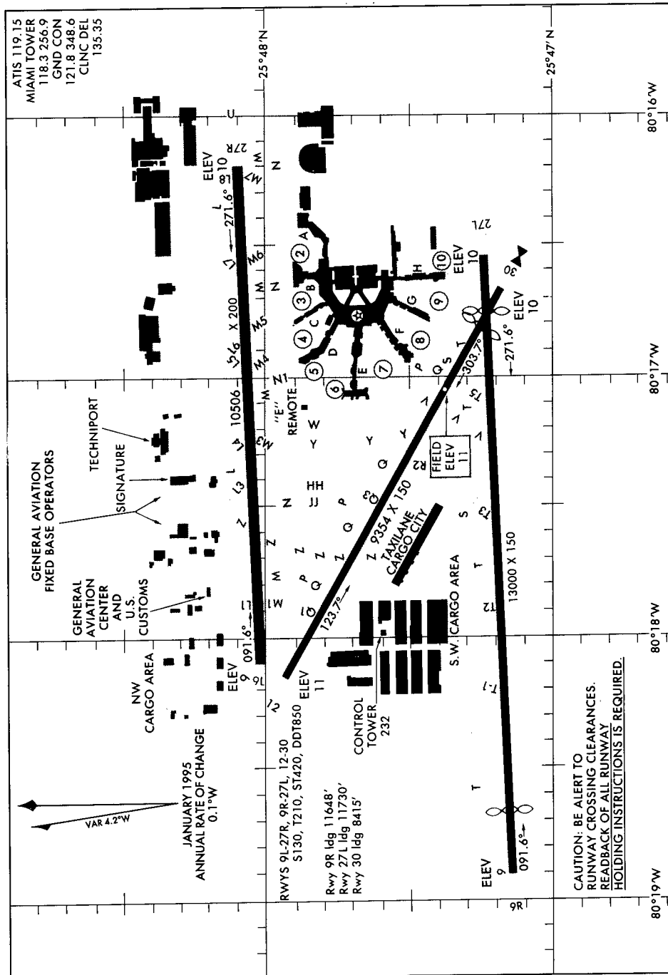
AIRPORT DIAGRAM 98225
