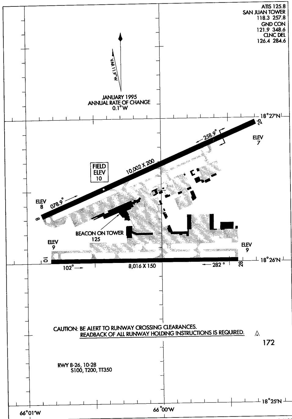
AIRPORT DIAGRAM 97254
