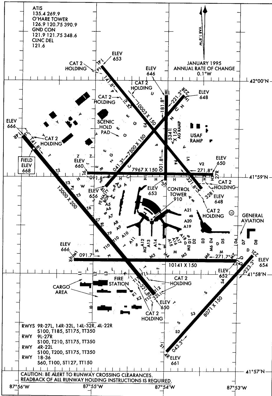
AIRPORT DIAGRAM 98113
