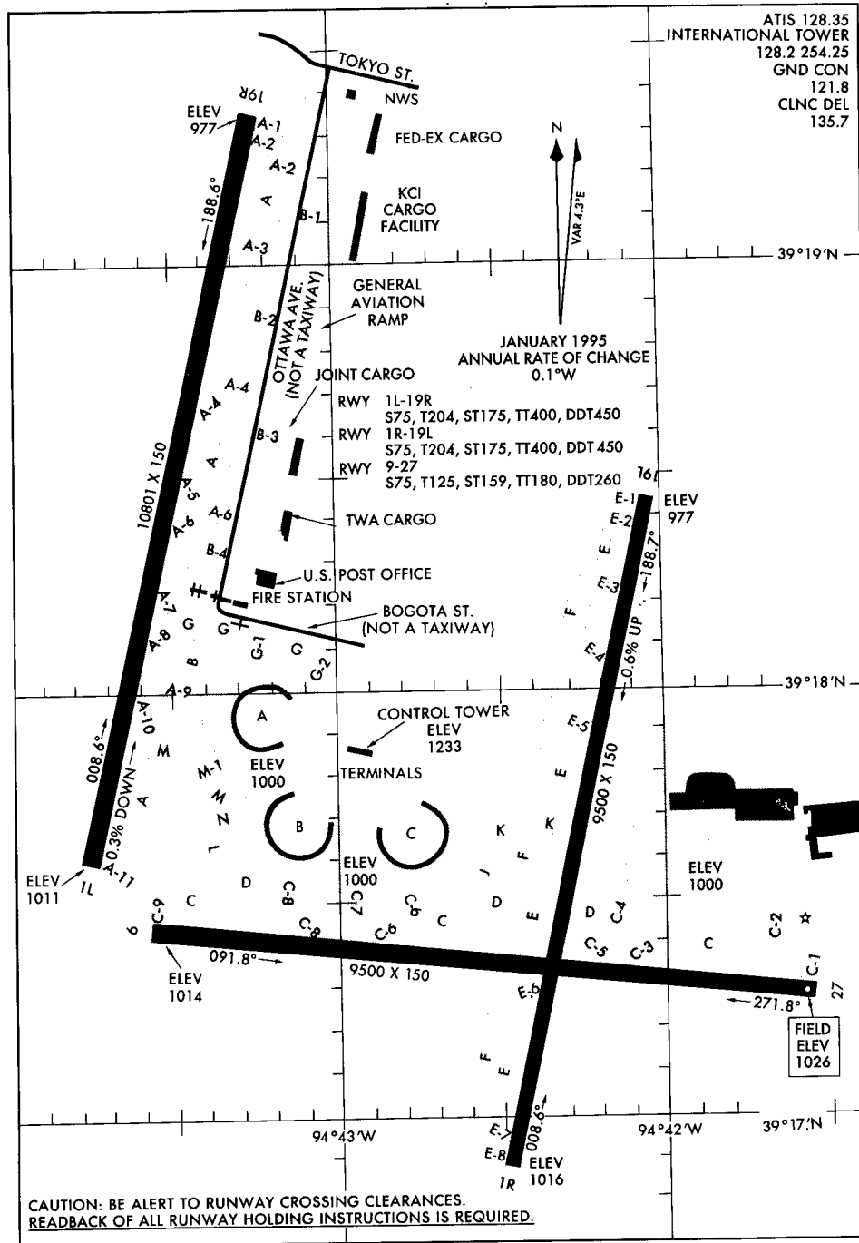
AIRPORT DIAGRAM 98225
