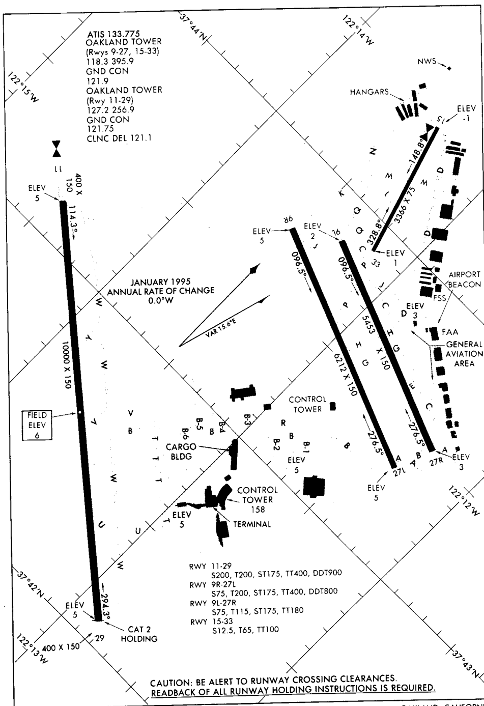
AIRPORT DIAGRAM 98057
