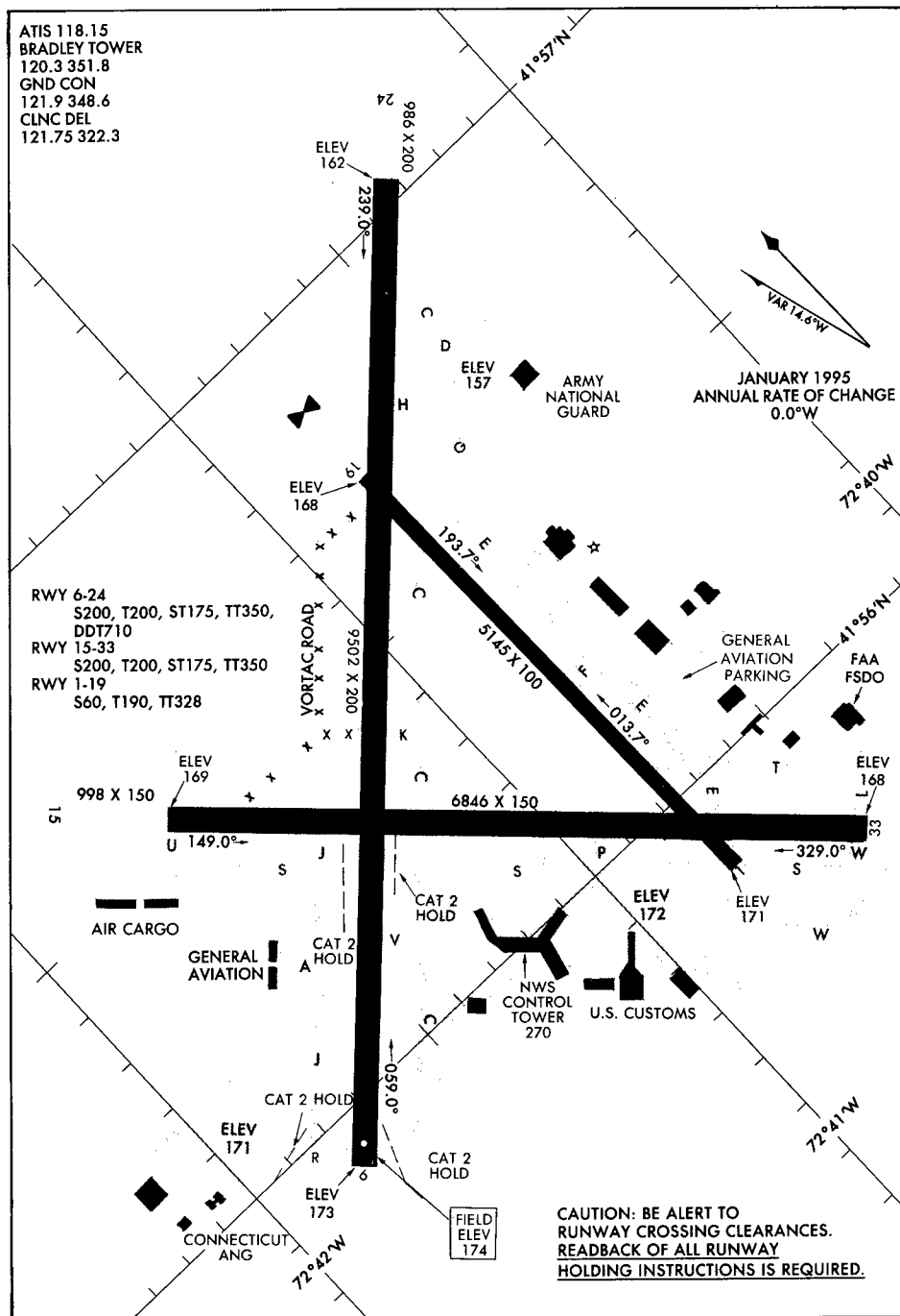
AIRPORT DIAGRAM 98281
