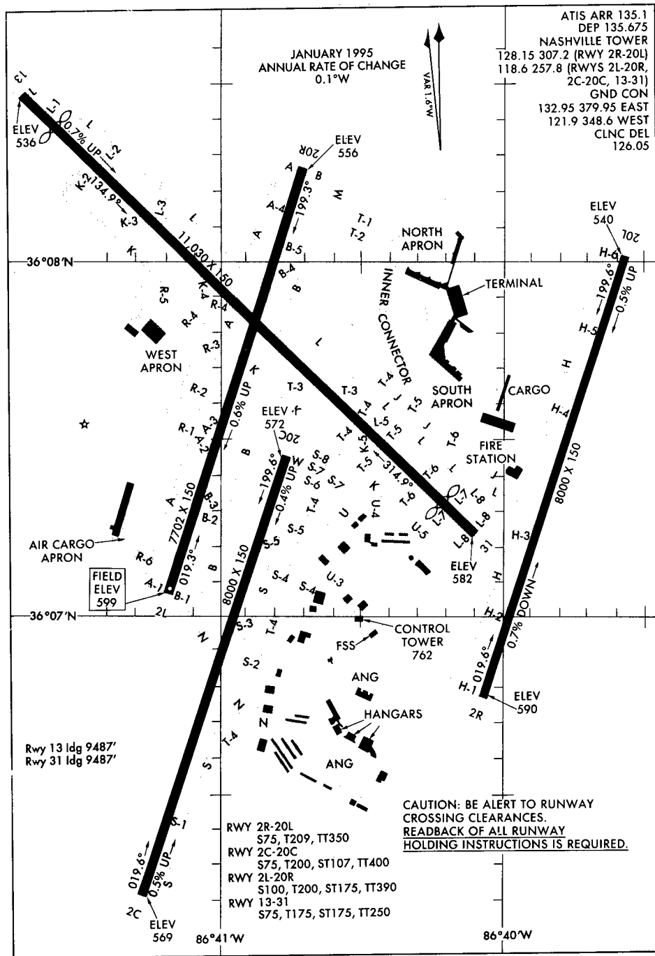
AIRPORT DIAGRAM 96340
