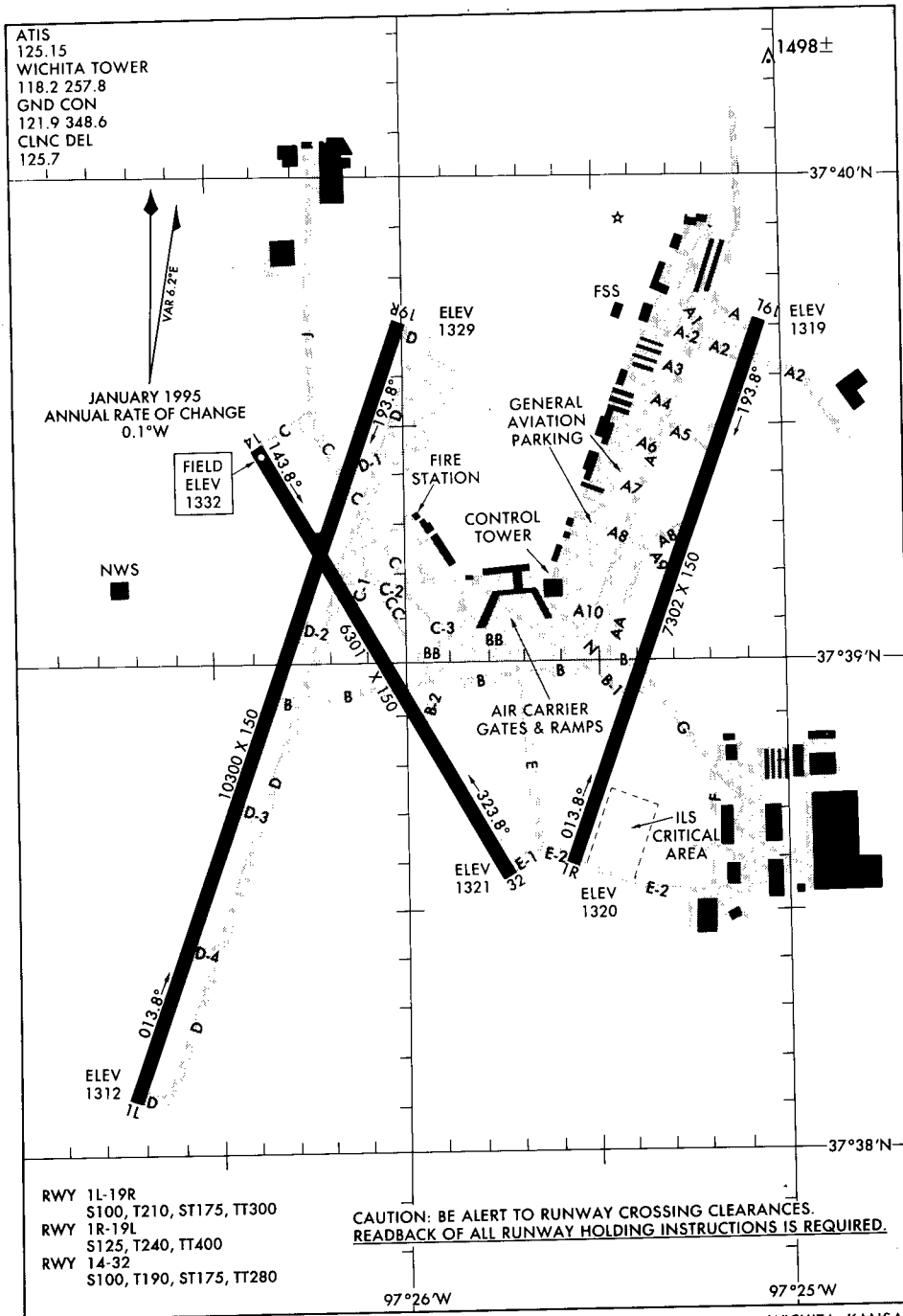
AIRPORT DIAGRAM 97254
