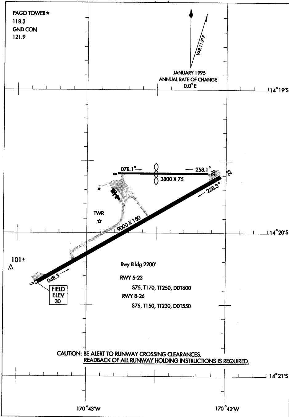
AIRPORT DIAGRAM 97254
