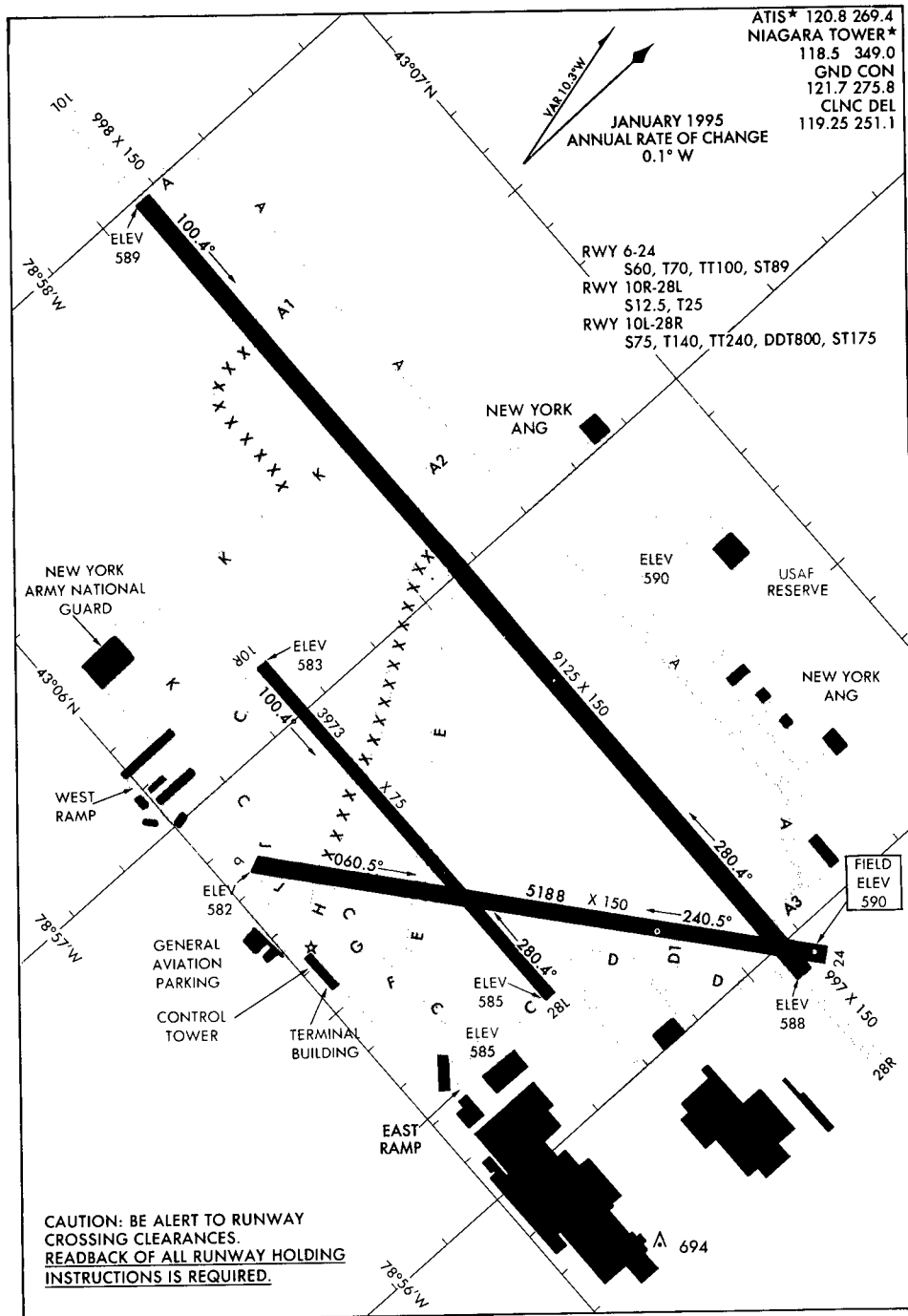
AIRPORT DIAGRAM
