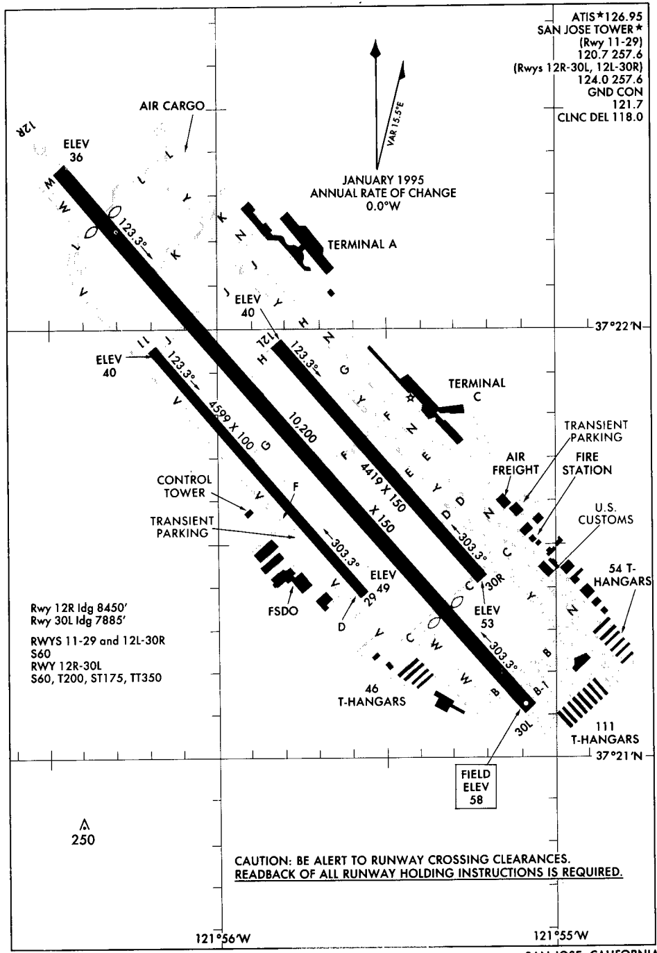
AIRPORT DIAGRAM
