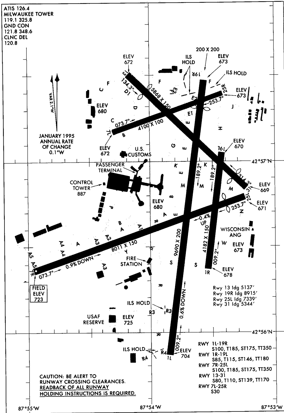
AIRPORT DIAGRAM 97030
