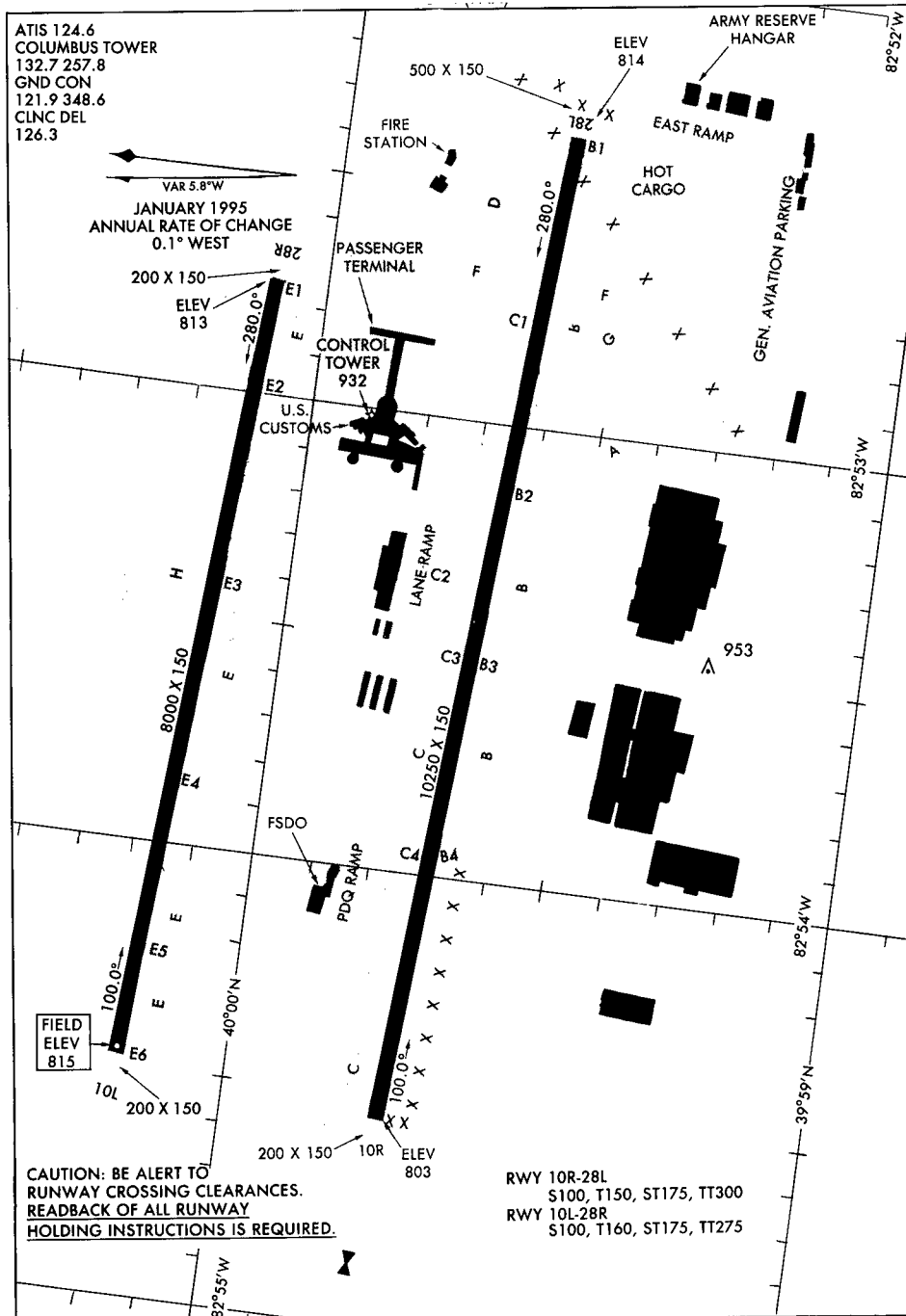
AIRPORT DIAGRAM 98281
