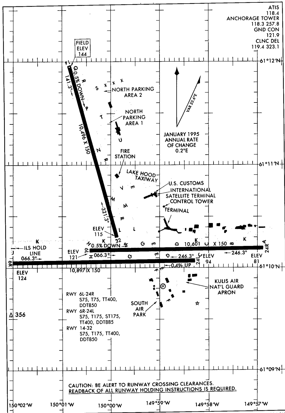
AIRPORT DIAGRAM
