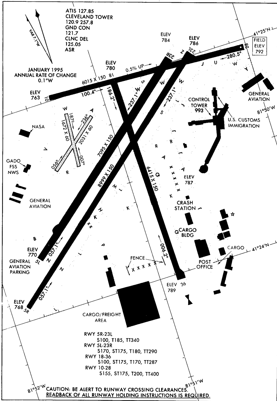
AIRPORT DIAGRAM 96340
