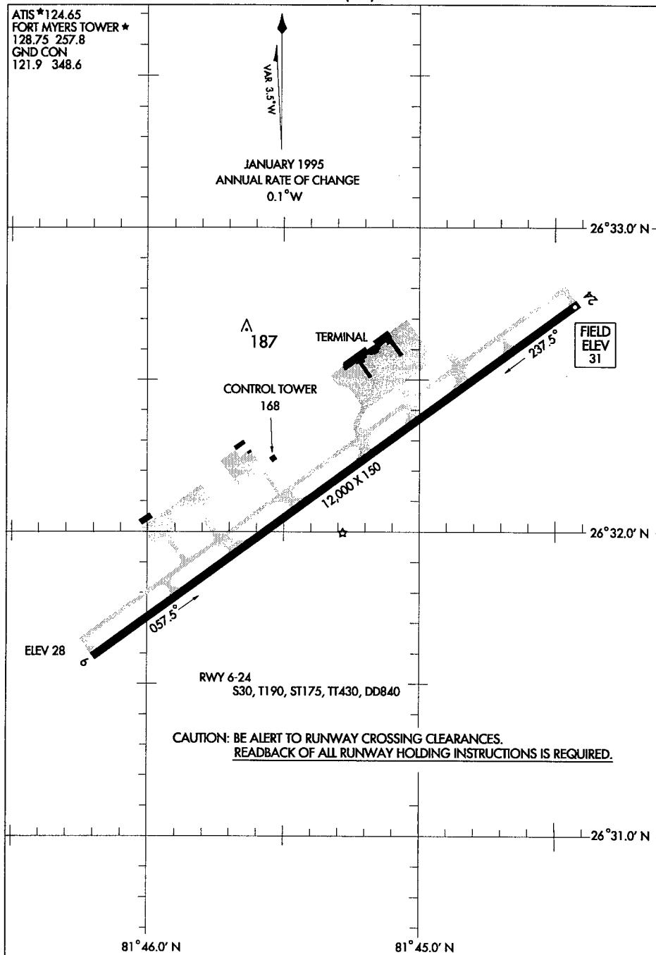
AIRPORT DIAGRAM 97254
