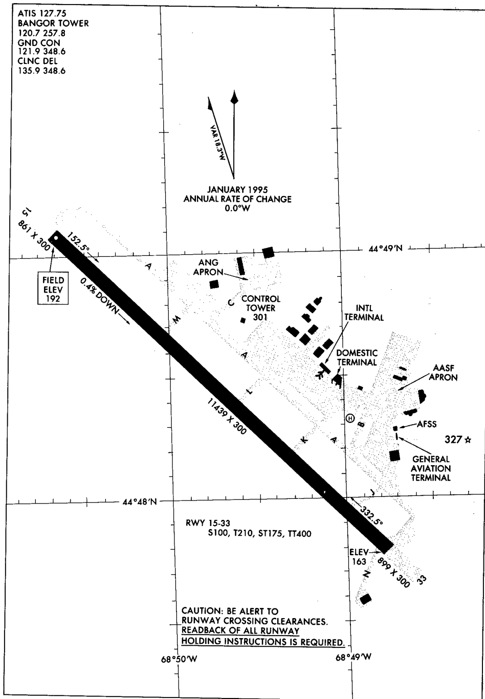
AIRPORT DIAGRAM
