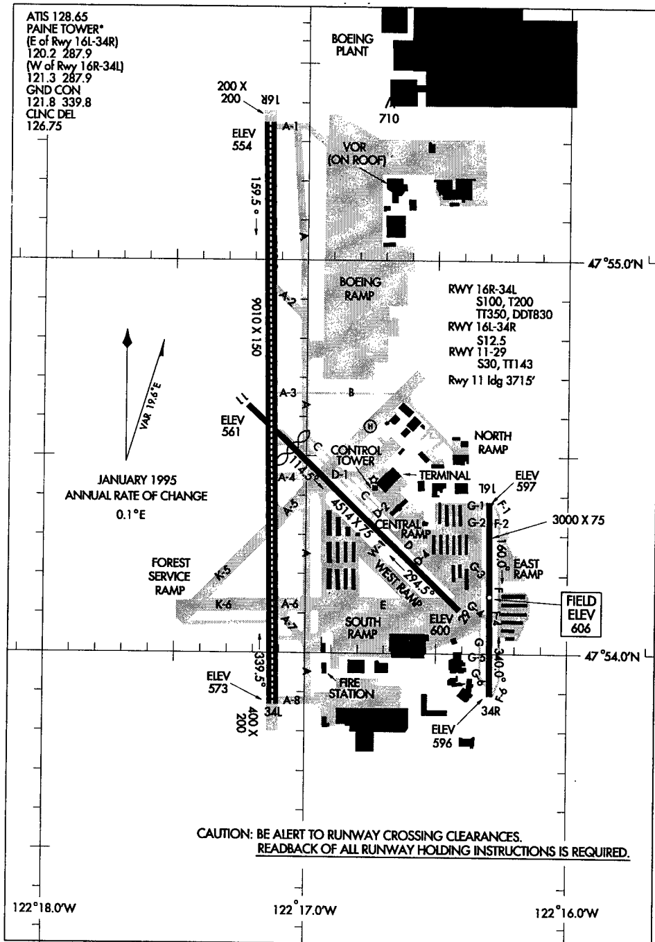
AIRPORT DIAGRAM 97254
