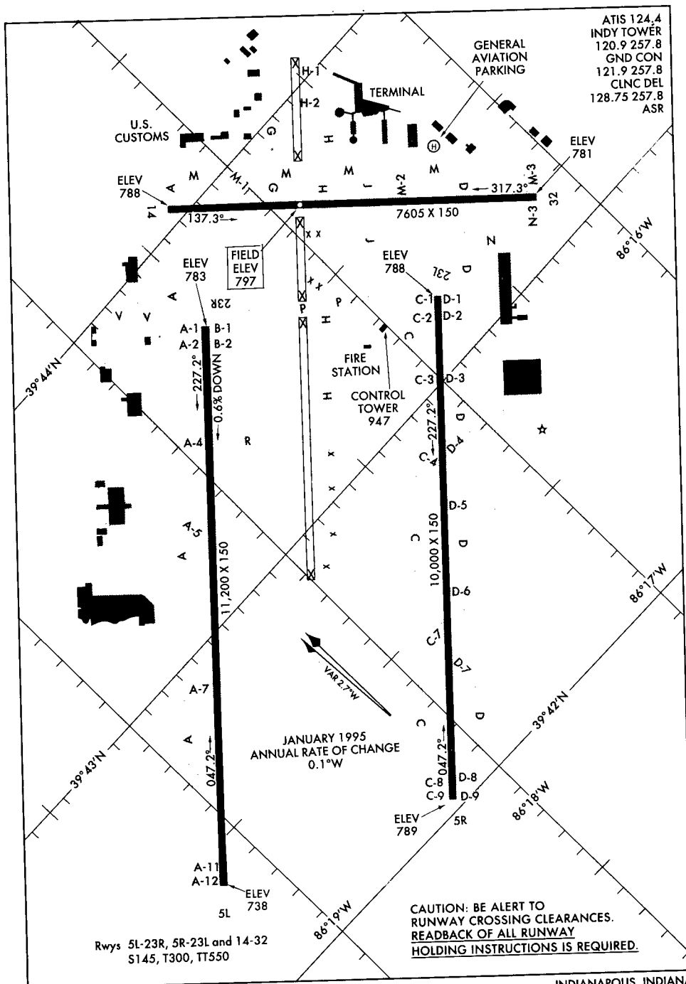
AIRPORT DIAGRAM 98169
