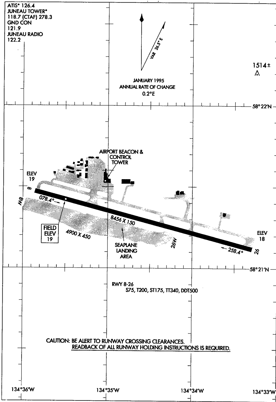
AIRPORT DIAGRAM
