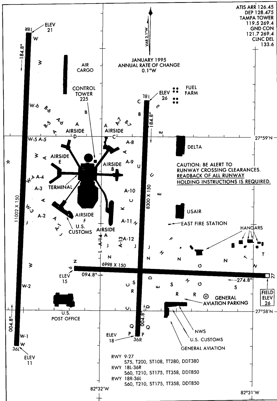
AIRPORT DIAGRAM 98281
