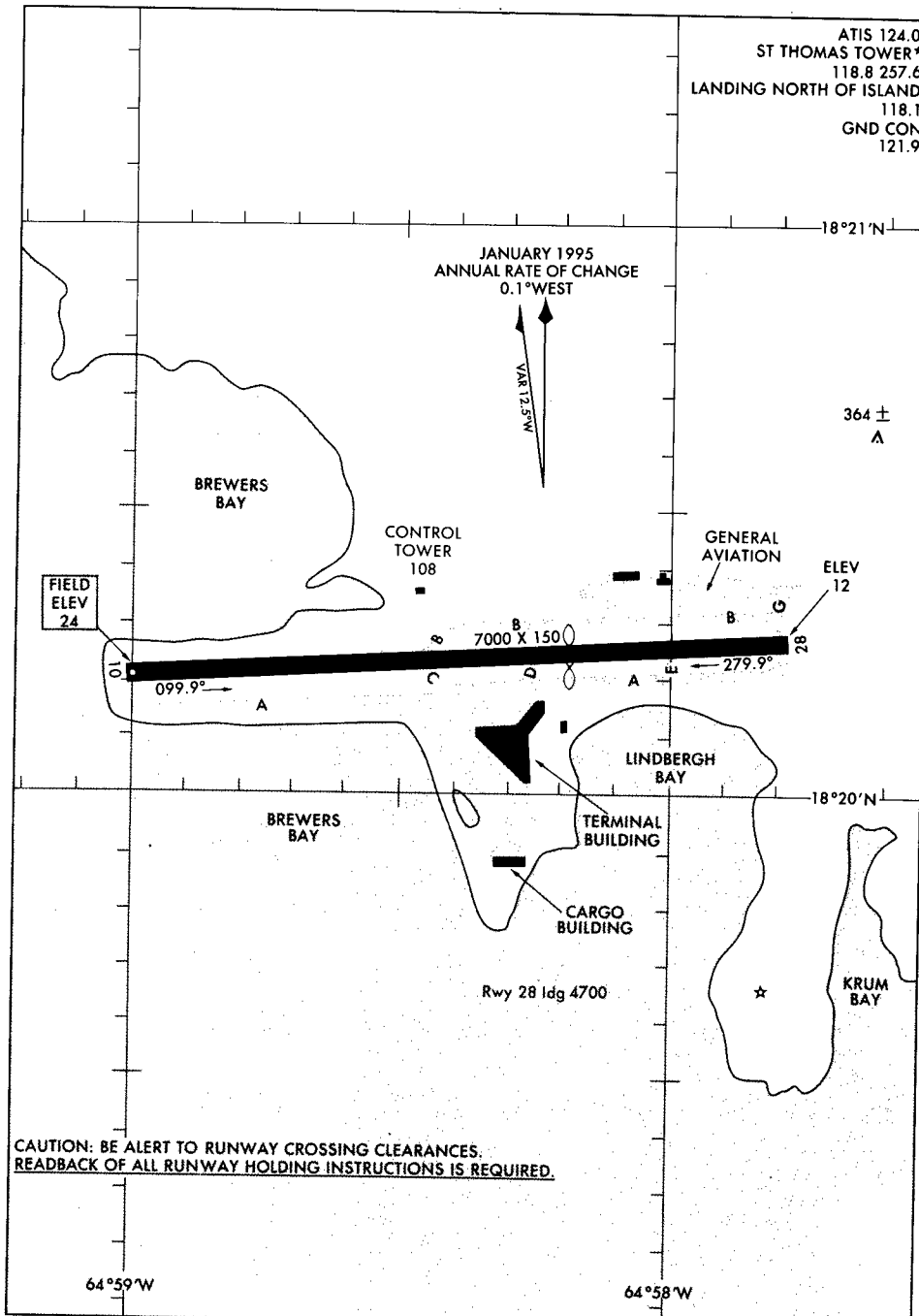
AIRPORT DIAGRAM 96340
