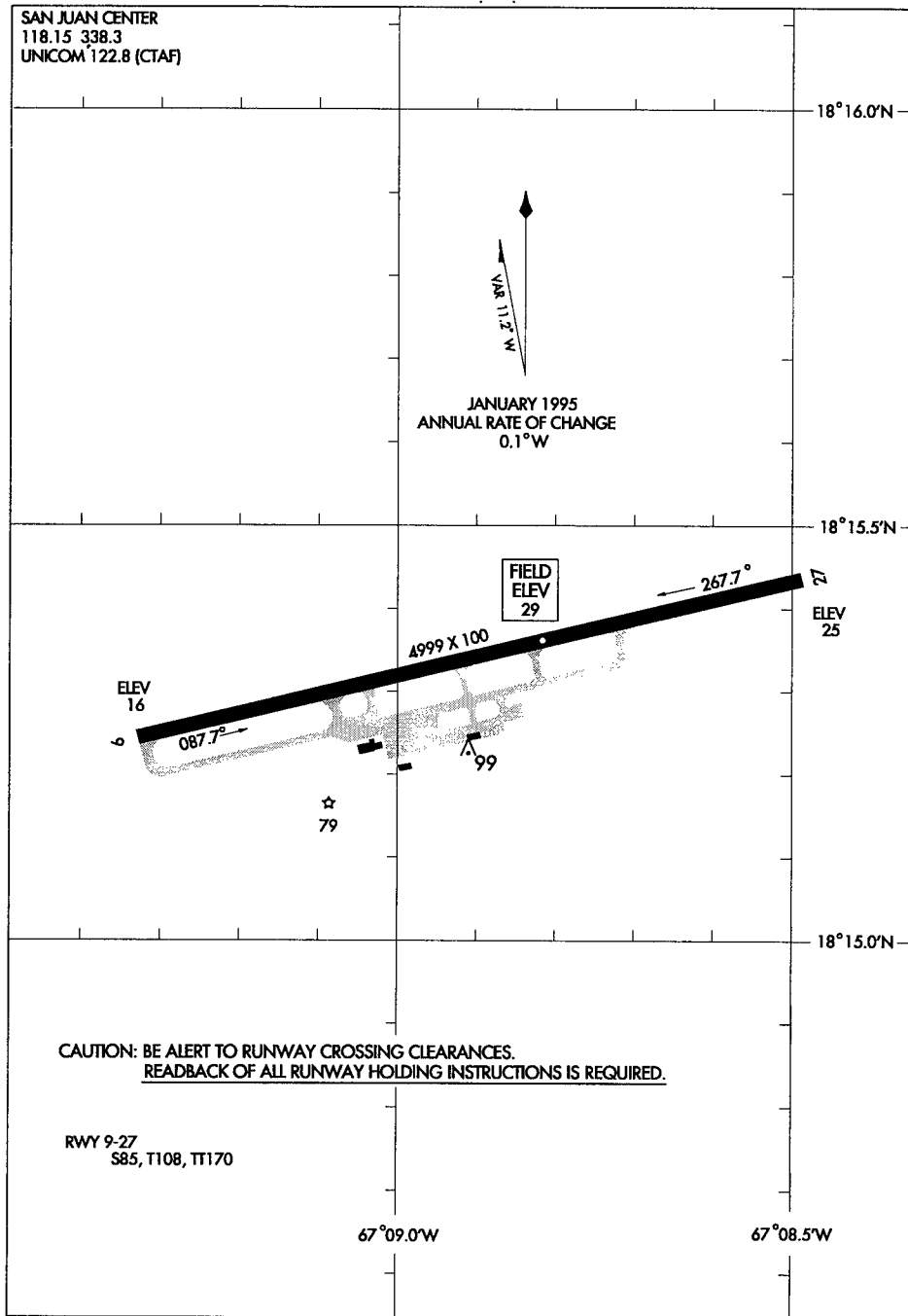
AIRPORT DIAGRAM 97254
