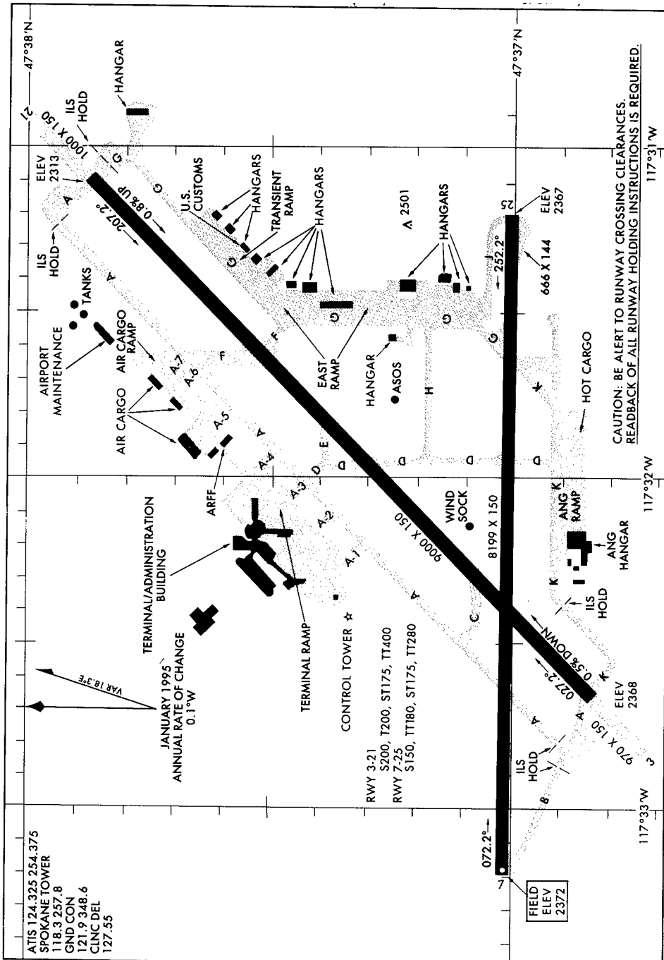
AIRPORT DIAGRAM 98113
