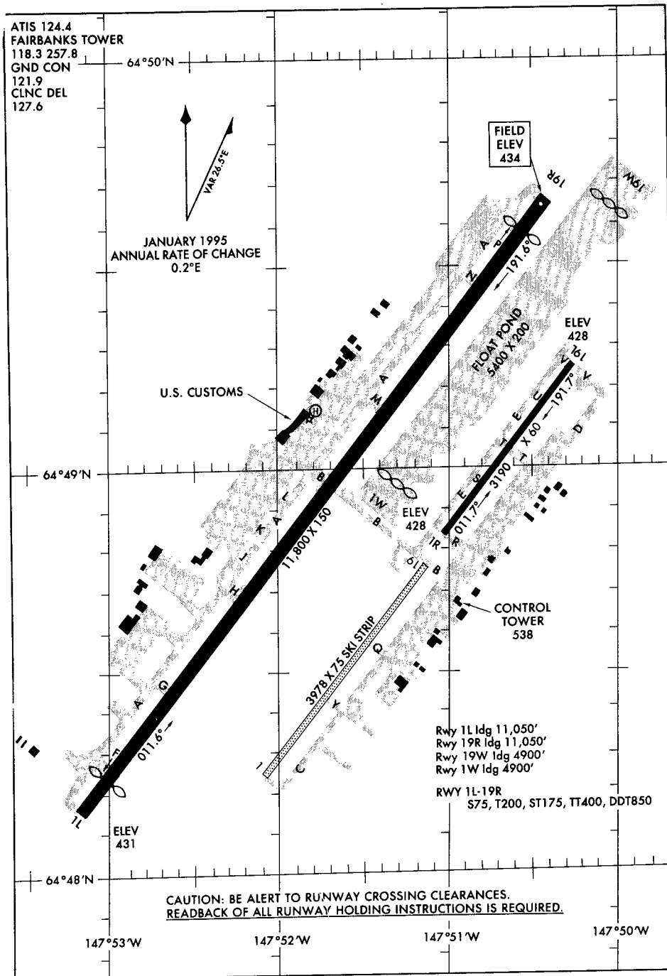
AIRPORT DIAGRAM
