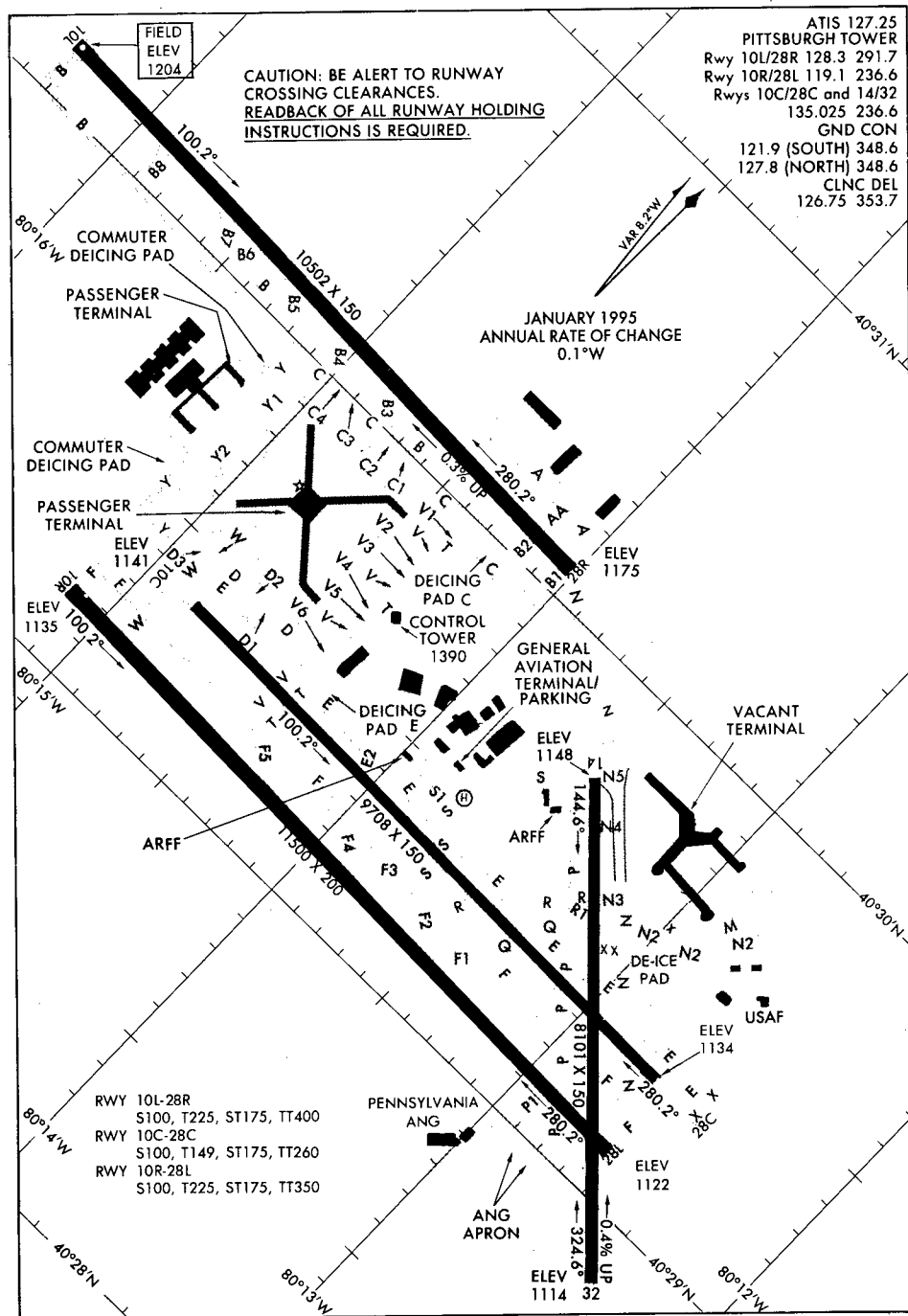
AIRPORT DIAGRAM 98169
