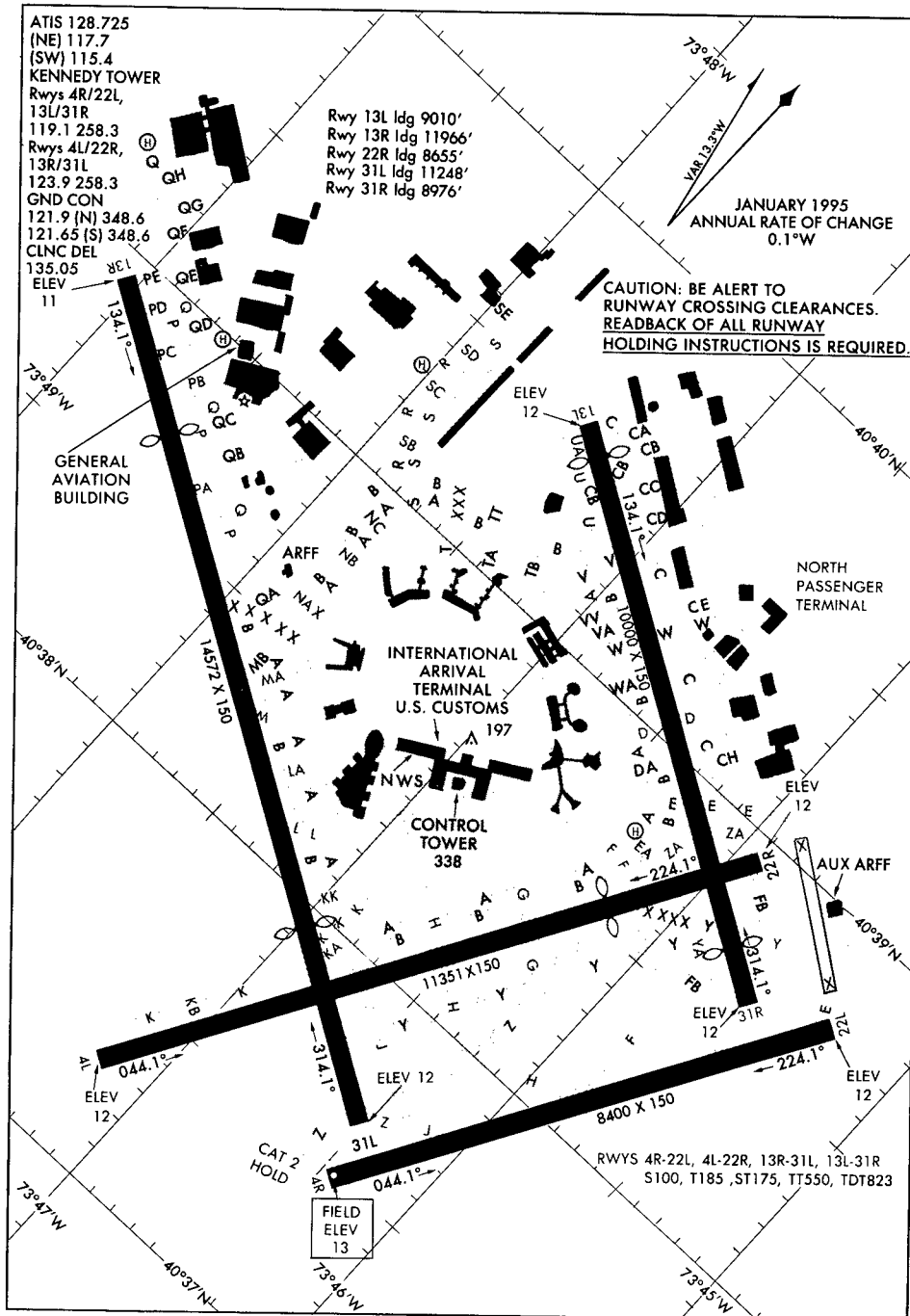
AIRPORT DIAGRAM 98281
