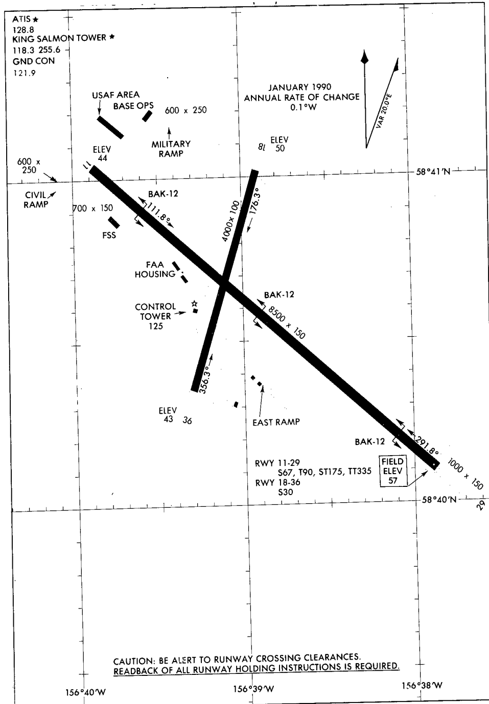
AIRPORT DIAGRAM
