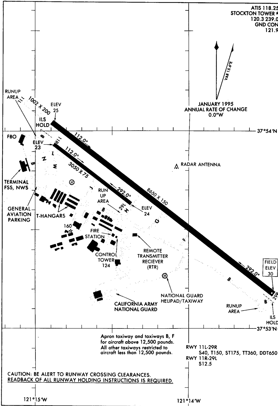
AIRPORT DIAGRAM 97030
