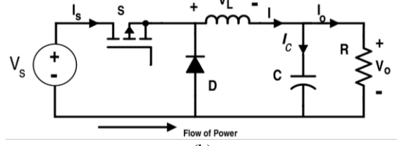
Figure 6. (a) Boost and (b) Buck converter circuit design using the GaN and SiC switches
