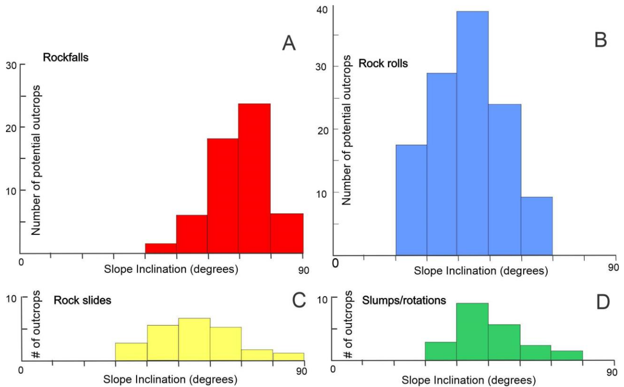
Figure 21. Embankment steepness and its relationship to slope failure type.
