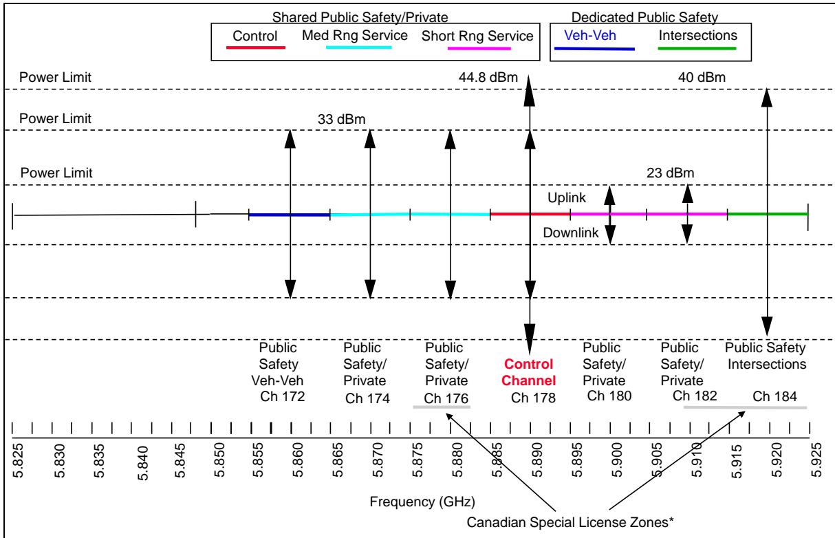
Figure 1-1: DSRC Channel Plan in the ITS Band 13 14
