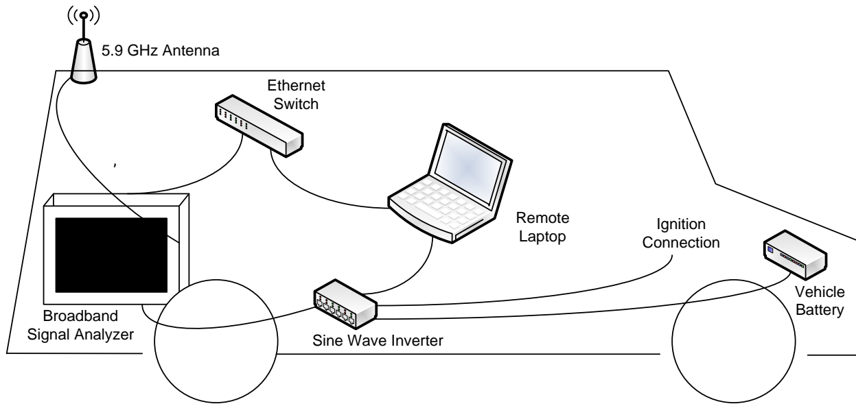
Figure 4-11: RF Signal Measurement Mobile Configuration
