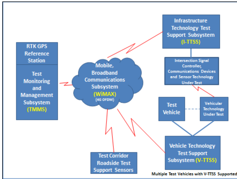
Figure 4-3: Simplified Overview of CVHT System
