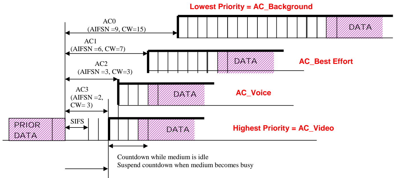
Figure B-2: Depiction of 802.11 default EDCA parameters
