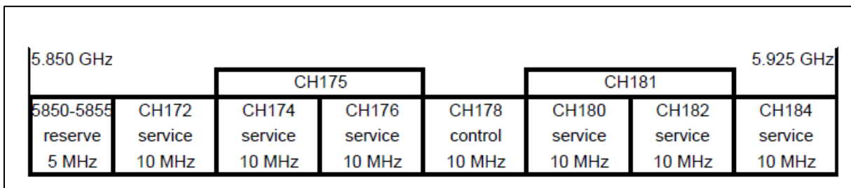
Figure 1-2: DSRC channel number designations for both 10 and 20MHz channels 15
