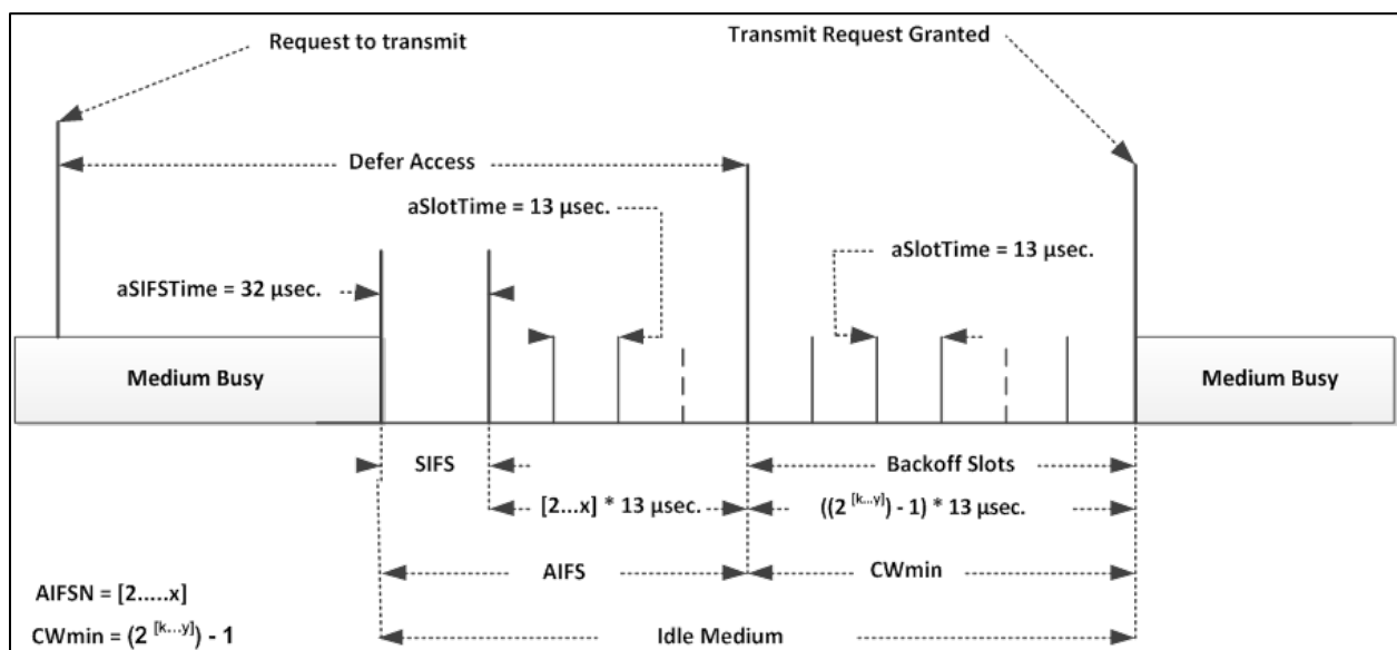
Figure B-1. Breakdown of Interframe Spacing
