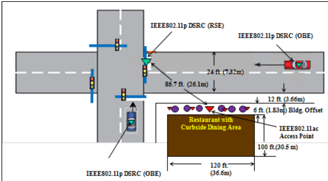
Figure 6-1: Depiction of Scenario 1 (Outdoor Access Point near intersection)
