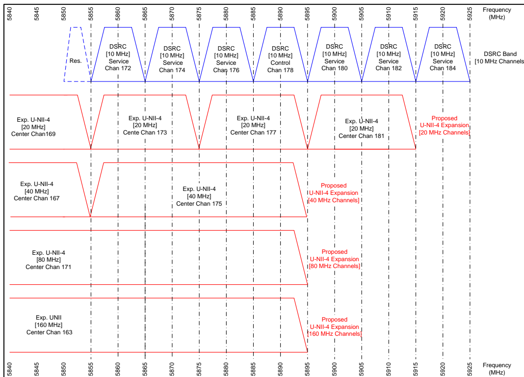
Figure 1-4: U-NII-4 overlap with the DSRC band 18
