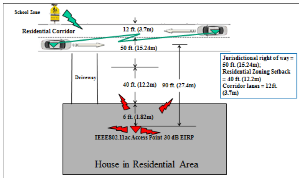
Figure 6-2: Depiction of Scenario 2 (Indoor Access Point by a residential street)
