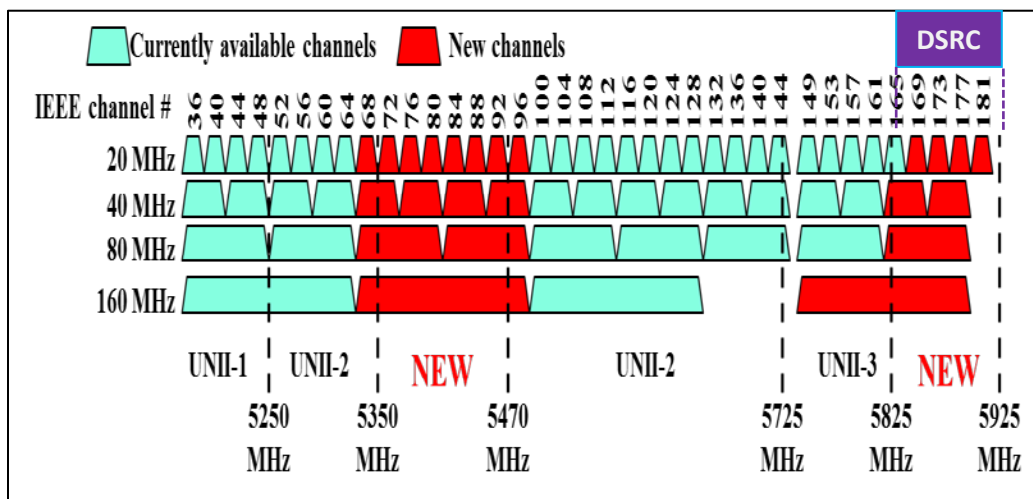
Figure 1-3: Proposed new U-NII-4 band
