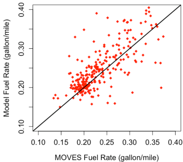
Figure 17. Model Prediction vs. MOVES Output for Fuel Consumption Rate in City of Eichstätt
