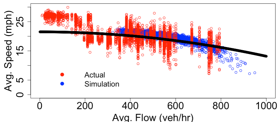
Figure 7. Comparison between the simulation results and real-world observations of detailed traffic patterns
