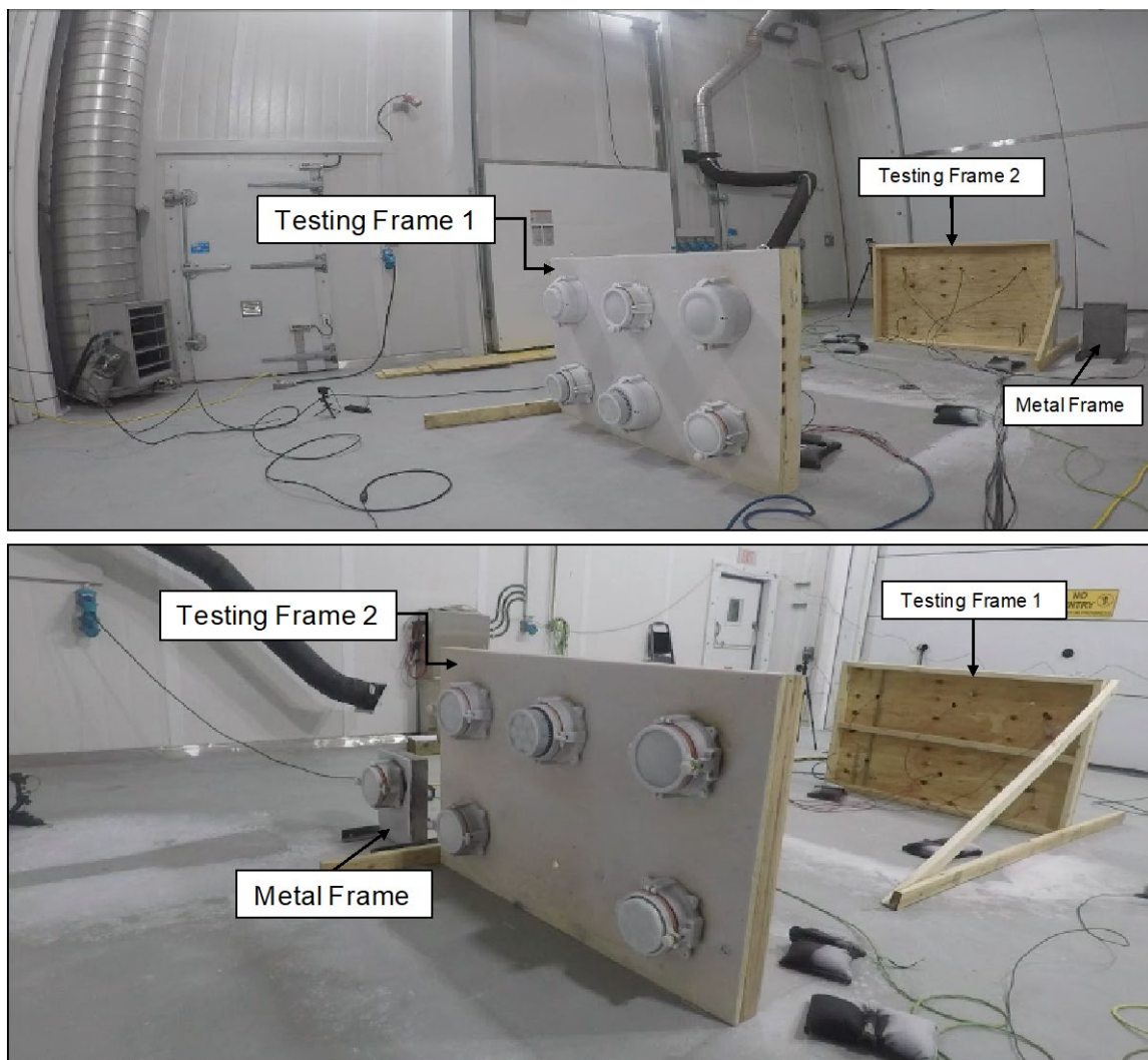
Figure 7. Setup of test frames in the SCC
