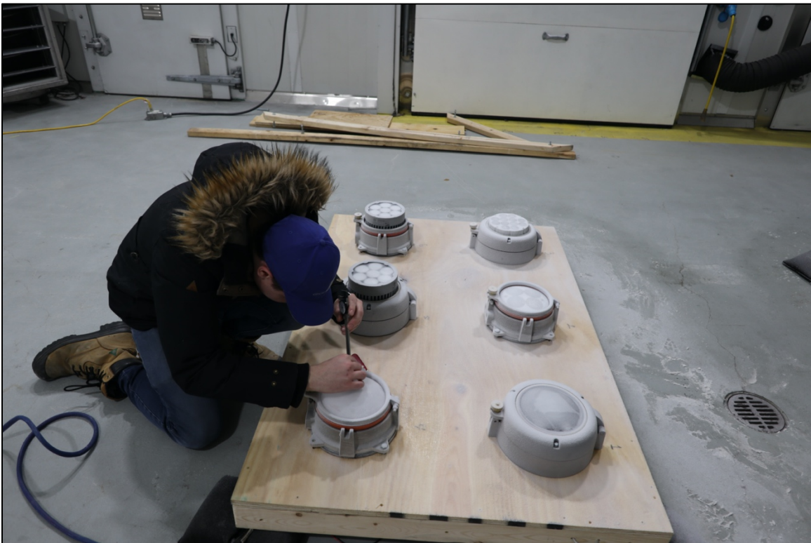
Figure 55. Experimenter measuring the ice layer thickness using a depth gauge
