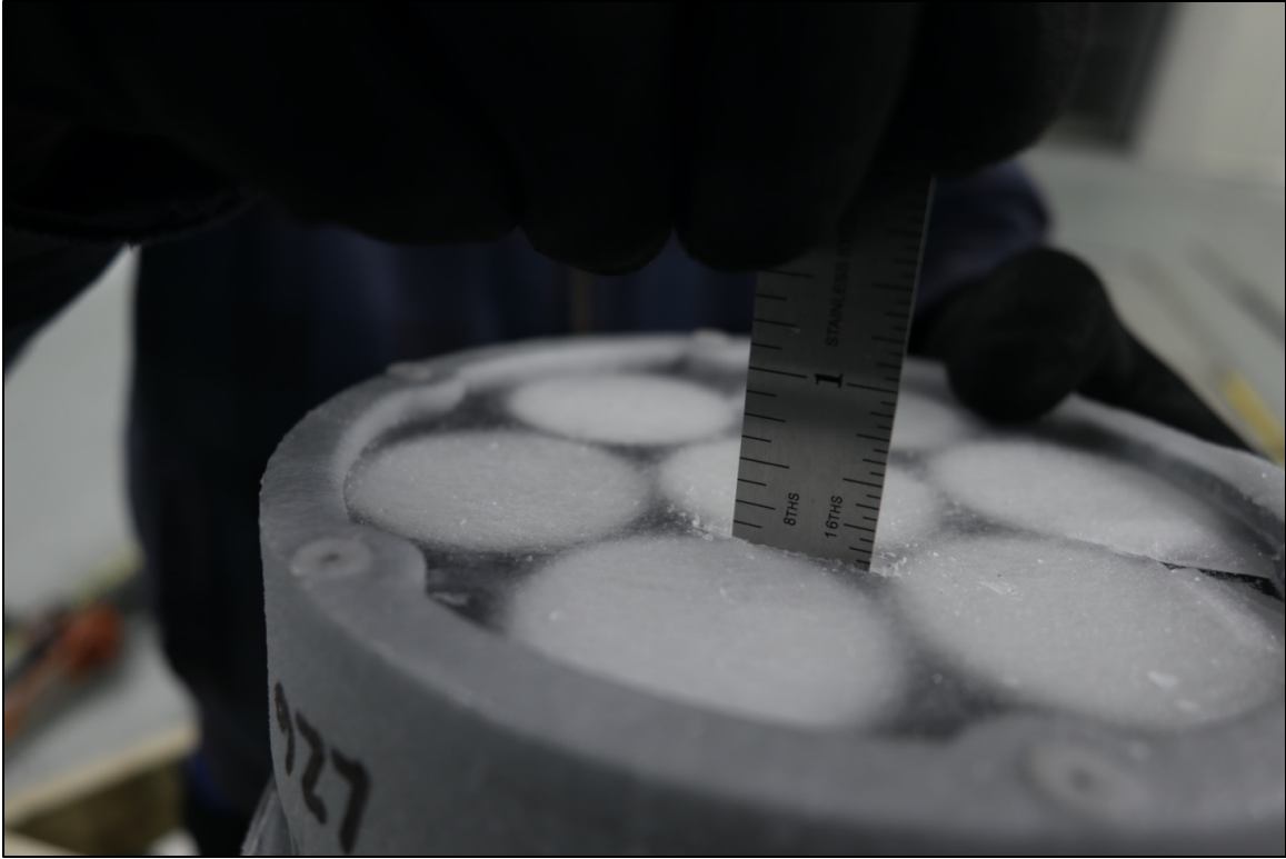
Figure 50. Measurement of ice thickness on LED sample after Trial 3
