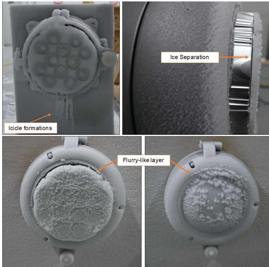
Figure 9. Light fixtures after Trial 3 and 30 minutes of operation
