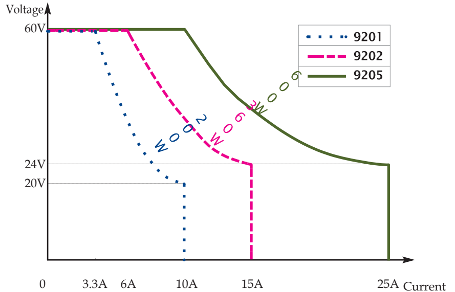
Models 9201 / 9202 / 9205 output characteristics
