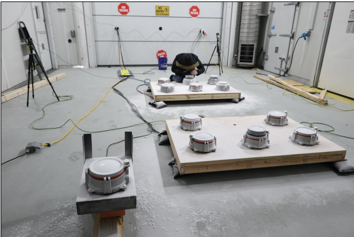
Figure 57. Test frames in the late stages of building the 1/4-inch layer of ice
