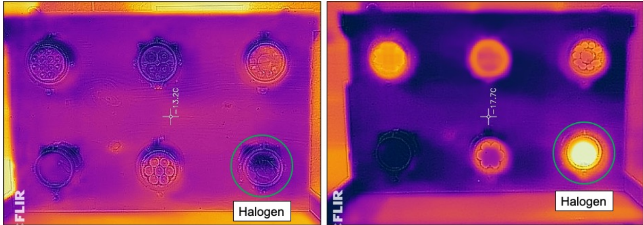
Figure 2. Thermal image of preliminary temperature testing
