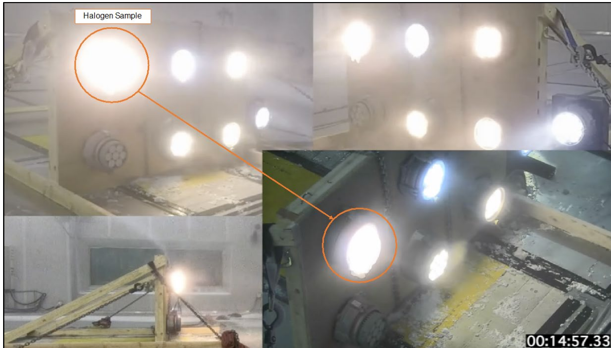
Figure 17. Photograph taken during Trial 2 showing ice accumulation on the halogen lamp
