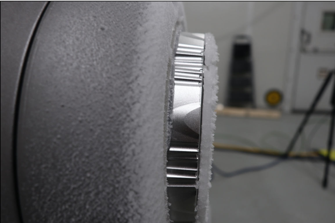
Figure 32. Separation of ice from lens of LED sample
