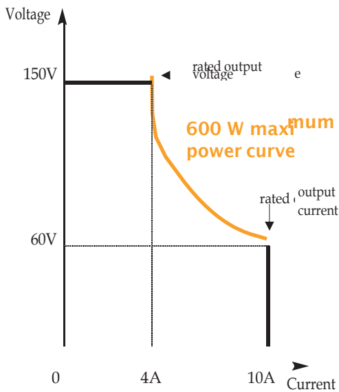
Model 9206 output characteristics
