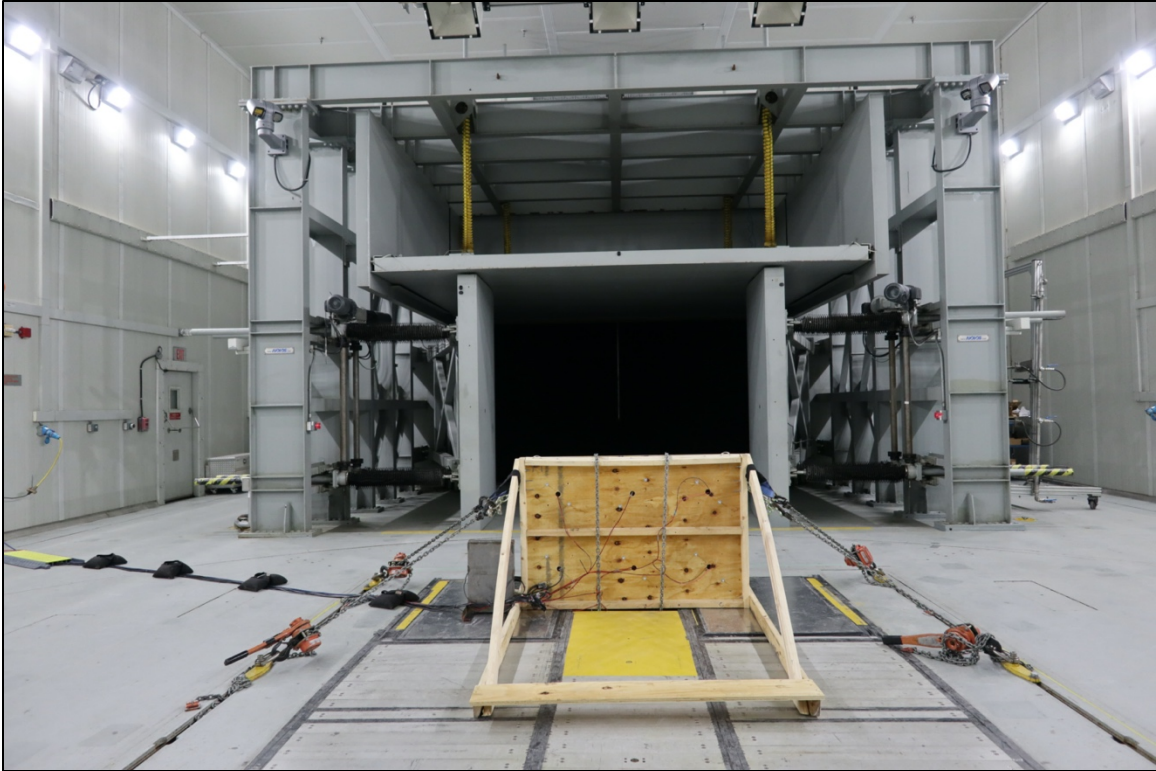
Figure 58. View of the testing area in the CWT
