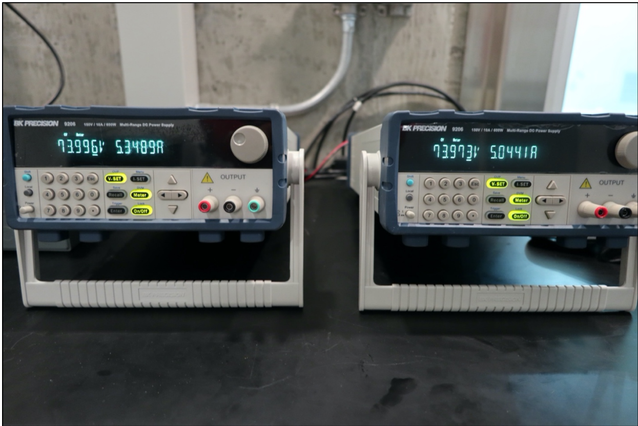
Figure 51. Power supplies used during Snow Accumulation Test
