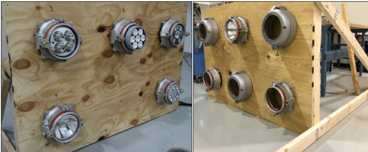
Figure 1. Test frames with light fixtures mounted
