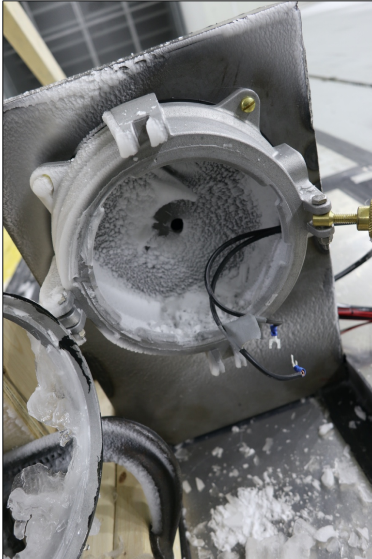
Figure 60. Documentation of snow inside the housing of the metal test frame
