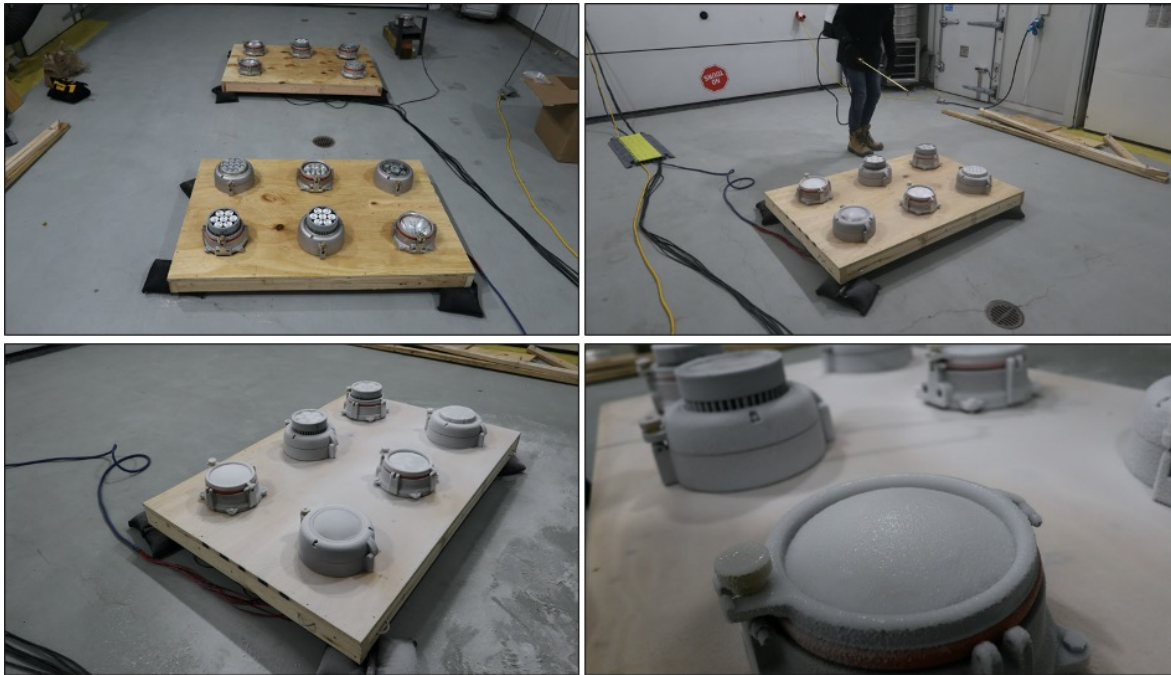
Figure 4. Setup of light fixtures in the SCC for ice layering
