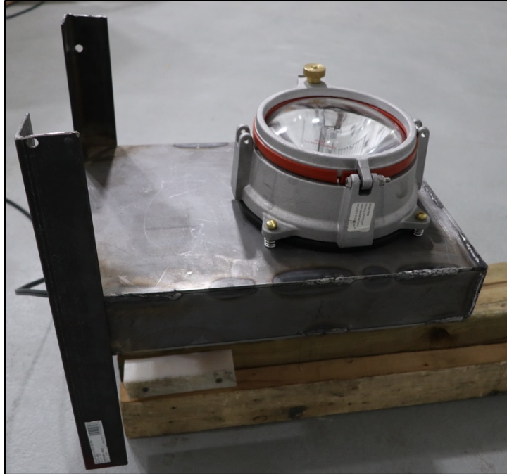
Figure 3. Metal test frame with housing and halogen lamp mounted
