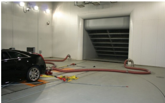
Dual closed-pipe vehicle exhaust extraction system
