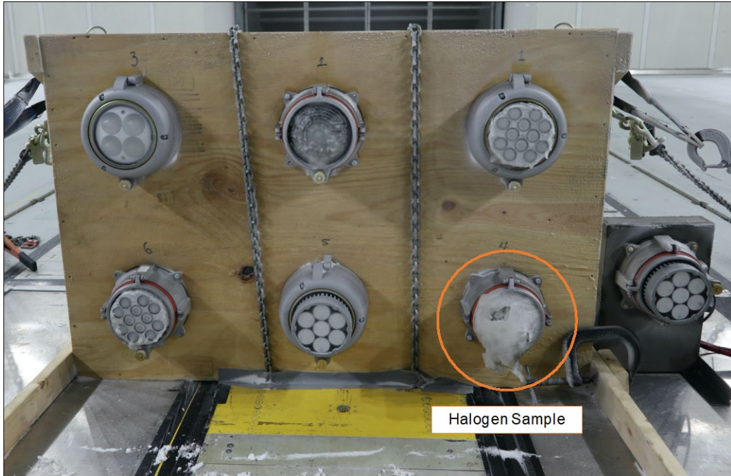
Figure 14. Accumulation of snow and ice on light fixtures after Trial 1
