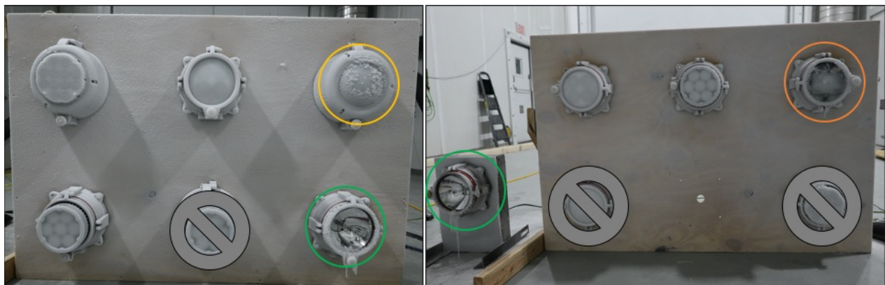
Figure 8. Extent of ice melting at the conclusion of Trial 2
