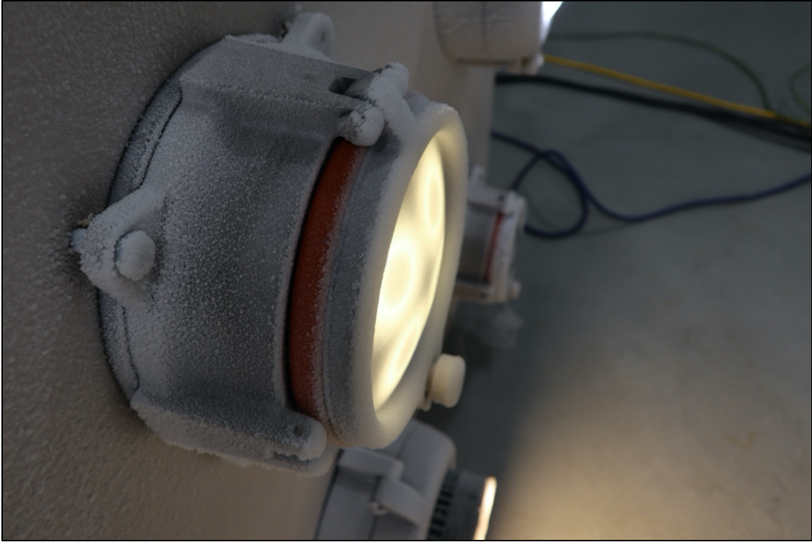
Figure 27. LED sample during testing
