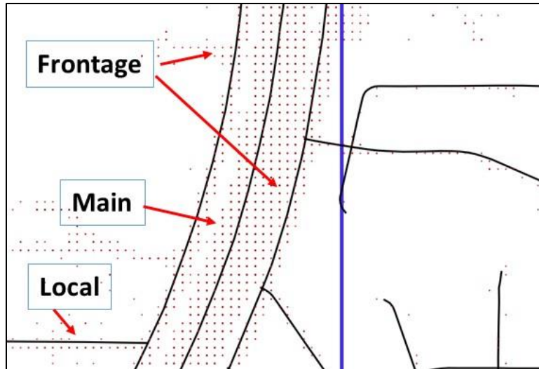
Figure 9. Matching GPS Data to Road Segments.
