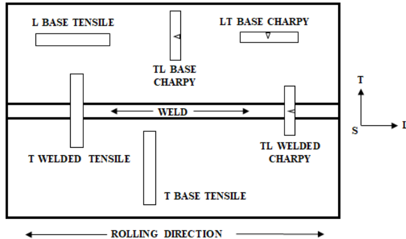
Figure 1. Schematic illustration of sample orientations with reference to a coordinate system defined by the L (longitudinal/rolling), and T (long transverse), and S (short-transverse) directions (the schematic is an indication of the types of samples used in Group 1 and 2, not the actual cut plan)
