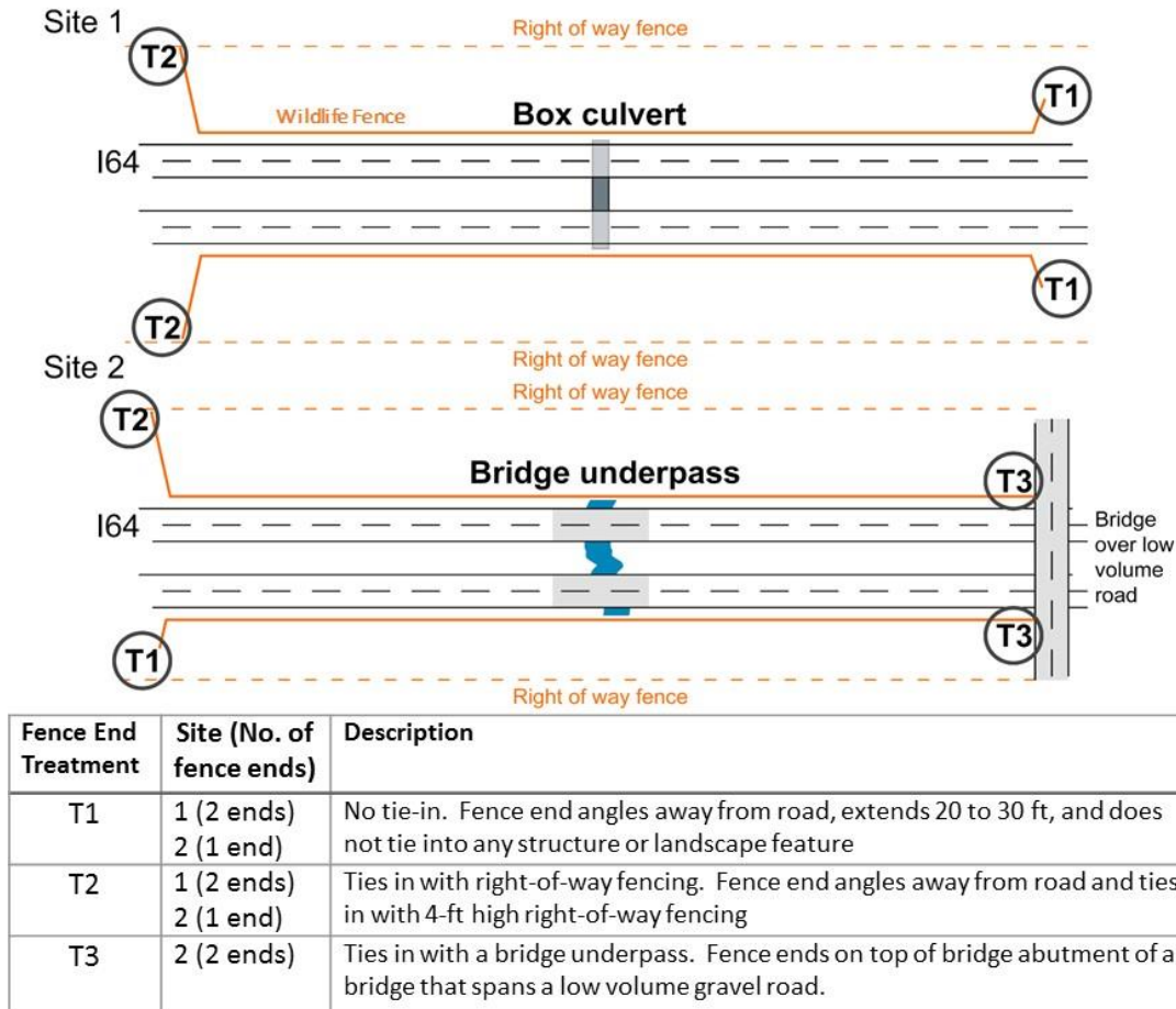
Figure 4. Fence End Treatments at the Two Study Sites
